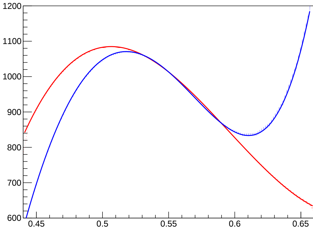
pol3 and pol9 fits
