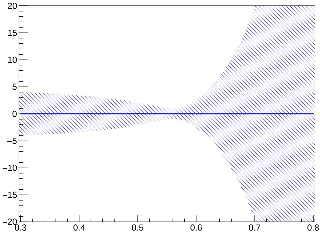
confidence band of pol9 fit
