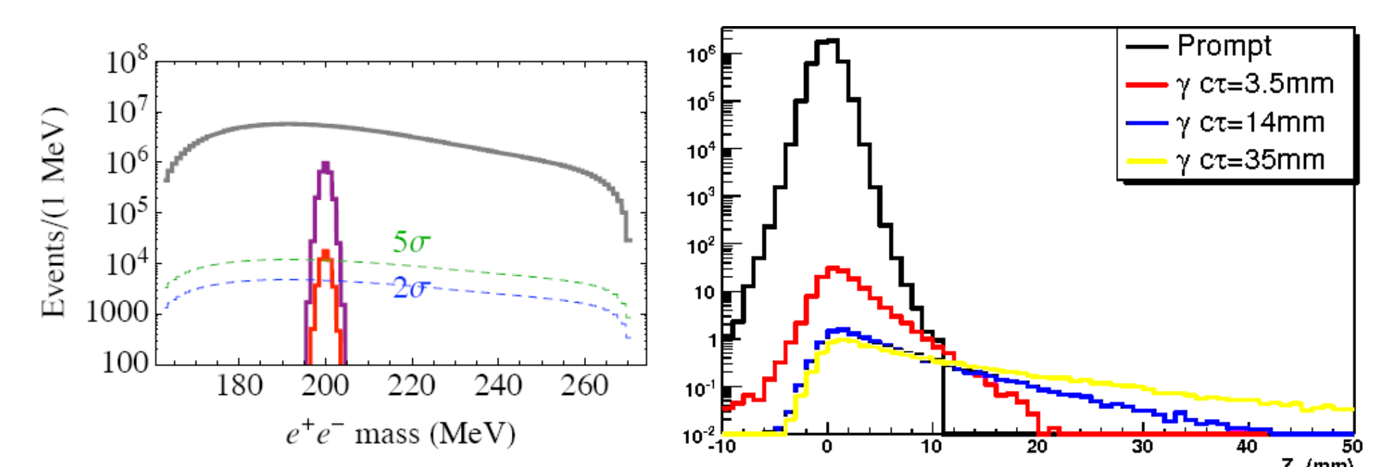
Figure 8: Example signals and backgrounds for (left) a resonance search and (right) a vertexing search.
