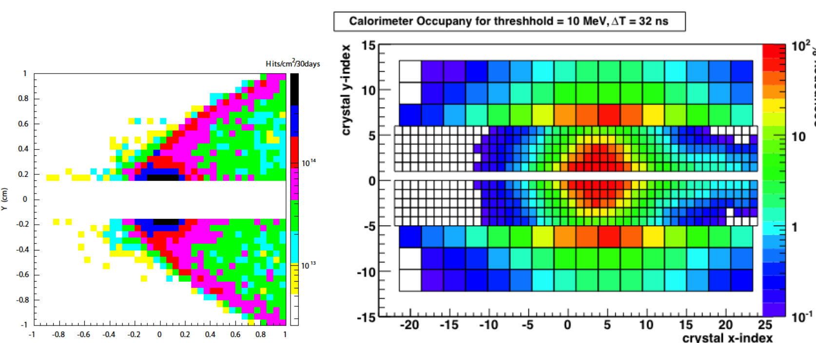
Figure 4: Beam background rates in Layer 1 on the silicon tracker (left) and the electromagnetic calorimeter (right).
