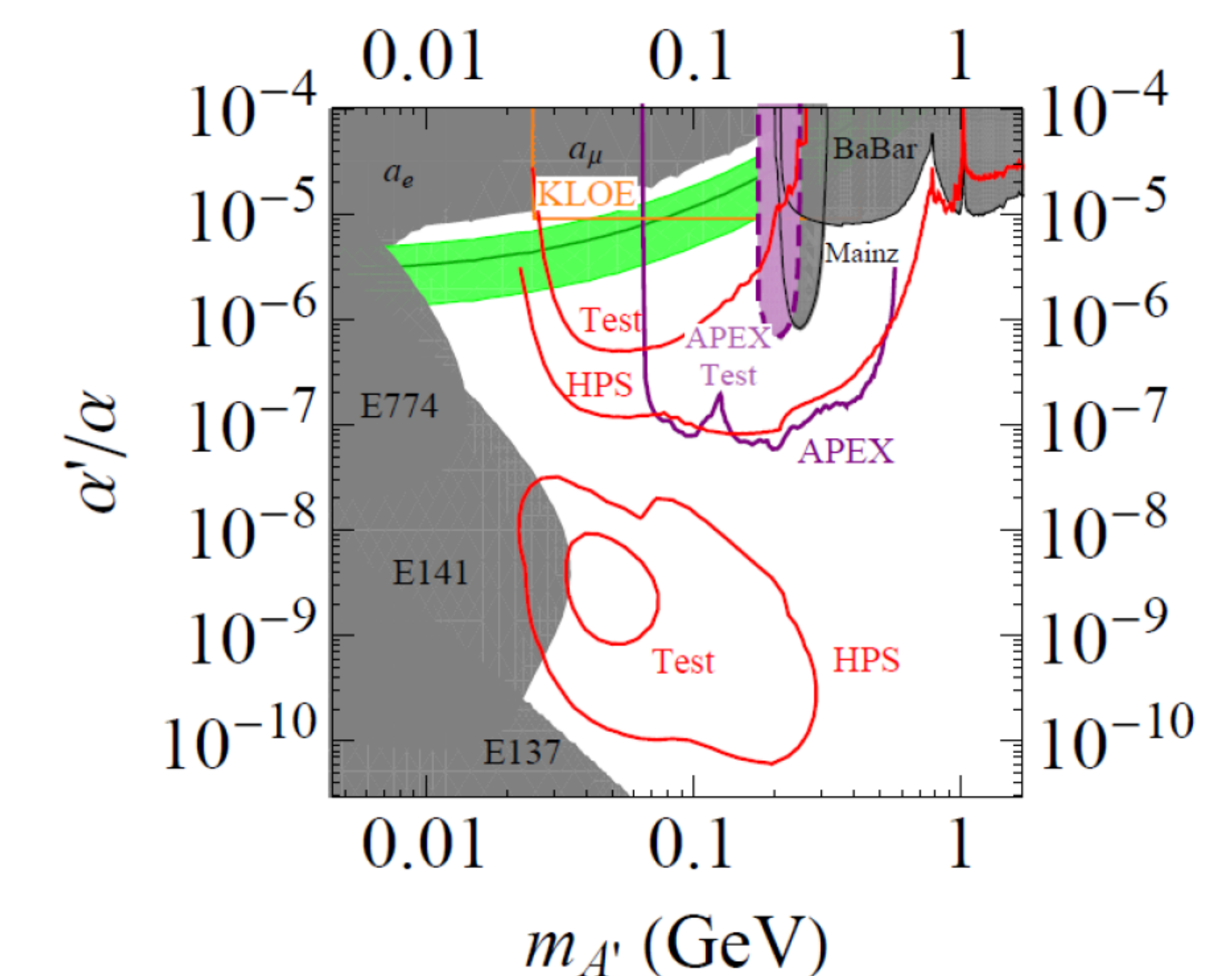
Figure 9: Anticipated reach in \alpha'/\alpha = e^2 for the Heavy Photon Search (HPS) experiment at Hall B in JLab (red lines) with existing constraints on an A' from electron and muon anomalous magnetic moment measurements, the BaBar search for \gamma(3S) \rightarrow \gamma\mu^+\mu^- , and three beam dump experiments, E137, E141, and E774. In addition, we show the projected 2\sigma sensitivities for the proposed "APEX" experiment in JLab Hall A (purple), recent results from Mainz and KLOE, and the parameter space suggested by ascribing the discrepancy in muon g-2 measurements to the heavy photon (green). The upper solid red lines correspond to the 2\sigma sensitivity of a full resonance search, and the lower solid red lines to the vertex search for HPS. The inner red lines show the reach of the HPS Test Run experiment.
