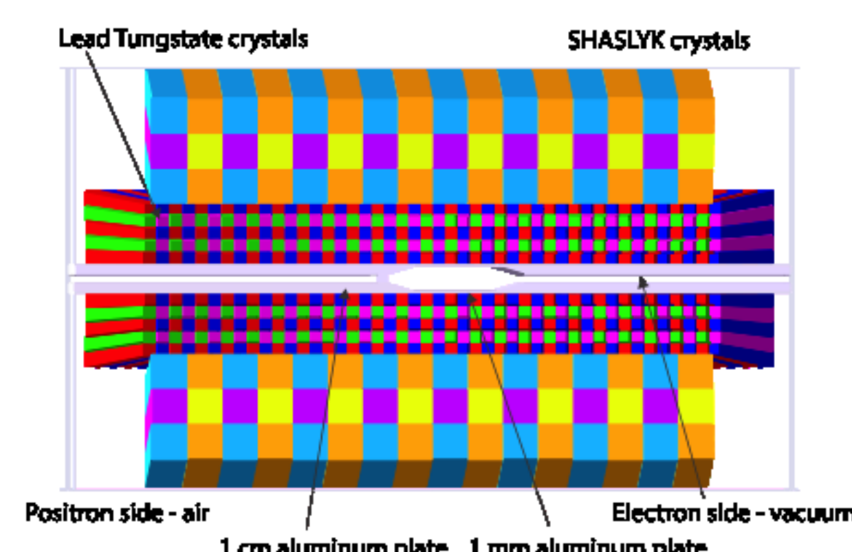
Figure 7: A rendering of the electromagnetic calorimeter setup looking down the beam line.
