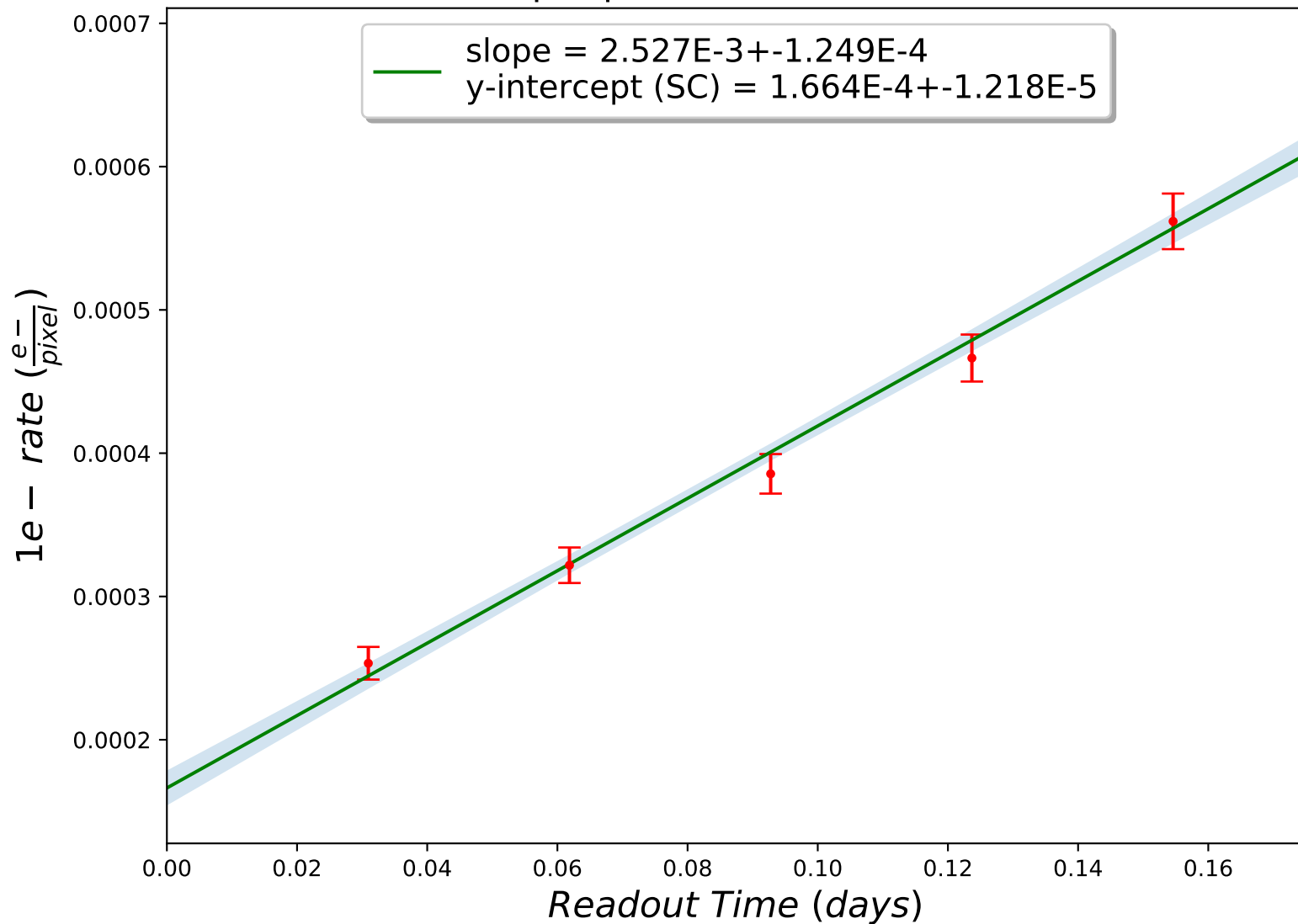
# of e- per pixel versus readout time.
