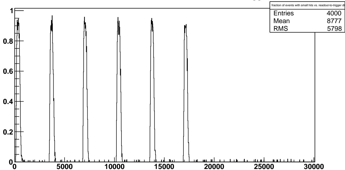
fraction of events with small hits vs. readout-to-trigger dt
