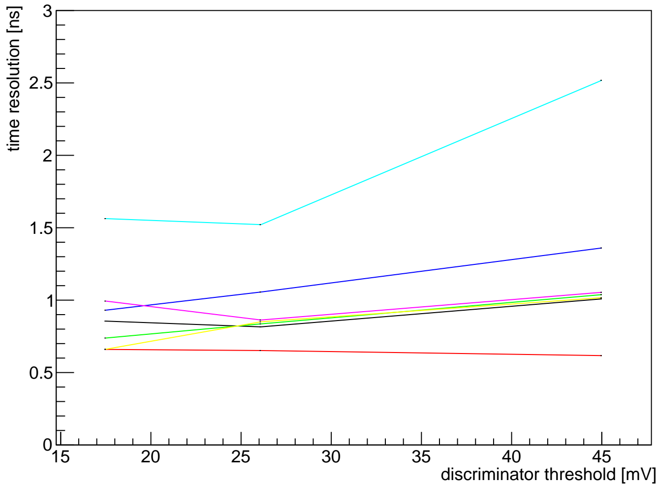
time resolution vs. threshold, nominal bias
