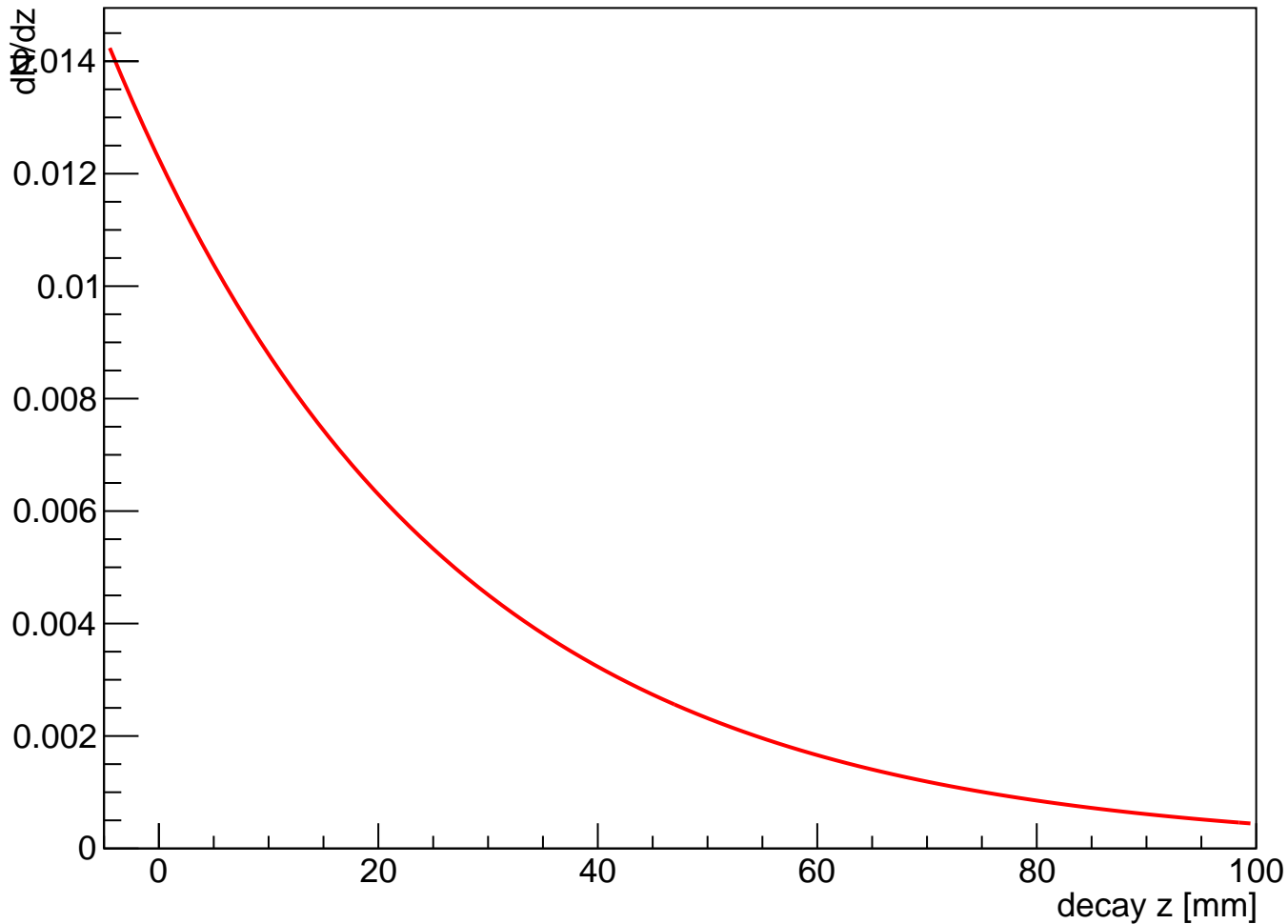
Decay distribution, 50 MeV heavy photon, gammact=30 mm
