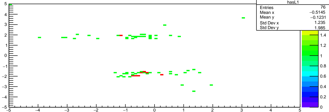
fspFirstHitY:fspFirstHitX {fspHasL1&&fspMatchChisq<5&&fspTrkChisq<25}
