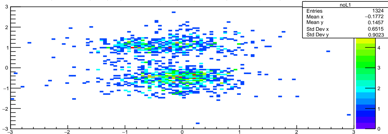
fspTrkZ0+100*fspPY/fspP:fspTrkD0+100*fspPX/fspP {!fspHasL1&&fspMatchChisq<5&&fspTrkChisq<25}
