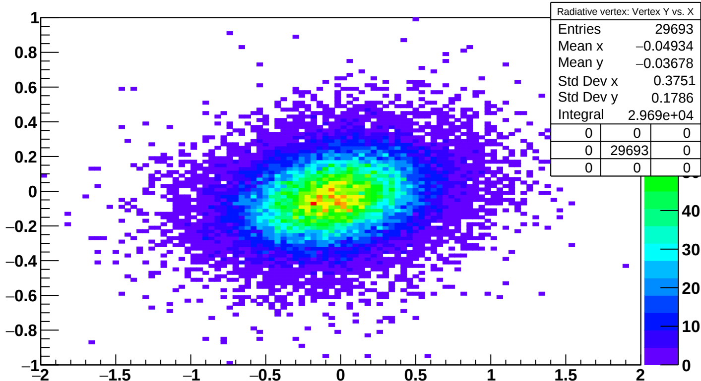
Radiative vertex: Vertex Y vs. X
