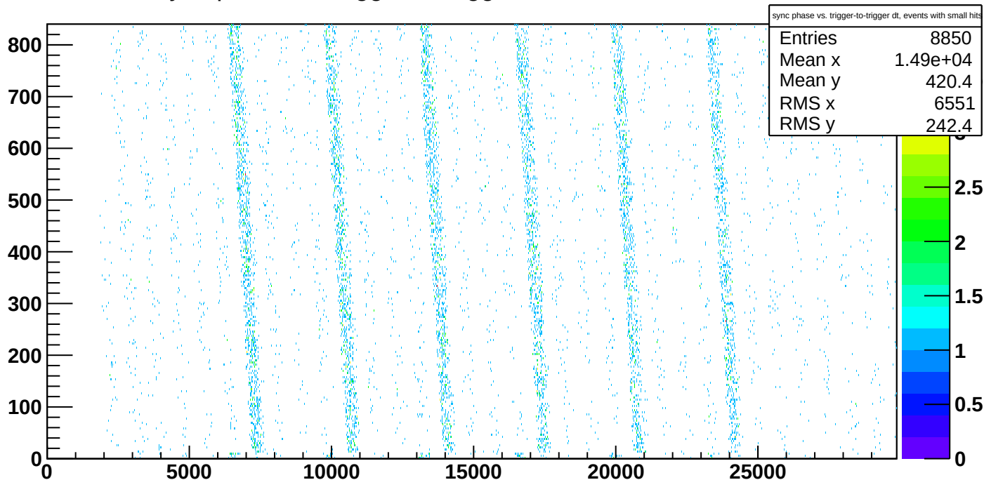
sync phase vs. trigger-to-trigger dt, events with small hits
