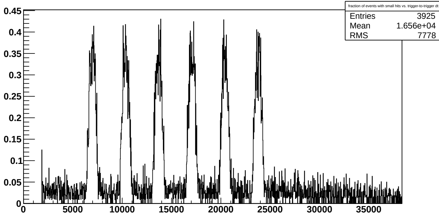
fraction of events with small hits vs. trigger-to-trigger dt
