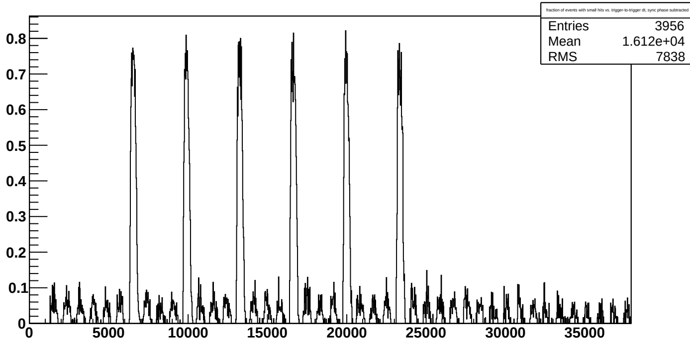
fraction of events with small hits vs. trigger-to-trigger dt, sync phase subtracted
