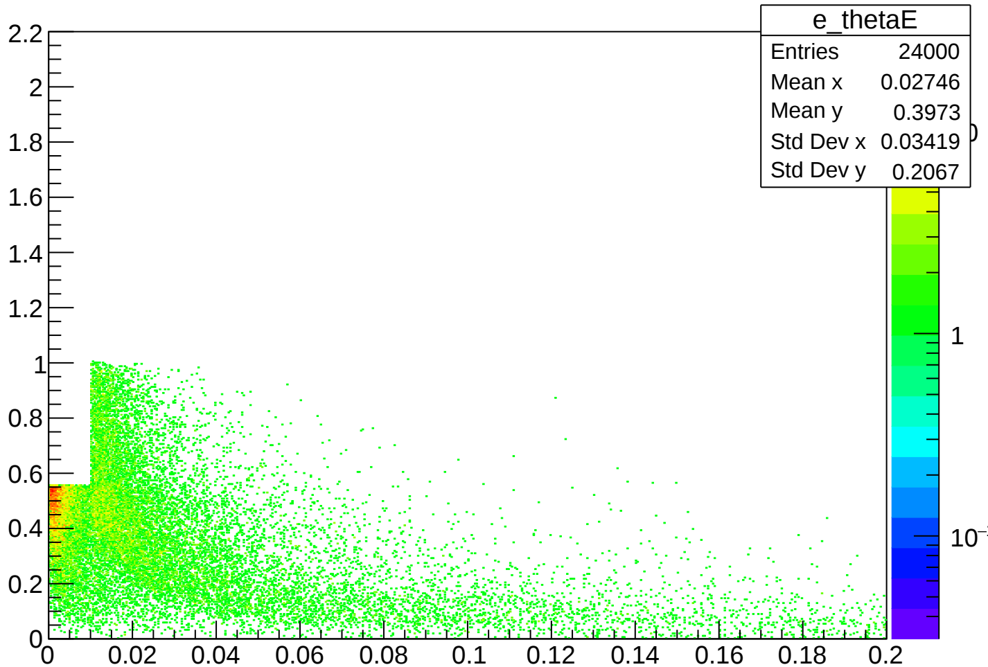
electron E vs. theta
