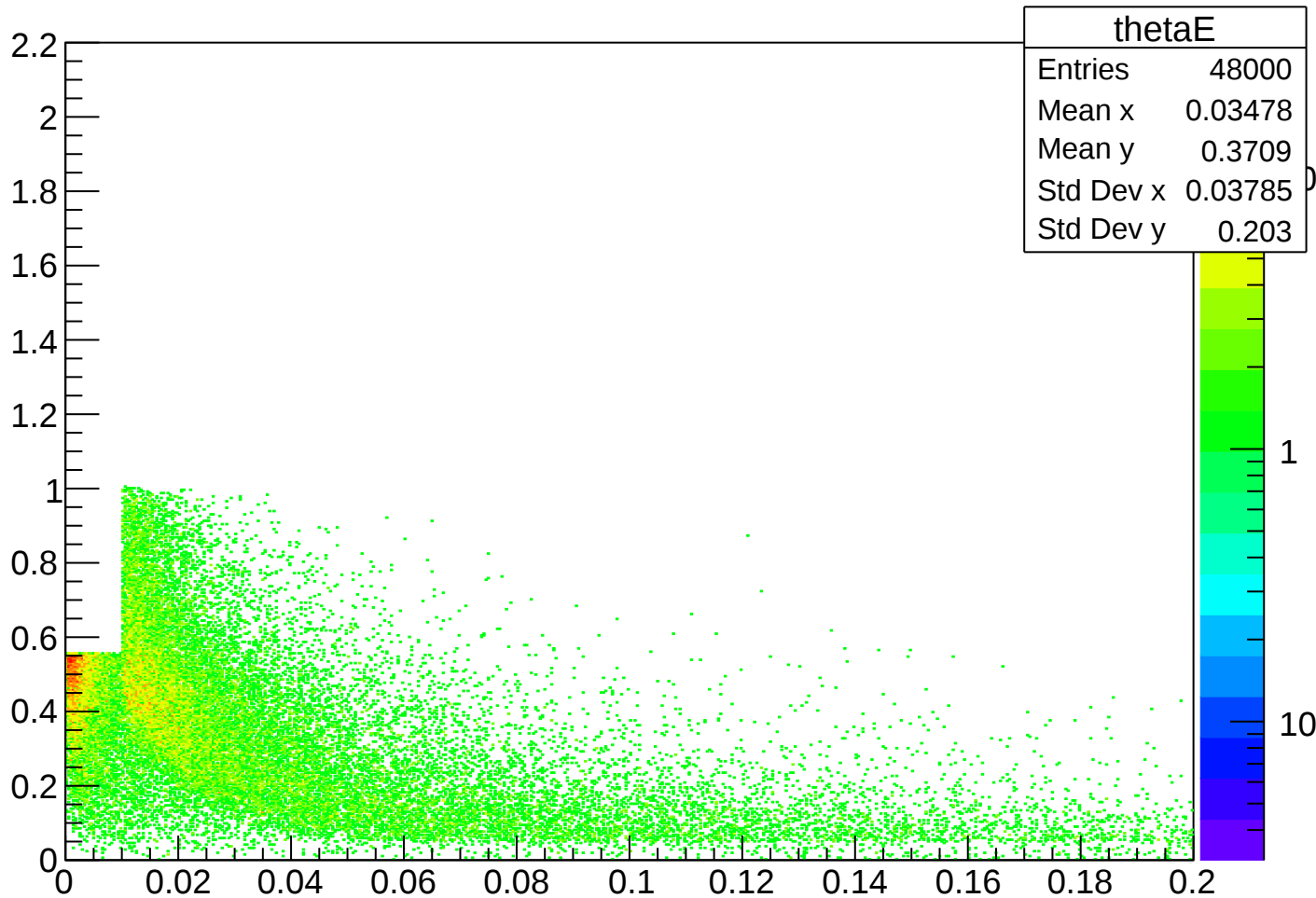
E vs. theta
