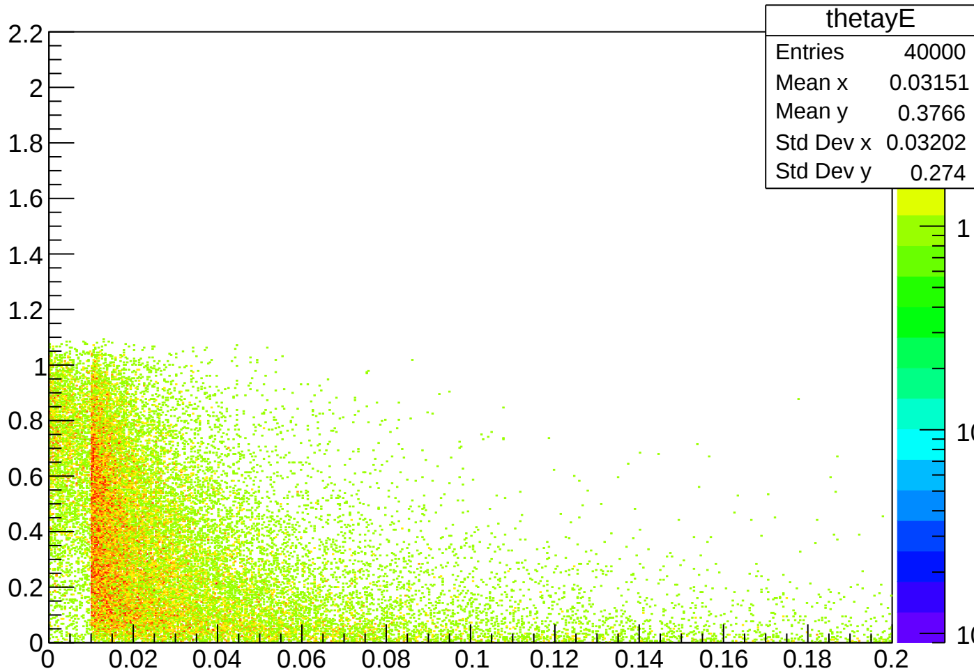
E vs. theta_y
