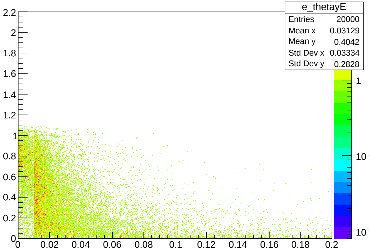
electron E vs. theta_y
