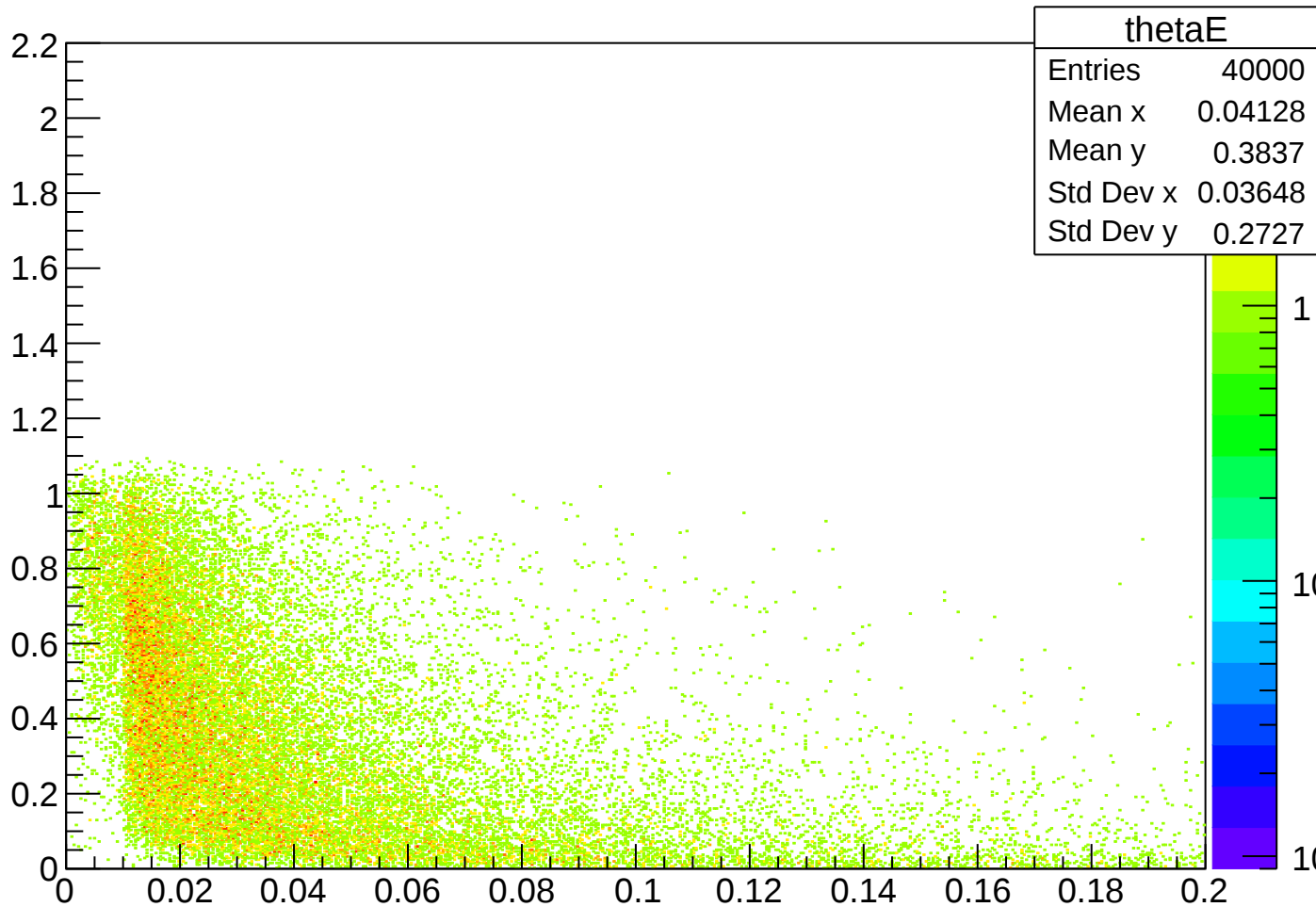
E vs. theta
