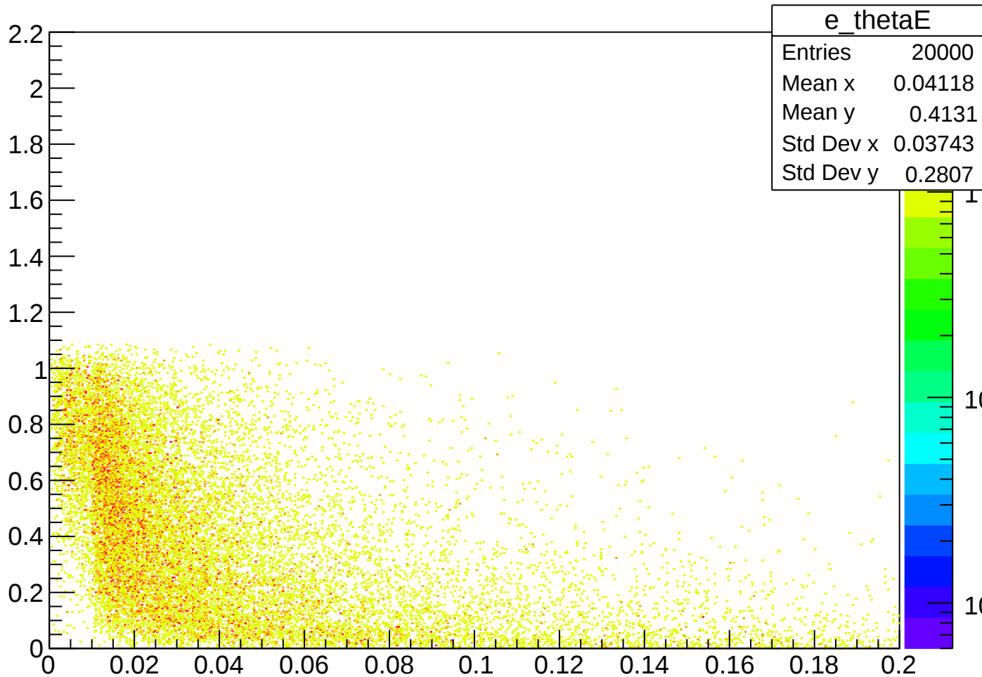
electron E vs. theta
