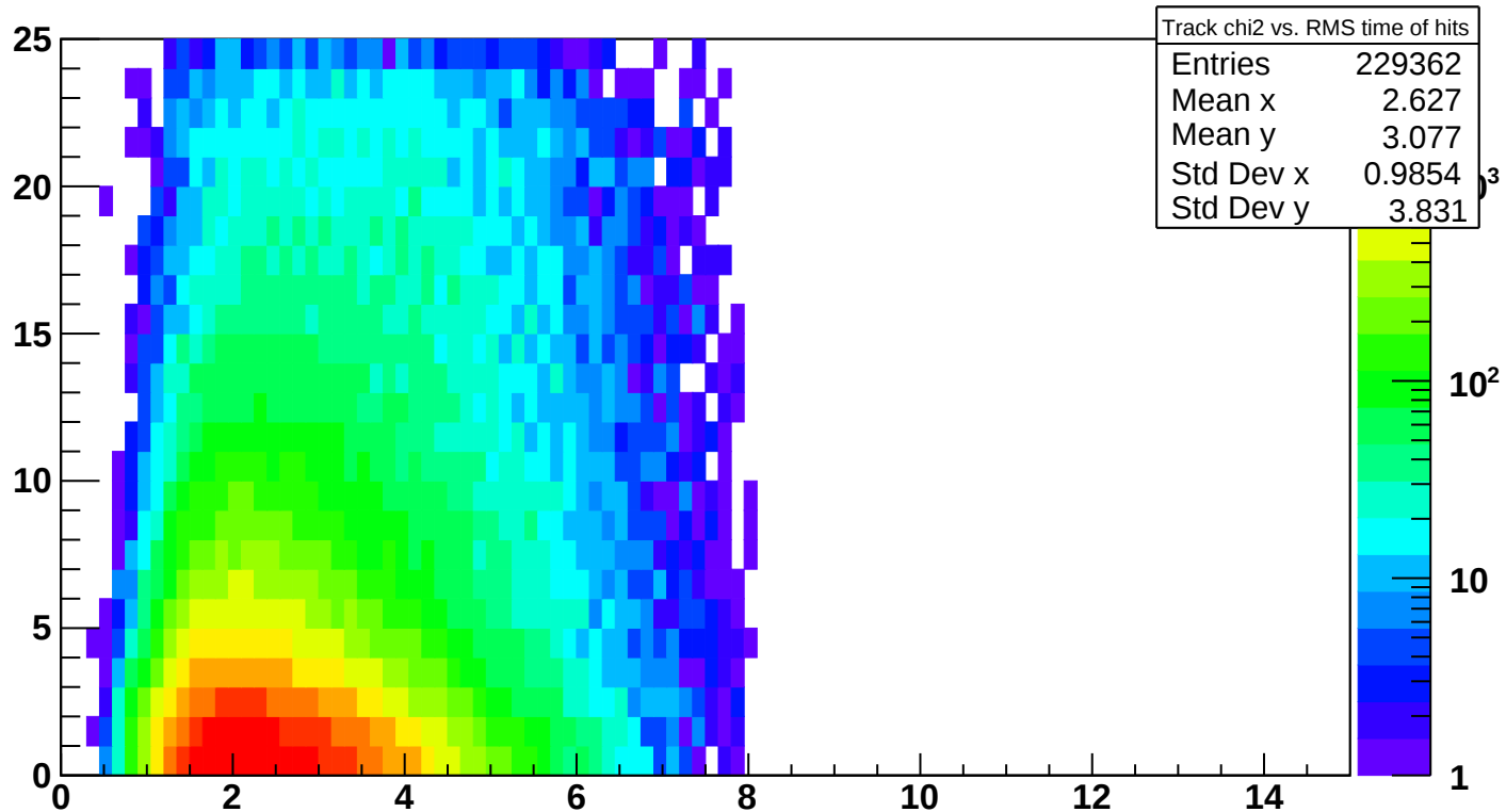
Track chi2 vs. RMS time of hits
