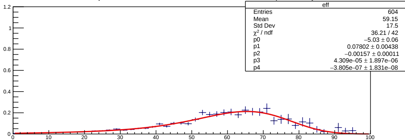
triEndZ {triP>0.8*1.056&&bscP>0.8*1.056&&eleHasL1&&!posHasL1}
