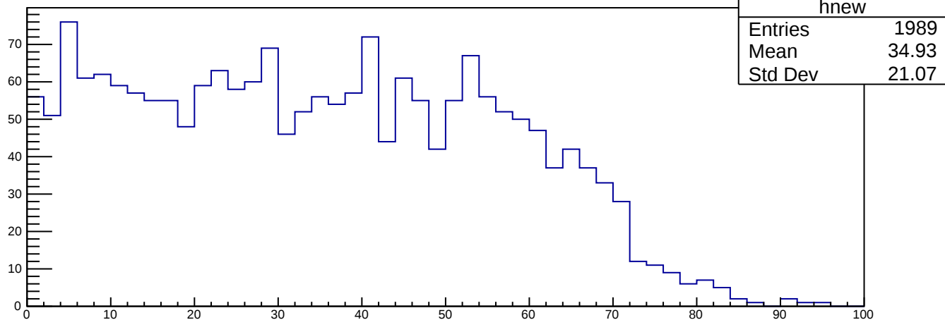
triEndZ {triP>0.8*1.056&&bscP>0.8*1.056&&eleHasL1&&!posHasL1}
