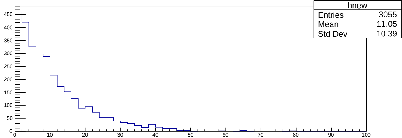
triEndZ {triP>0.8*1.056&&bscP>0.8*1.056&&eleHasL1&&posHasL1}
