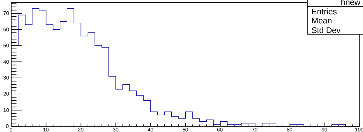
triEndZ {triP>0.8*1.056&&bscP>0.8*1.056&&eleHasL1&&!posHasL1}
