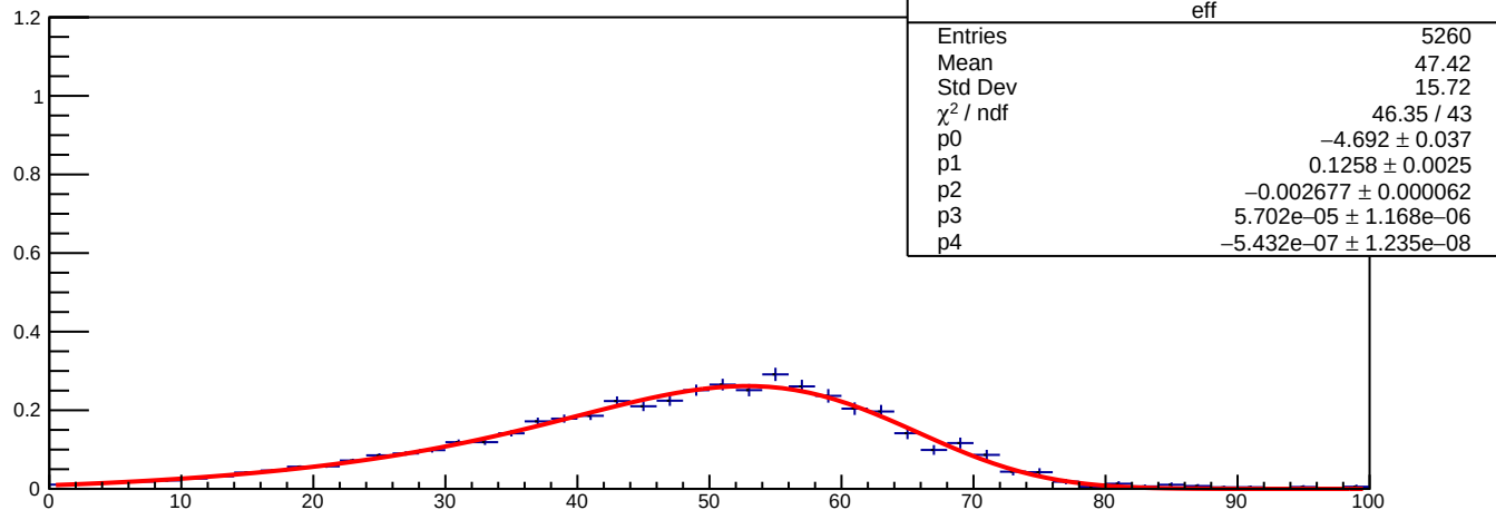
triEndZ {triP>0.8*1.056&&bscP>0.8*1.056&&eleHasL1&&!posHasL1}
