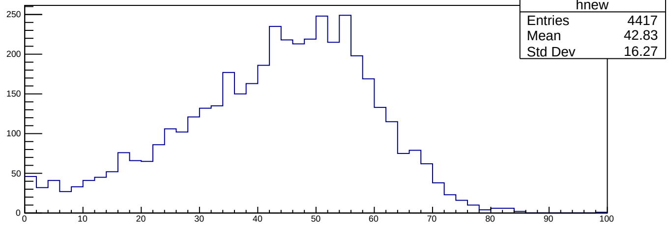
triEndZ {triP>0.8*1.056&&bscP>0.8*1.056&&!eleHasL1&&posHasL1}
