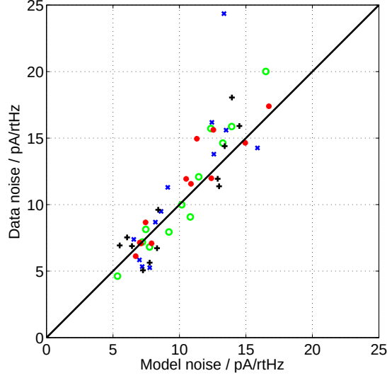
Figure 2.9: Correlation of predicted and observed phonon noise at 20 kHz. Each symbol represents one channel of one detector: PA (x), PB (o), PC (*), PD (+). All twelve detectors are shown, using noise traces from the data set 140808_1920.
