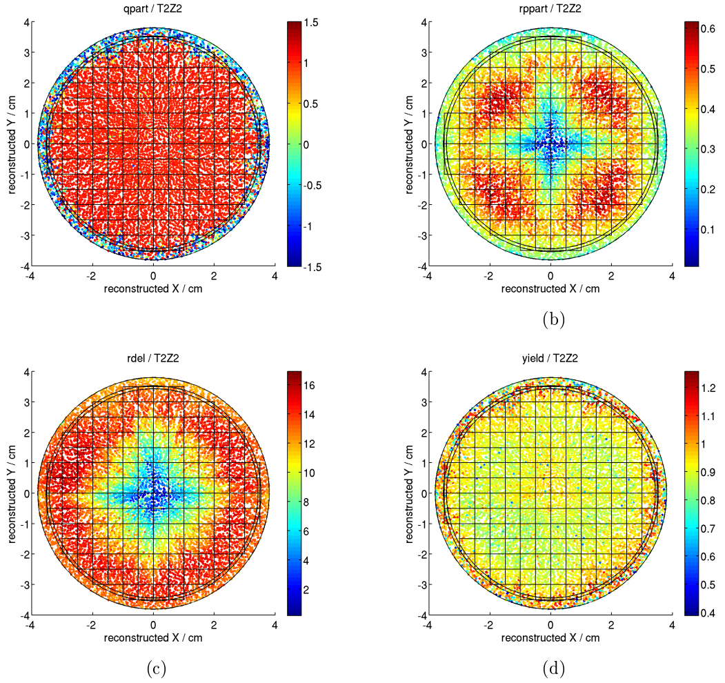
Figure 6.9: Results of the position reconstruction for detector T2Z2. Reconstructed x and y are calculated from corrected \theta , and r after the last R-step.
