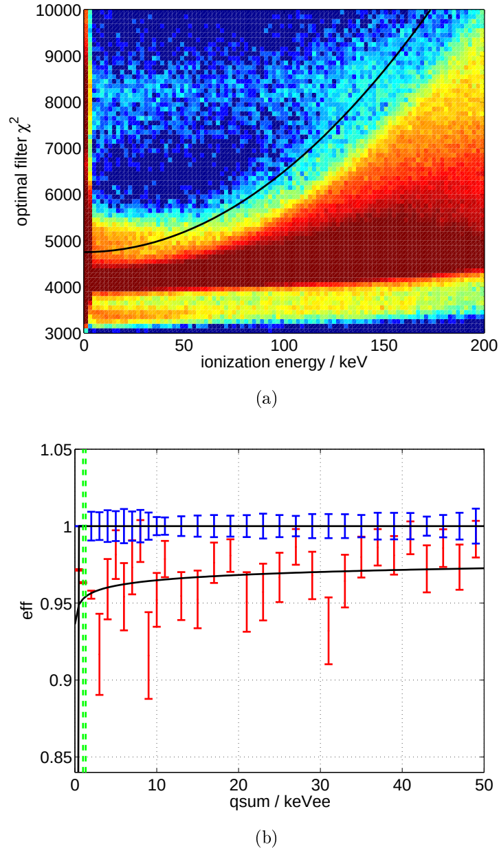
Figure 8.7: In (a), the ionization channel chi-squared cut in T1 Z5. The data shown are barium calibration events. The events along the left edge of the plot are electronic glitches, which can make large signals but don't resemble real pulses. The faint second band at \chi^2 values around 8000 comes from the activity of the sliding seal heater. In (b), the efficiency of the chi-squared cut in T1 Z5. The upper (blue) error bars are from Run 119, with nearly 100% efficiency. The lower (red) error bars are from Run 118, with efficiency reduced by a few percent because of the sliding seal heater noise.
