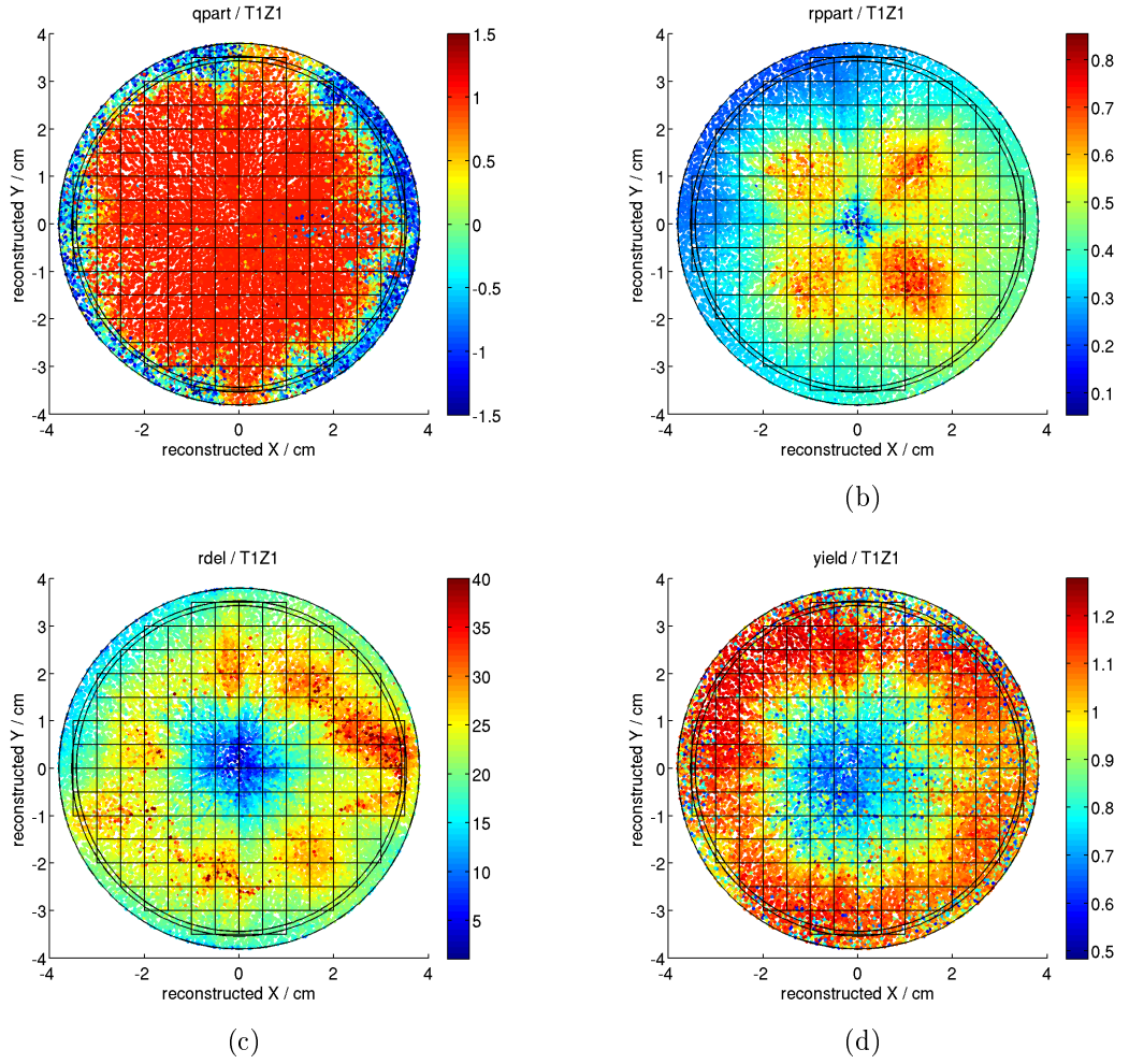
Figure 6.7: Results of the position reconstruction for detector T1Z1. Reconstructed x and y are calculated from corrected \theta , and r after the last R-step.
