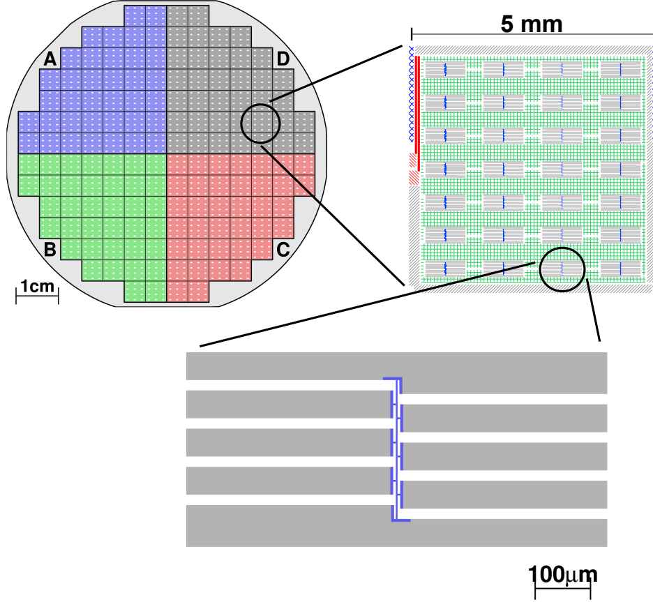
Figure 2.5: QETs on a ZIP detector. At upper left, the entire phonon side: each quadrant has 37 5\text{mm}\times 5\text{mm} dies. The area outside the stairstep boundary of the phonon sensors is covered with metal grid, and is electrically isolated in some detectors. At upper right, a single die with 28 TESs surrounded by Al grid (green crosshatch). The horizontal stripes of grid bias the TESs, with one stripe at the bias voltage and the next at ground. Around the periphery are bias rails (grey diagonal hatch), wire bonding pads (red horizontal hatch), and alignment marks (blue diagonal crosshatch). Bottom: a single QET, showing the Al absorber fins around the thin W TES.
