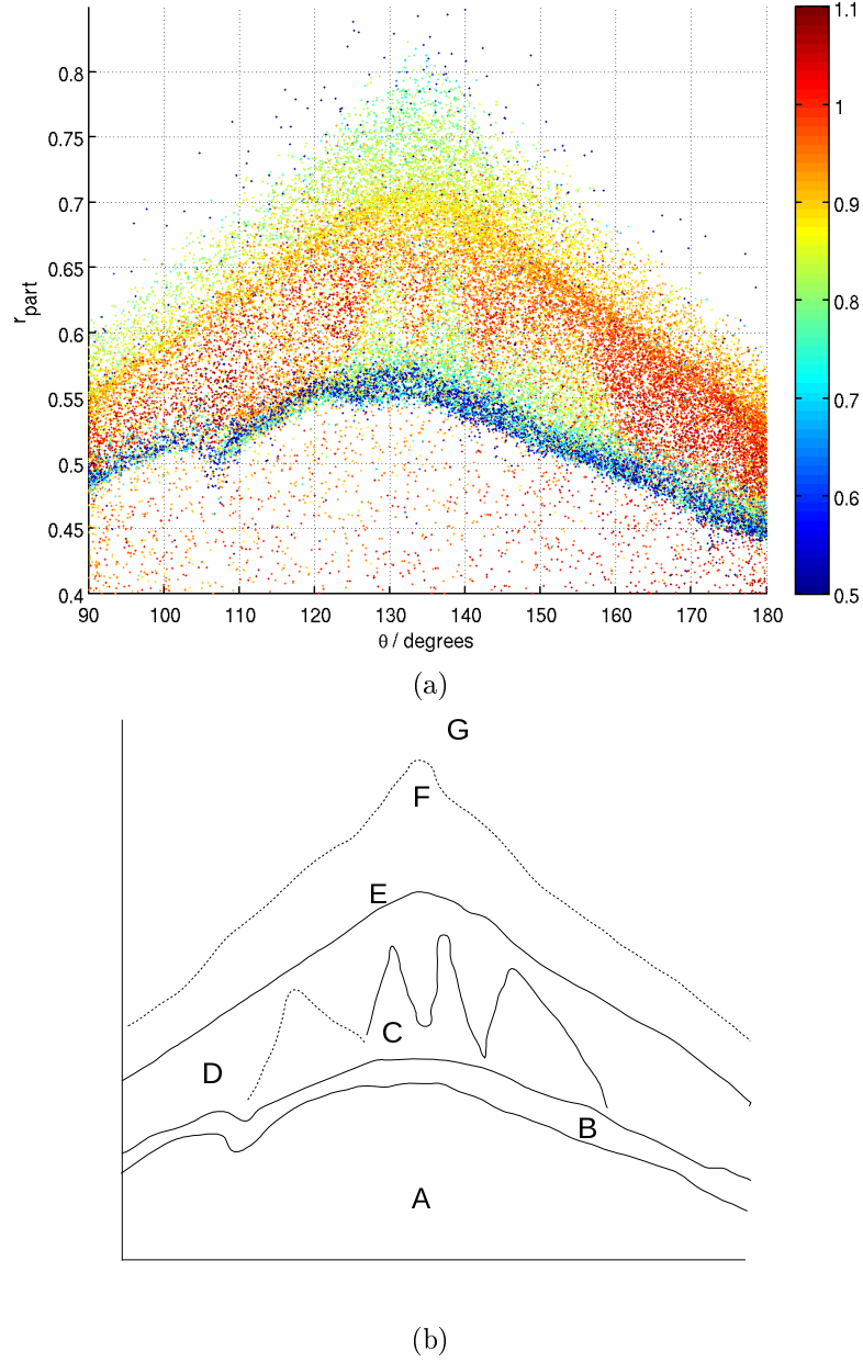
Figure 6.11: Depth sensitivity through phonon partition, in partition radius and angle. The x - y coordinates are similar to one corner of the partition or “box” plot, zoomed in to the top left corner to show only Quadrant A. In this view, the box plot is conveniently shown in r and \theta . Color in (a) is uncorrected ionization yield, and is used to identify the populations of events labeled in (b). The plot covers quadrant A of T1 Z5, in r and \theta from the box plot. The regions are: A , events very near the center of the detector; B , outer electrode events; C , “holiday island” events; D , bulk inner electrode events; E , the foldback point for Q-side events; F , the foldback point for P-side events; and G , P-side surface events.
