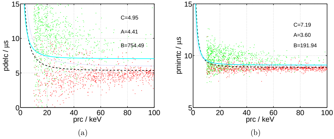
Figure 9.5: Beta timing vs. energy and band edges in data from published Run 119 analysis. Phonon pulse delay is shown in (a), and rise time in (b). The green (light) events are selected neutrons, and red (dark) are surface events from photon calibration data. The curves are as follows: blue, dotted - chosen by eye in published Run 119 timing cut; black, dashed - fitted here using 80% point; cyan, solid - fitted here using 90% point. A single detector, T1 Z5 (Ge), is shown.
