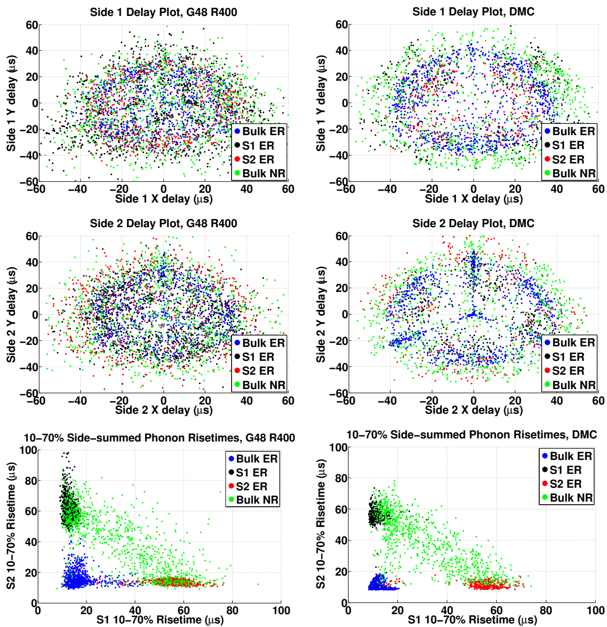
Figure 4-22: Comparison of iZIP4 phonon parameters from data (left) and simulation (right)
