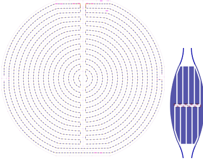
(a) Figure 4-6: Illustration of the mask design of the iZIP3 detector. The thicker, ‘dashed-looking’ lines are the phonon channels, and each ‘dash’ is an individual QET, pictured to right of the image. The thinner lines are the ionization rails.
