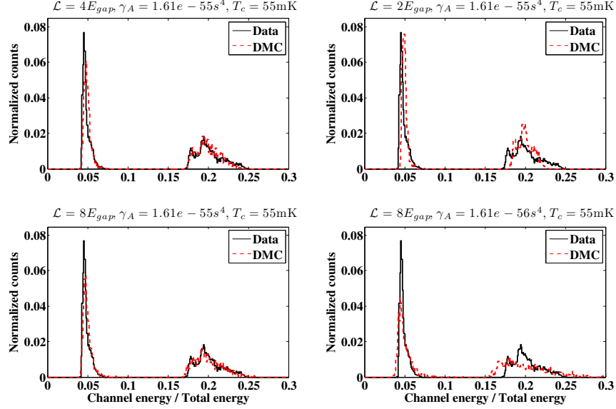
Figure 4-9: Histograms of the fraction of energy in the eight phonon channels from data (black solid line) and four different simulation runs (red dashed line). The smaller outer channels each collect \sim 5\% of the energy, while the larger inner channels are distributed around 20%. Increasing \mathcal{L} and increasing \gamma_A both increase the degree of partitioning (the breadth of the histogram), as expected.
