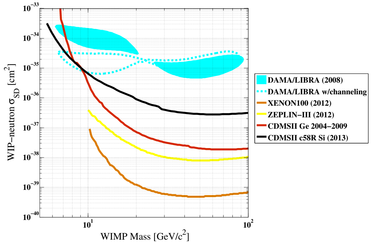
Figure 8-10: Limit on the spin-dependent WIMP-neutron cross-section from this analysis. Results from other direct dark matter searches are included for comparison.
