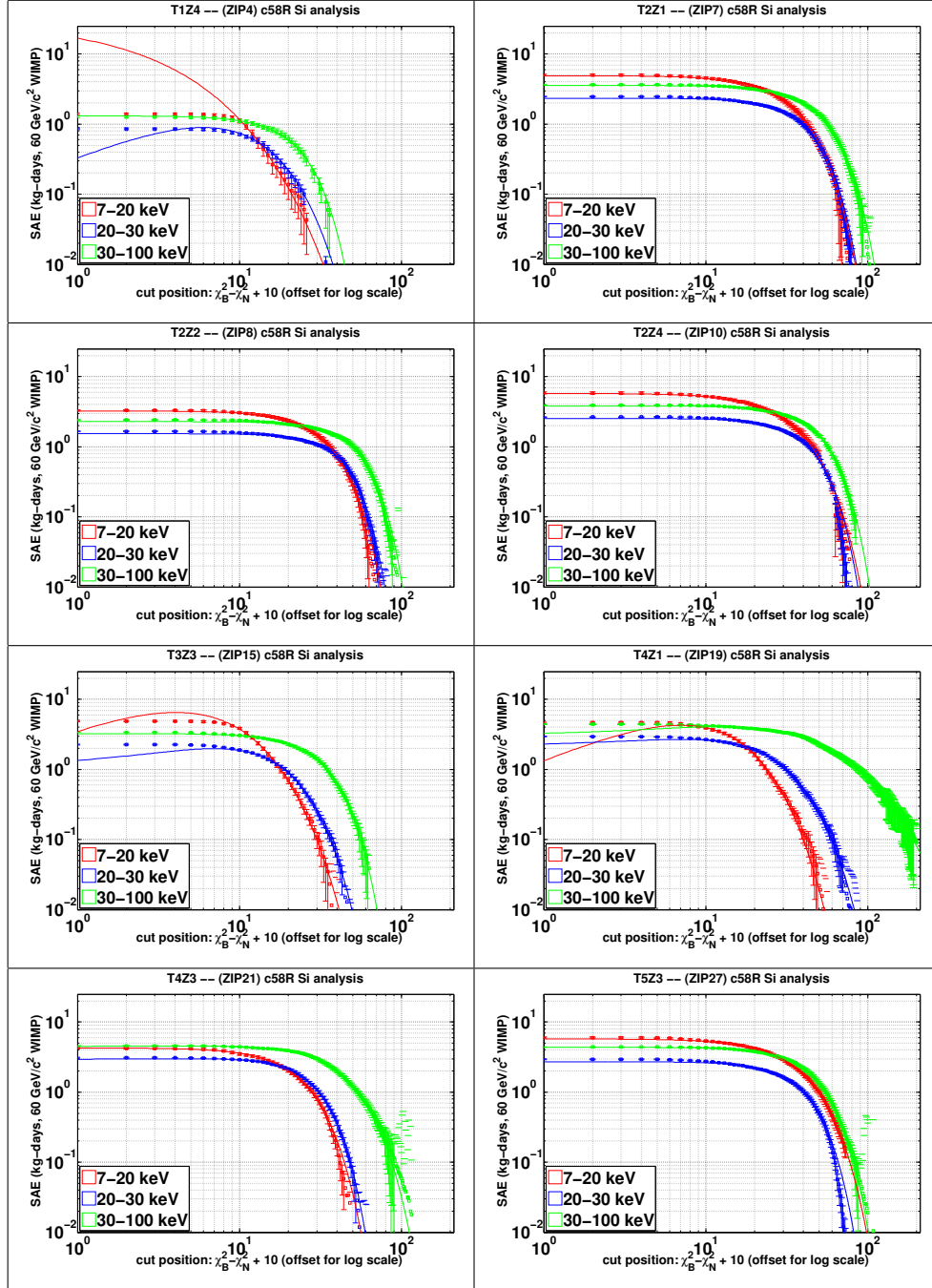
Figure 7-33: Measured and fit Spectrum-Averaged Exposure to a 60 \text{ GeV}/c^2 WIMP vs. rejection cut position in all detectors in recoil energy bins: 7-20 keV (red), 20-30 keV (blue), 30-100 keV (green). The cut position is offset by 10 to allow negative cut values to appear on the log scale x-axis. The fit is only required to be good at values of the rejection parameter >10 .
