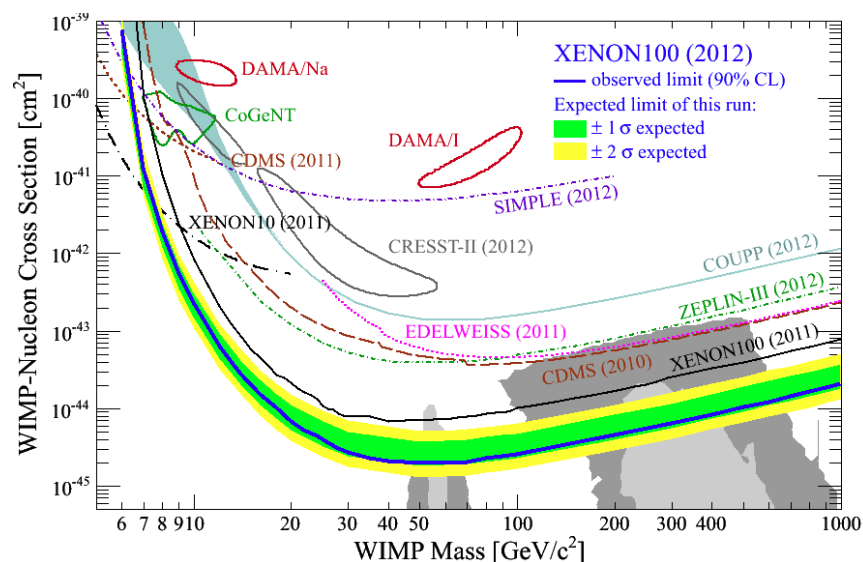
Figure 2-3: Recent limits and regions of interest in the WIMP mass and cross-section plane from a variety of direct dark matter search experiments. Figure from [70]
