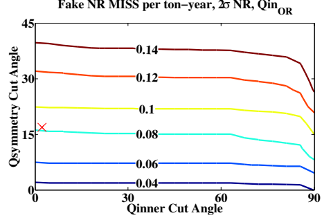
(b) Same as 5-10(a), using Q_{inner} OR rather than Q_{inner} AND. When the OR cut is used, the MISS rate becomes very sensitive to the symmetry cut, as the Q_{symmetry} cut acts as the only cut constraining both charge sensors.
