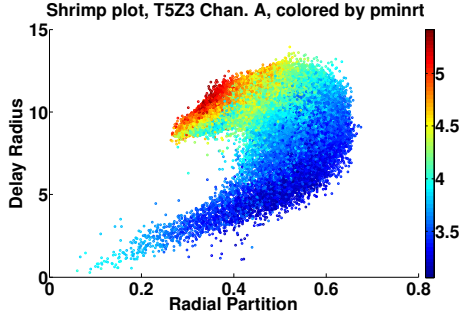
(a) Shrimp plot colored by measured p_{\text{minrt}} from Run 126, Detector T5Z3, Channel A. [139]
