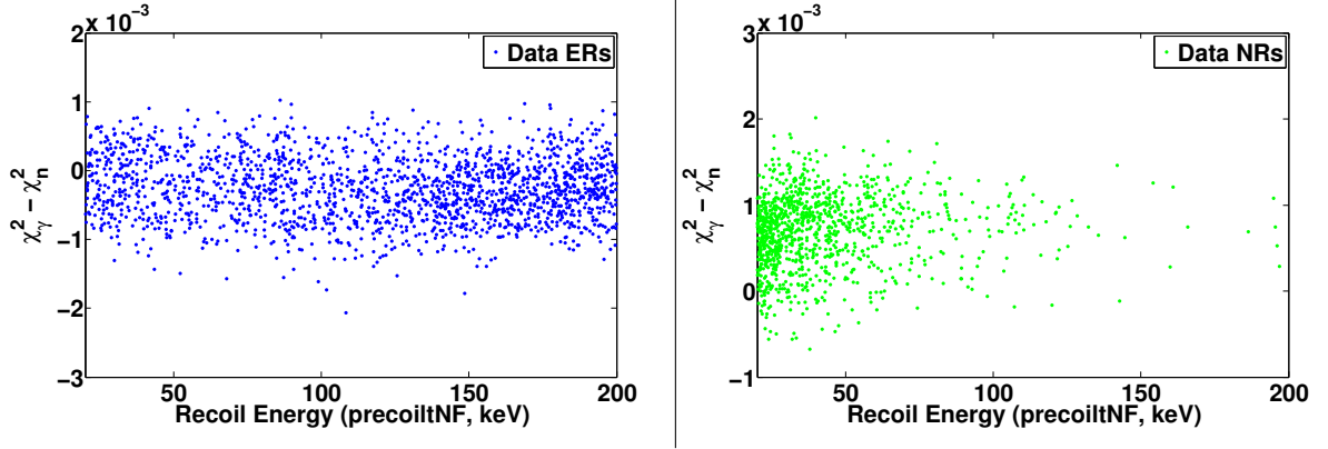
Figure 6-6: Recoil energy dependence of the rejection parameter for electron recoils (left) and nuclear recoils (right) when matching all 8 phonon pulses.
