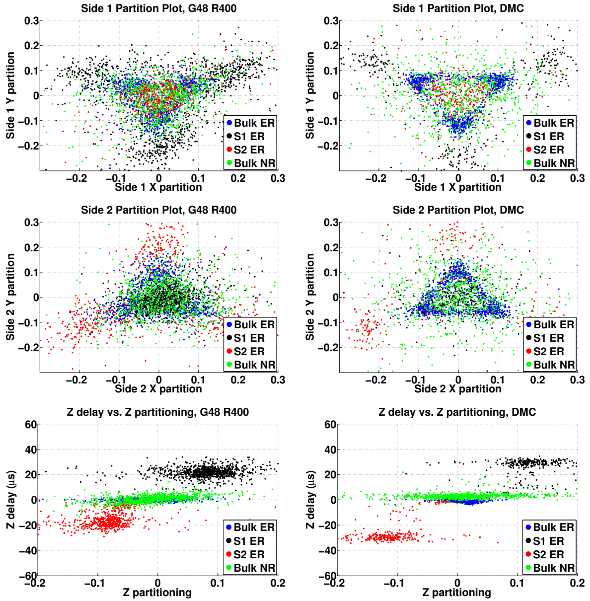
Figure 4-21: Comparison of iZIP4 phonon parameters from data (left) and simulation (right)
