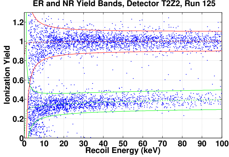
Figure 7-24: The yield bands for electron recoils (red) and nuclear recoils (green) vs. event energy. The mean yields of the ER and NR bands are presented as dashed lines, and the \pm 2\sigma limits are indicated by solid lines.
