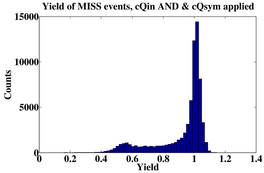
Figure 5-8: Histogram of MISS event yields from events passing the ionization fiducial volume cuts ( Q_{in,AND} & Q_{sym} ). The MISS candidate sample contains large fraction of true bulk events with yields around 1. The expected secondary population of well-collected true MISS events around 0.5 in yield is also evident. The tail of yields below the secondary peak arises due to MISS events with incomplete ionization collection in one or both of the surface scatters.
