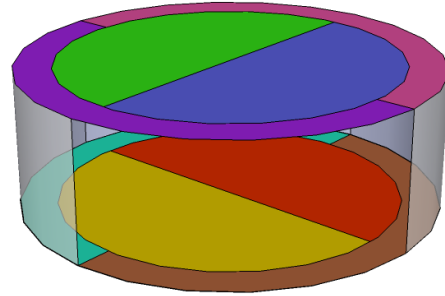
(b) Schematic of an iZIP3 detector, illustrating the 4 TES channels on both sides. The inner ionization channel extends throughout the three inner phonon channels, and the outer ionization channel occupies the same space as the outer phonon channel.
