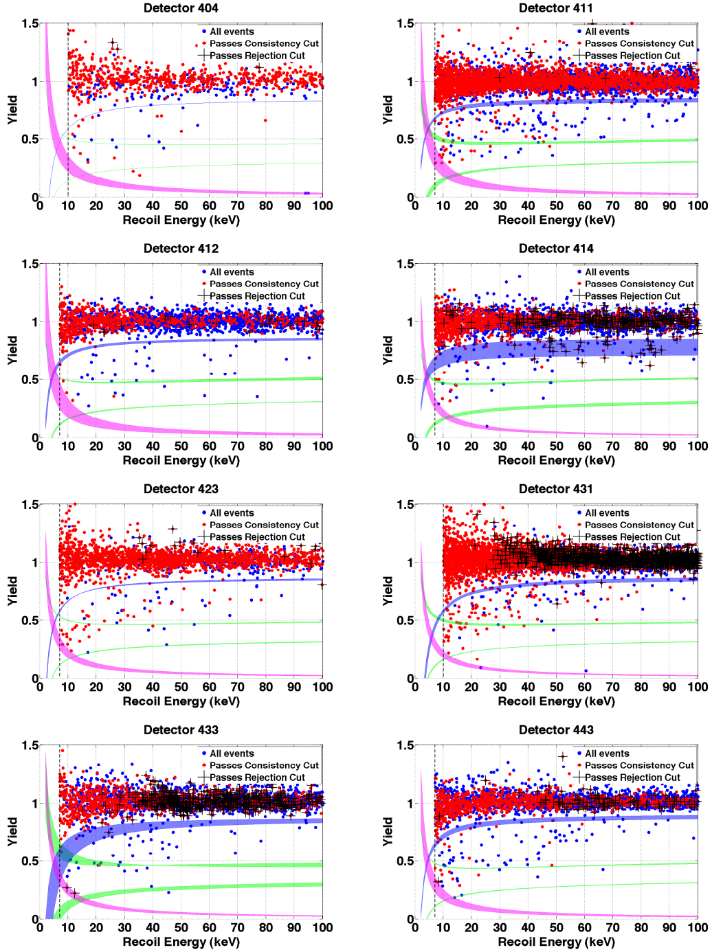
Figure 8-3: Yield (yic) vs. recoil energy (pric, keV) of all good low-background events from Runs 125-128 in the 8 Si detectors of this analysis. Events in red pass the neutron consistency cut, and events with black crosses pass the rejection cut. The signal NR band is outlined in green, the -3\sigma edge of the ER band is in blue, the charge threshold cut is shown in magenta, and the recoil energy threshold is the black dashed line. The width of these lines indicate variations in the band/threshold definitions across runs and series.
