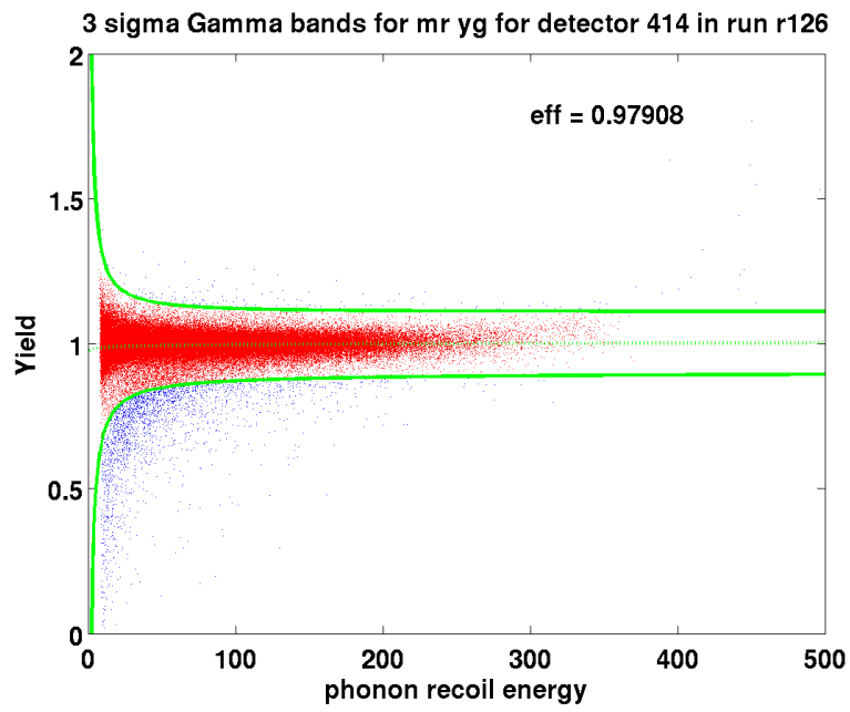
Figure 7-14: Electron recoil band after first-pass correction in Run 126, Detector T2Z4. Events in red pass the first-pass yield cut, while those in blue fail it.[139]
