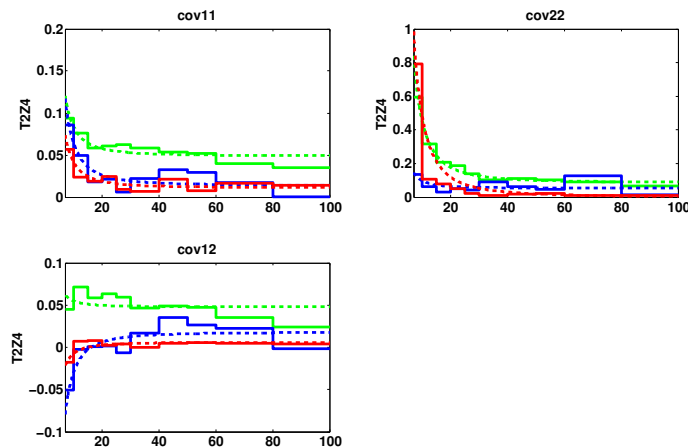
Figure 7-28: Fits of the elements of the covariance matrix between p_{del} and p_{minrt} in Detector T2Z4. Neutrons are shown in green, phonon-side surface events in blue, and charge-side surface events in red. [171]
