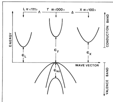
(a) Electron and hole valley structure of germanium, showing the electron L-valley at \langle 111 \rangle , the \Gamma -valley at \langle 000 \rangle , and the X-valley at \langle 100 \rangle . Figure from [97].
