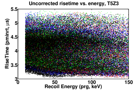
(b) Measured p_{\text{minrt}} vs. pr , Run 126, Detector T5Z3, with the 4 phonon channels distinguished by marker color.[139]
