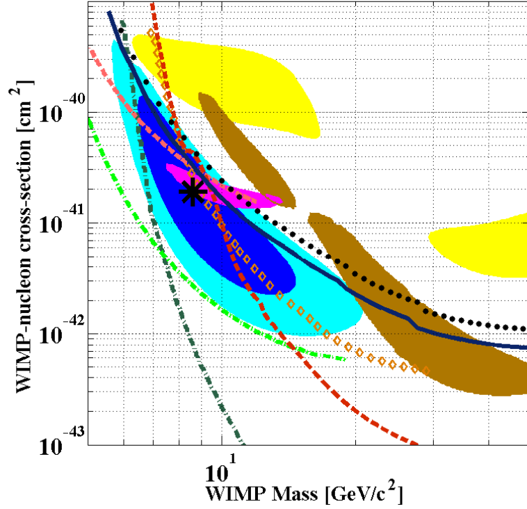
Figure 8-9: Experimental upper limits (90% confidence level) for the WIMP-nucleon spin-independent cross section as a function of WIMP mass. We show the limit obtained from the exposure analyzed in this work alone ( black dots ), and combined with the CDMS II Si data set reported in [181] ( blue solid line ). Also shown are limits from the CDMS II Ge standard [182] and low-threshold [183] analysis ( dark and light dashed red ), EDELWEISS low-threshold ( orange diamonds ) [184], XENON10 S2-only [185] ( light dash-dotted green ), and XENON100 [186] ( dark dash-dotted green ). The filled regions identify possible signal regions associated with data from CoGeNT [187] ( magenta , 90% C.L., as interpreted by Kelso et al. including the effect of a residual surface event contamination described in [188]), DAMA/LIBRA [189, 190] ( yellow , 99.7% C.L.), and CRESST [191] ( brown , 95.45% C.L.) experiments. 68% and 90% C.L. contours for a possible signal from these data are shown in blue and cyan, respectively. The asterisk shows the maximum likelihood point at (8.6 GeV/c 2 , 1.9 \times 10^{-41} cm 2 ).
