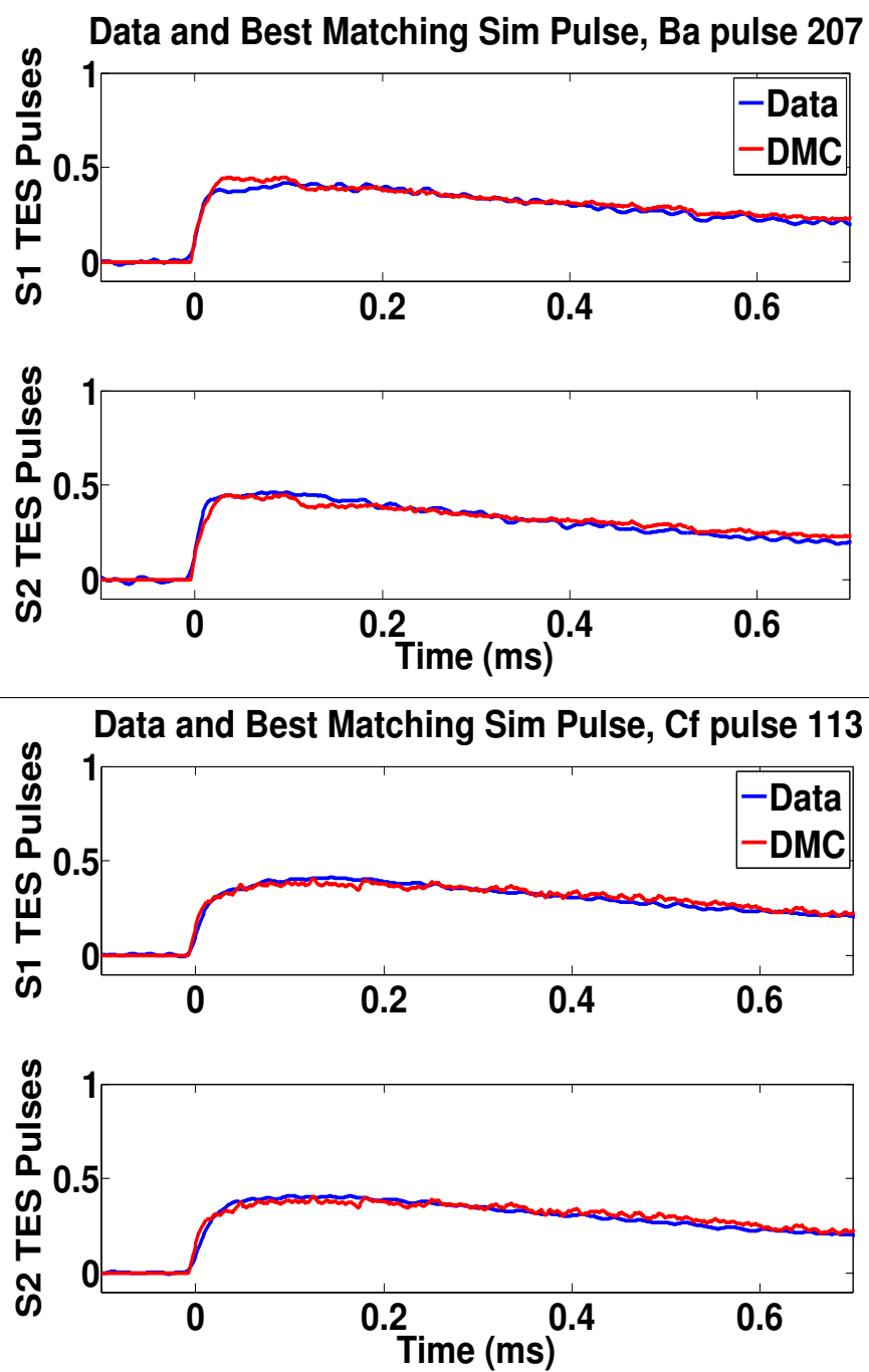
Figure 6-3: Best-matching DMC pulses for a correctly identified electron recoil (top) and nuclear recoil (bottom), zoomed on the first 700 \mu\text{s} of the event.
