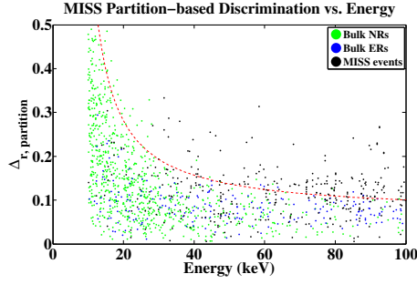
(a) \Delta r_{\text{part}} vs. recoil energy for bulk ERs, bulk NRs, and MISS events, from iZIP4 DMC. A proposed MISS identification cut is shown in red.
