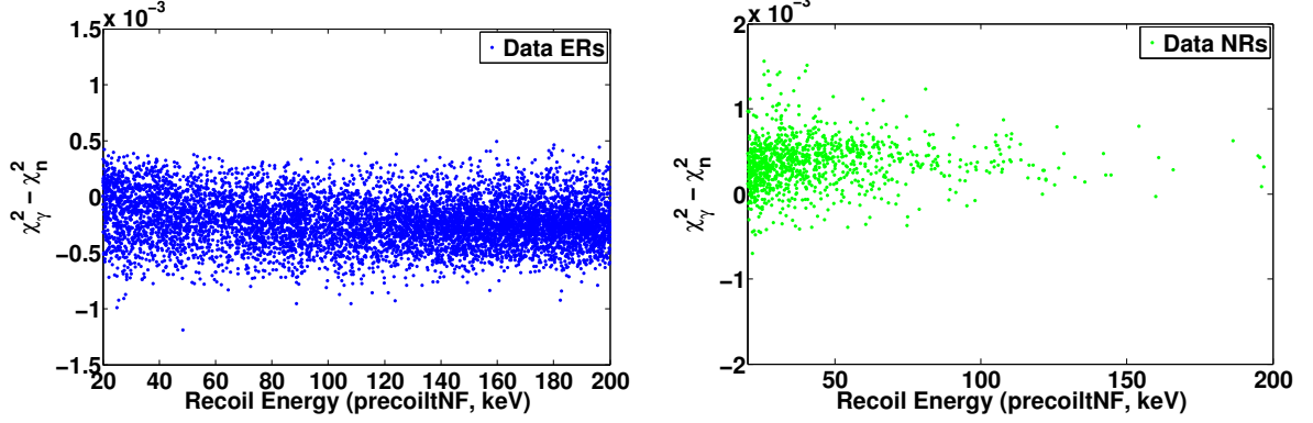
Figure 6-2: Recoil energy dependence of the rejection parameter for electron recoils (left) and nuclear recoils (right)
