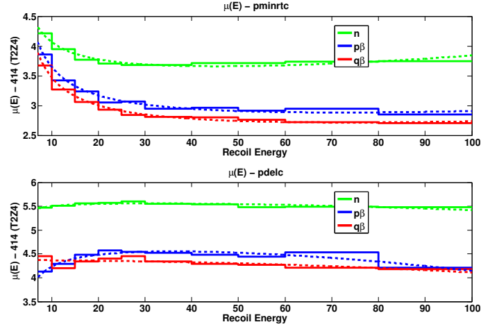
Figure 7-27: Fits of the mean pdele and pminrt in Detector T2Z4. Neutrons are shown in green, phonon-side surface events in blue, and charge-side surface events in red. [171]
