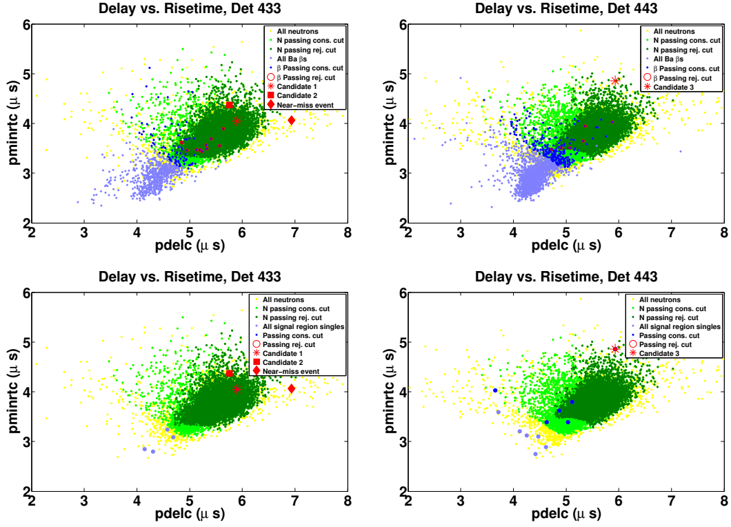
Figure 8-5: Phonon delay vs. phonon risetime in the two detectors containing the three WIMP candidates. The top row shows the neutrons and barium surface event calibration sets, along with the candidate events. The bottom row shows the neutrons, the candidate events, and all other signal region singles in these two detectors.
