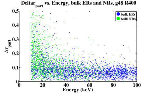
(b) \Delta r_{\text{part}} vs. recoil energy for bulk ERs and bulk NRs from g48 R400. A cut similar to that shown in 5-15(a) may be useful for identifying MISS events at higher energies, where the bulk ERs and NRs are fairly well constrained, and the events at high \Delta r_{\text{part}} can be identified as ERs or NRs and separated from MISS events based on the ionization yield.
