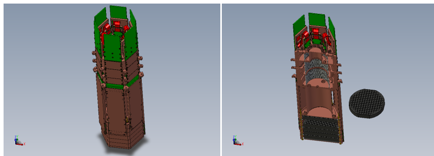
Figure 7-7: CAD rendering of a fully assembled detector stack: detectors, towers, and SQUETS. At right is a cross-sectional view, with one ZIP removed. Courtesy: Patrick Wikus.
