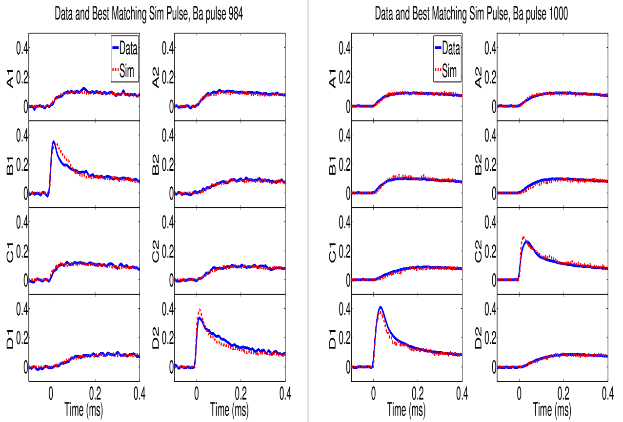
Figure 6-8: Example pulse matches from two correctly identified ERs, showing that the DMC does not seem to match strongly peaked pulses as well as less ‘peaky’ pulses.
