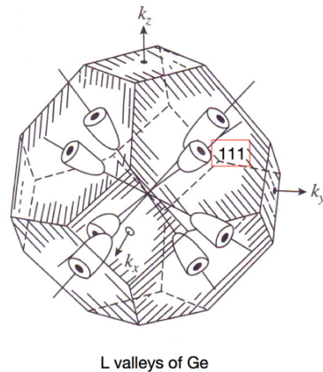
(b) Brillouin zone of germanium, with L-valleys depicted along \langle 111 \rangle axes. The bands are described as ellipsoids with \frac{m_\perp}{m_\parallel} \approx 19.5 . Figure from [97].
