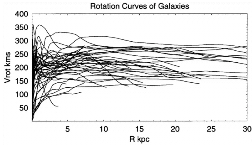
Figure 1-6: Set of galactic rotation curves. Note that the velocity of stars does not decrease at high radius, but rather asymptotes to a constant, indicating an interior mass function M(r) \propto r . As the luminous interior mass grows much more slowly than this, these curves imply contributions from a significant dark matter component [21].
