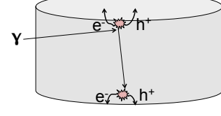
(c) Illustration of a MISS event in the iZIP detector. Both charge species from each scatter are collected and observed only by the nearest electrode. The observed phonon signal will measure the total energy of both scatters, but each ionization electrode will measure only the energy of the local scatter, resulting in a reduced ionization yield.
