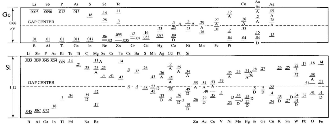
Figure 7.4: Impurity binding energies for a variety of impurity species in Ge (top) and Si (bottom) in eV. Si doesn't have impurity levels below about 33 meV, while Ge has many impurities around 10 meV. This could explain in part the huge difference in leakage behavior between the two substrates for the same environment. These figures do not include overcharged states (which have energies on the order of 1 meV [99] or the possibility of carriers bound in crystal defects. See [85] for an in depth discussion.
