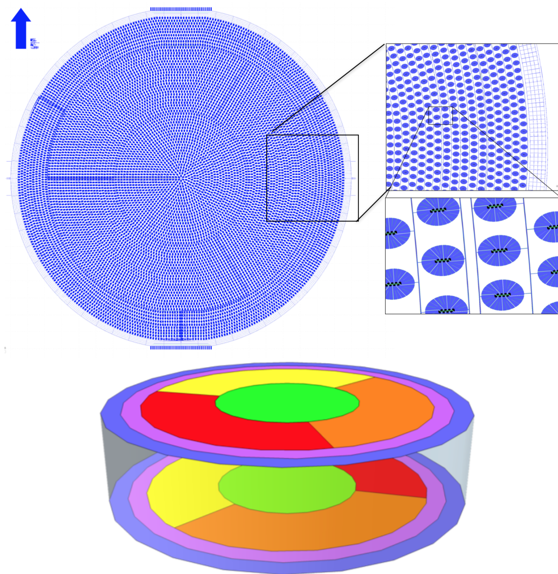
Figure 4.25: Top: Top side detector mask with zoom-in regions showing a fraction of the channel and a subset of QETs. Even in the large image the channel splits and wiring can be clearly seen. Some dead metal is saved by having all QETs share bias lines with those adjacent. QET placement was done to make each channel have equal area and equally space the QETs across the detector face. Bottom: 3D rendering of CDMS HV detector showing the relative rotation of the top and bottom masks.
