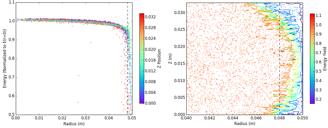
Figure 4.16: Energy yield of events as a function of their initial position in the crystal. Left: Yield versus radius colored by z-position. Right: Radius versus z position near the edge of the crystal with yield shown in color scale. The vertical black line shows where the electrode ends. The result is that the NTL gain is a function of radius and there is radial-z covariance at high radius, limiting the full gain region to about 5 mm from the crystal sidewall.
