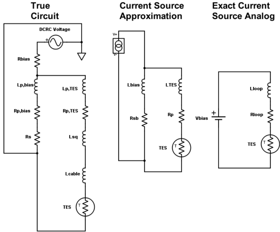
Figure 3.4: TES circuit analogs. Left is the actual circuit, arranged top to bottom by temperature. Middle is a very close approximation, assuming R_{bias} \gg Z_{loop} , which is true for 1\text{ M}\Omega bias resistor in the SNOLAB electronics. Right is exactly equivalent to the middle circuit; resistance and inductance are moved to the right-hand side, and an effective impedance is used to calculate the voltage supplied by the voltage source.
