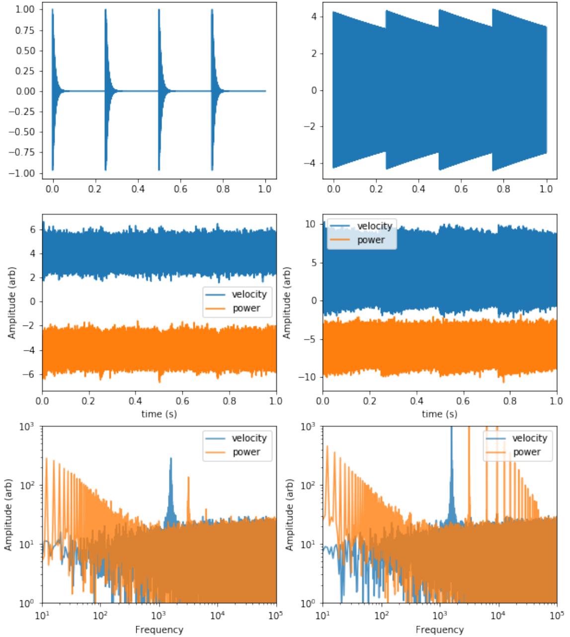
Figure 5.17: A simple vibrational noise model based on the ansatz equation 5.64. Both columns use an oscillation frequency of 1.6 kHz and period of 0.25 seconds, the left column uses a 10 ms decay right and the right column a 1 second decay time. The top row shows the pure signal, the middle shows the signal with noise and the rectified signal with noise, and the bottom shows PSDs for these two signals. We see that both have similar low-frequency noise, but the longer decay time allows for much stronger high-frequency noise.
