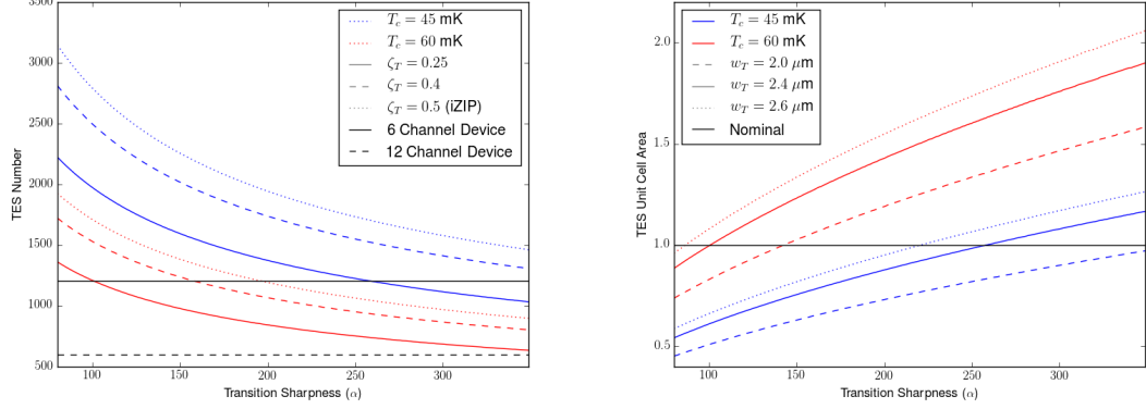
Figure 3.7: Number of QET unit cells as a function of alpha and TES width (left), and as a function of transition sharpness and volume fraction (right), with width and thickness as set in Table 3.1. The third plot shows area per unit cell (assuming 1/6 or 1/12 the area of the crystal surface per channel) as a function of transition sharpness and TES width, using zeta=0.25. The horizontal lines denote the number of unit cells assuming a nominal area of one square millimeter for a 6 and 12 channel face.
