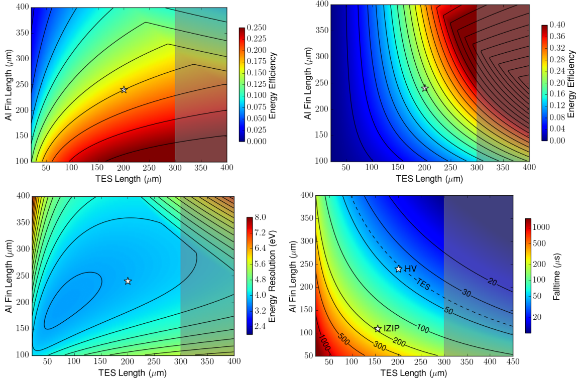
Figure 7.1: 2D optimization plots for updated CDMS HV fab specs, including reduced wire widths ( 10 \rightarrow 2 \mu\text{m} ) and reduced TES width ( 2.4 \rightarrow 0.5 \mu\text{m} ) as well as higher R_n ( 150 \rightarrow 300 \mu\text{m} ) and thicker fins at 1.2 microns. I also updated this code to take into account a modified resistivity expectation of around \rho \sim 5 * 10^{-8} \Omega\text{m} found from our test devices. Top Left: Energy Efficiency. Top Right: First-pass phonon collection efficiency. Bottom Left: Energy resolution. Bottom Right: Phonon collection time. Notice that we now have a broader space in which we can achieve the same resolution, and we could even change the existing design according to these parameters without any significant modifications aside from changing the QET number. This demonstrates that without improvements in quasiparticle collection, our only other handle is fabrication. We improve efficiency somewhat by reducing line widths, but that only allows us to make smaller QETs, not significantly improve our resolution.
