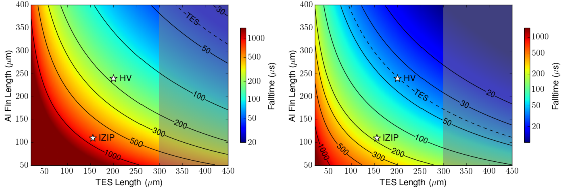
Figure 4.6: Phonon collection time as a function of TES and fin length for Ge (Si) on the left (right). The iZIP, which only has an aluminum coverage of \sim 4\% , is much slower. Si is faster than Ge due both to the faster sound speed and the better impedance match between Si and Al. The Si HV detector is expected to be fully bandwidth matched, i.e. the phonon and TES falltimes should be about the same.
