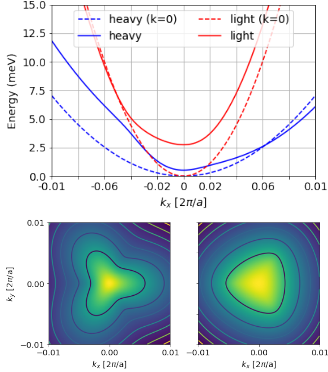
Figure 2.14: Brillouin zone for the holes rotated so that k_z is along the \langle 111 \rangle direction. Top: Dispersion relation at k_y = 0 for E(k_x = 0, k_z) = 1 meV and k_z = 0 at the band minimum. The equal energy surfaces for both the light and heavy holes as a function of crystal momentum become anisotropic for charges at non-zero drift velocity. For drifting charges, the heavy hole band will be preferentially filled by inter-band phonon emission. Bottom: Contours of constant kinetic energy for heavy (light) holes are shown on the left (right) where the center of the pattern shows contours for carrier energy of \sim 3 meV for the heavy holes and the mean energy of the contours is \sim 10 meV, comparable to the mean hole energy for low electric field strength. The upper plot is a cutline through the lower plots for k_y = 0 . Reproduced from Ref [74].
