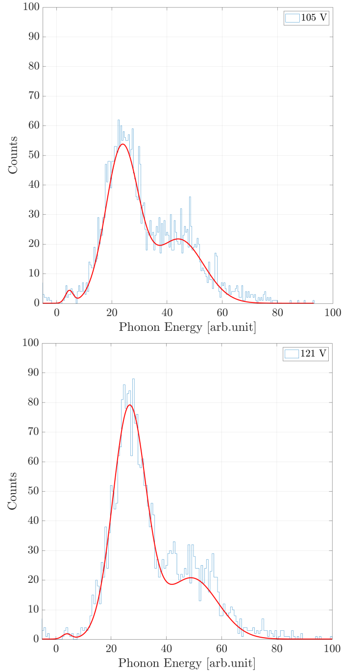
Figure 5.27: Energy spectra from HVeV detector for bias voltages 105 and 121 V (see text for more details).
