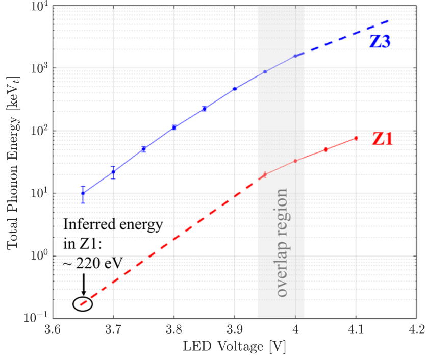
Figure 5.15: Total phonon energy as a function of LED bias voltage for detectors Z1 and Z3 while operated at 0 V.
