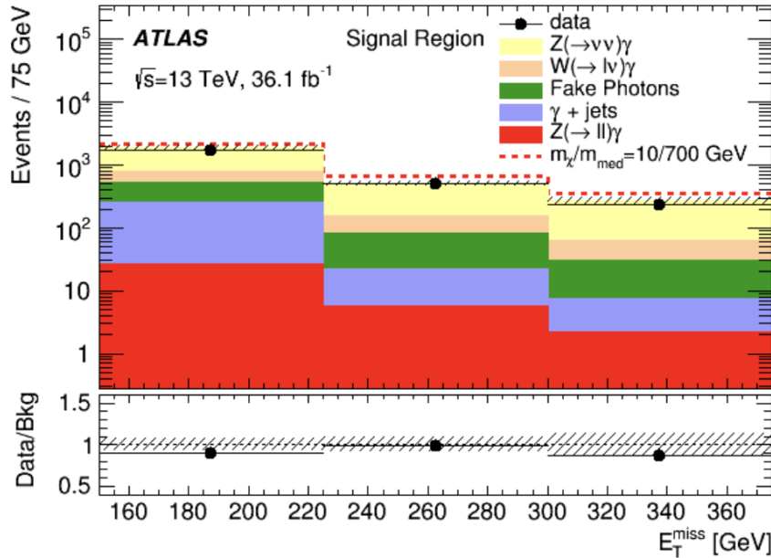
Figure 1.14: Red dashed line shows an example of WIMP scenario in a transverse missing momentum distribution. Image source: [49]
