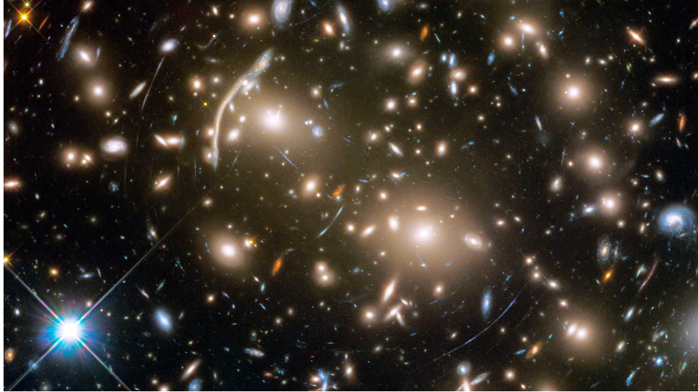
Figure 1.3: The effect of gravitational lensing of galaxy Abell 370. The blue-ish arcs are the distorted light from galaxies far behind the cluster. Image source: NASA, ESA, J. Lotz and the HFF Team/STScI.
