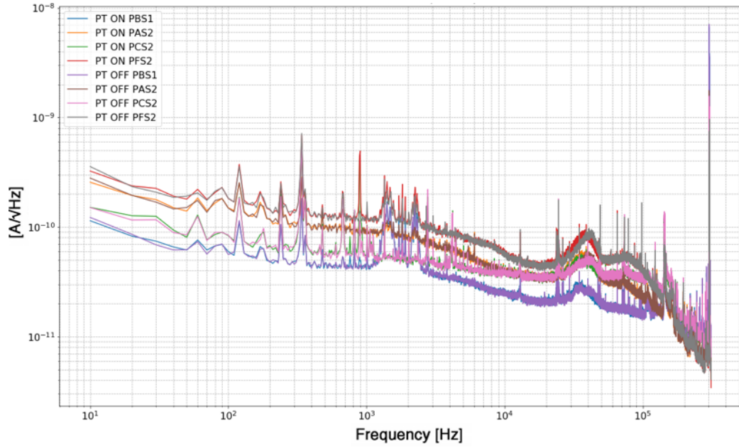
Figure 4.33: Transition noise PSD for detector T5Z2 when turning the PT on and off. The sensor name shown in the legend follows the following name convention: “Phonon” + “Sensor Name” + “Detector Side Number”, i.e. “P” + “B” + “S1”.
