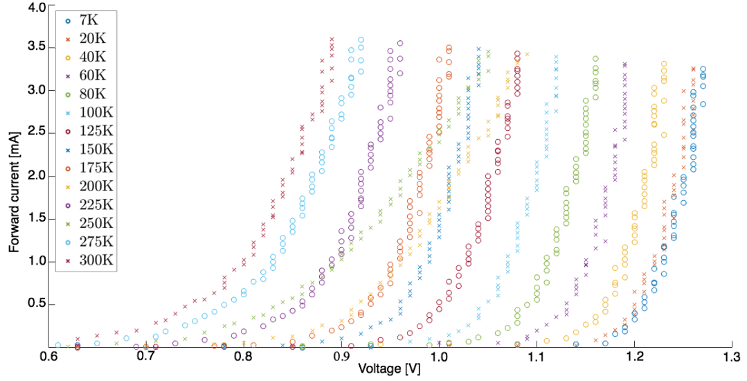
Figure B.1: IV curve for the 1200 nm LED as a function of temperature. See section 5.2.8 for more details.
