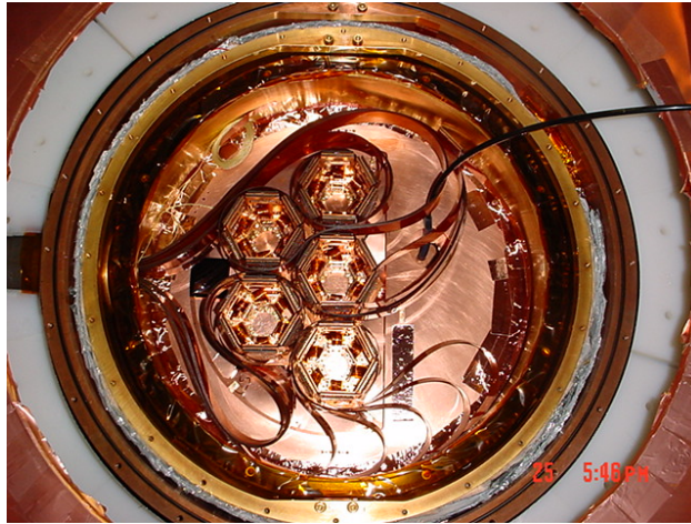
Figure 4.9: Final configuration of the Soudan icebox before the 5-Tower runs, showing the SQUETs and striplines atop the 4K lid. The E-stem and warm electronics lie to the left of the photo, while the dilution refrigerator lies to the right.
