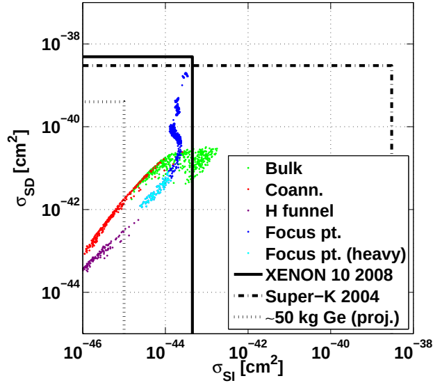
Figure 2.20: Comparison of spin-independent and spin-dependent WIMP interaction cross sections and experimental sensitivities. Colored points represent a selection of CMSSM models from the regions described in the text, following the color conventions of Figure 2.19. Lines represent approximate minimum upper limits on spin-independent and spin-dependent WIMP-nucleon scattering cross sections from various leading experiments, under the assumption that a_p \approx a_n . Boxes represent recent results from a leading direct search (XENON 10 [158, 159]), a leading indirect neutrino search (Super-K [125]), and the projected reach of a hypothetical large Ge detector.
