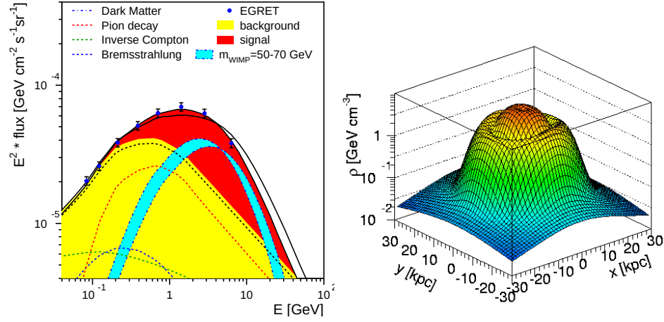
Figure 2.8: (a) Illustration of the proposed EGRET gamma ray excess (red), including the contribution from a \sim 60 \text{ GeV}/c^2 neutralino model (cyan). (b) Proposed density profile of the galactic WIMP halo based upon the EGRET data. Plots taken from [114].
