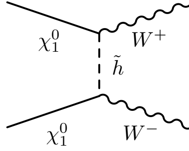
(b) Annihilation to gauge bosons, characteristic of the focus point.
