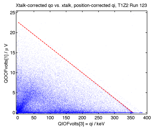
Figure 3.9: q_i and q_o amplitudes for ^{133}\text{Ba} events in T1Z2, showing events shared between the electrodes. The red line indicates q_i + q_o = 356 keV.
