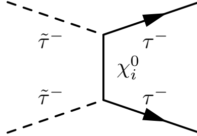
(d) A stau annihilation process relevant in the coannihilation region.
