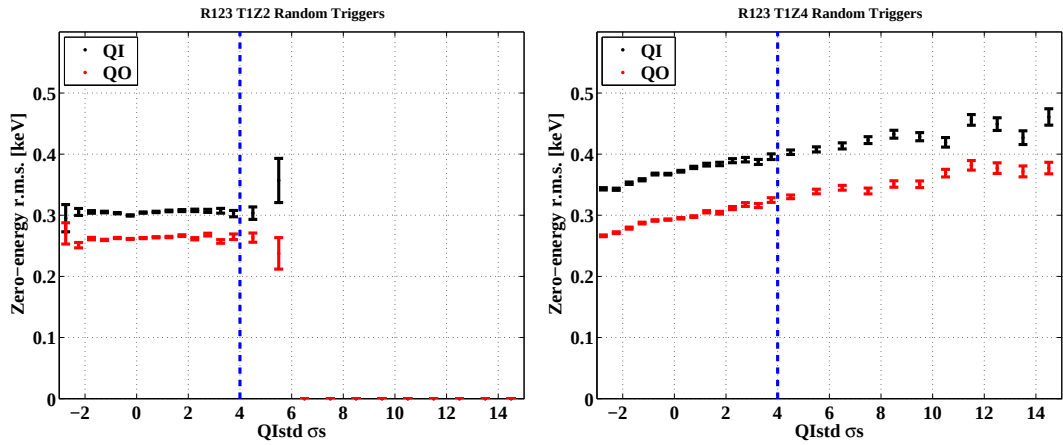
Figure 6.8: Ionization resolution (standard deviation) as a function of QIstd , measured in normalized units. The left plot shows a microphonically insensitive detector (T1Z2), the right a microphonically sensitive one (T1Z4).
