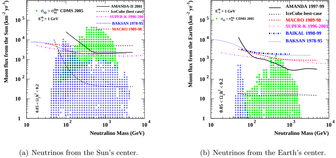
Figure 2.12: Limits and projections for indirect WIMP detection with various neutrino detectors. Colored points indicate a sample of MSSM models. Green circles are excluded by CDMS's 2005 result[3], while blue crosses are not. Plots taken from [123].
