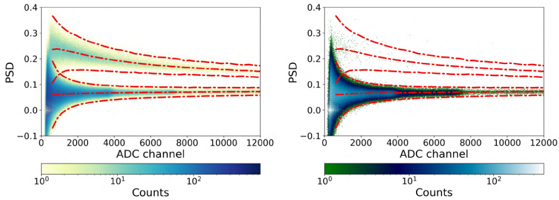
FIGURE 6.21: (left) PSD distribution for the Am-Be source showing clear separation between neutron and gamma events. Events within the mean \pm 3\sigma region are identified used for further analysis. Adapted from Ref. [11]. (right) PSD distribution for background data, demonstrating negligible leakage of ambient gamma events into the neutron band. The misidentified fraction is \sim 0.17\% relative to the Am-Be neutron event rate, indicating a negligible impact on the analysis.
