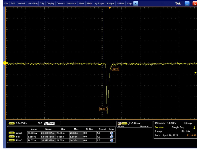
FIGURE 6.20: Example of a raw pulse recorded using an oscilloscope for an Am-Be source.
