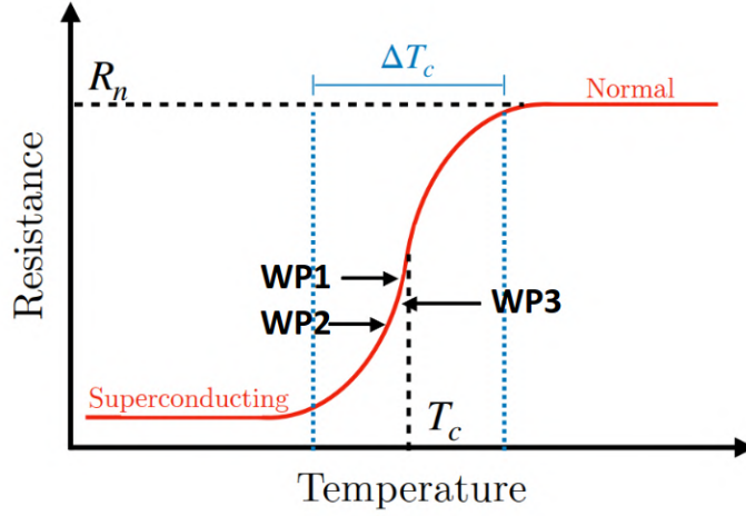
FIGURE 3.9: Schematic representation of the three working points (WP1, WP2, and WP3) selected along the TES resistance–temperature (R–T) transition curve during LED data collection. The working points are defined by different applied QET bias currents. Increasing the QET bias current shifts the operating point upward in the transition curve and reduces the effective current gain of the detector response.
