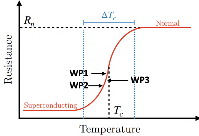
FIGURE 3.34: Illustration of different working points (WPs) along the superconducting R–T transition curve. Points lower on the transition correspond to a higher current scale (i.e., a larger first e^-h^+ peak position in current units). WP2 corresponds to the highest current scale, WP3 to an intermediate current scale, and WP1 to the lowest current scale.
