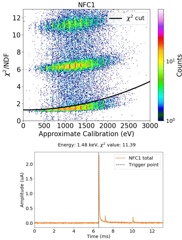
FIGURE 3.29: (top) Reduced \chi^2 from the frequency-domain OFL fit as a function of reconstructed energy for the high-voltage LED calibration series in the NFC1 detector. High- \chi^2 /n.d.f. populations are dominated by pile-up events. (bottom) Example of events rejected by the \chi^2 selection.
