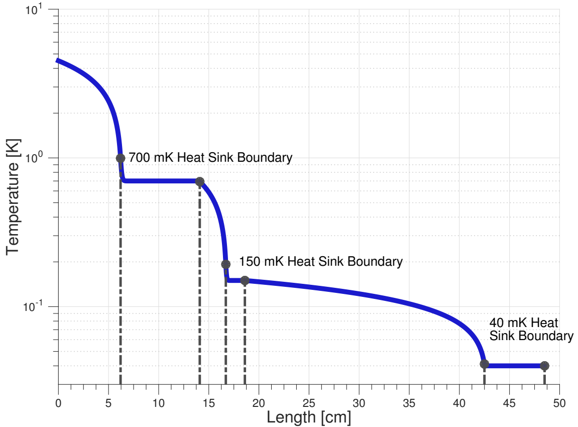
Figure 7.33: The temperature profile of the vertical phonon cable including the effect heat sinking but not the effect of added electronic component heat dissipation. The heatsinks include the total thermal resistance plotted in Figure 7.32. Length = 0 cm is the cryocooler stage of the tower whose temperature is estimated to be around 4.5 K due to the low altitude of the SNOLAB facility. The cable extends considerably beyond the 40 mK heat sink to reach the detector, but we truncate to plot at this heat sink. This plot assumes a 0.06 inch thick cirlex stiffener is located between the cable and heat sink attachment surface, which represents the worst case heat sinking efficiency. Even in this scenario, the cable is rapidly brought to the heat sink temperature.
