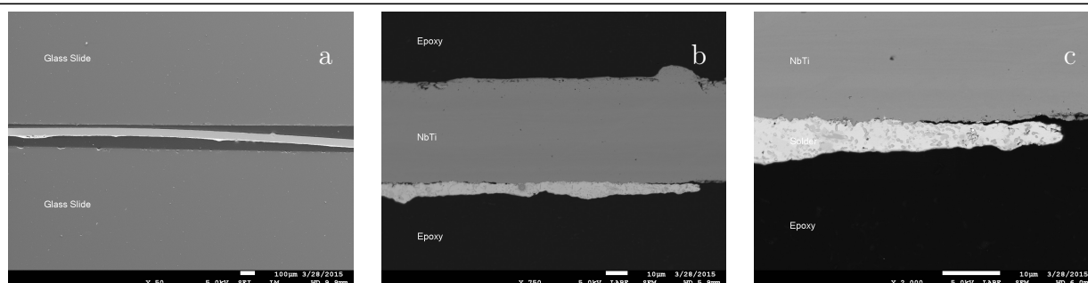
Figure 7.28: SEM micrographs of activated solder on Nb-47Ti foil. The solder was applied using and ultrasonic soldering iron only to the bottom side of the foil, which is approximately 0.003 inch thick.
