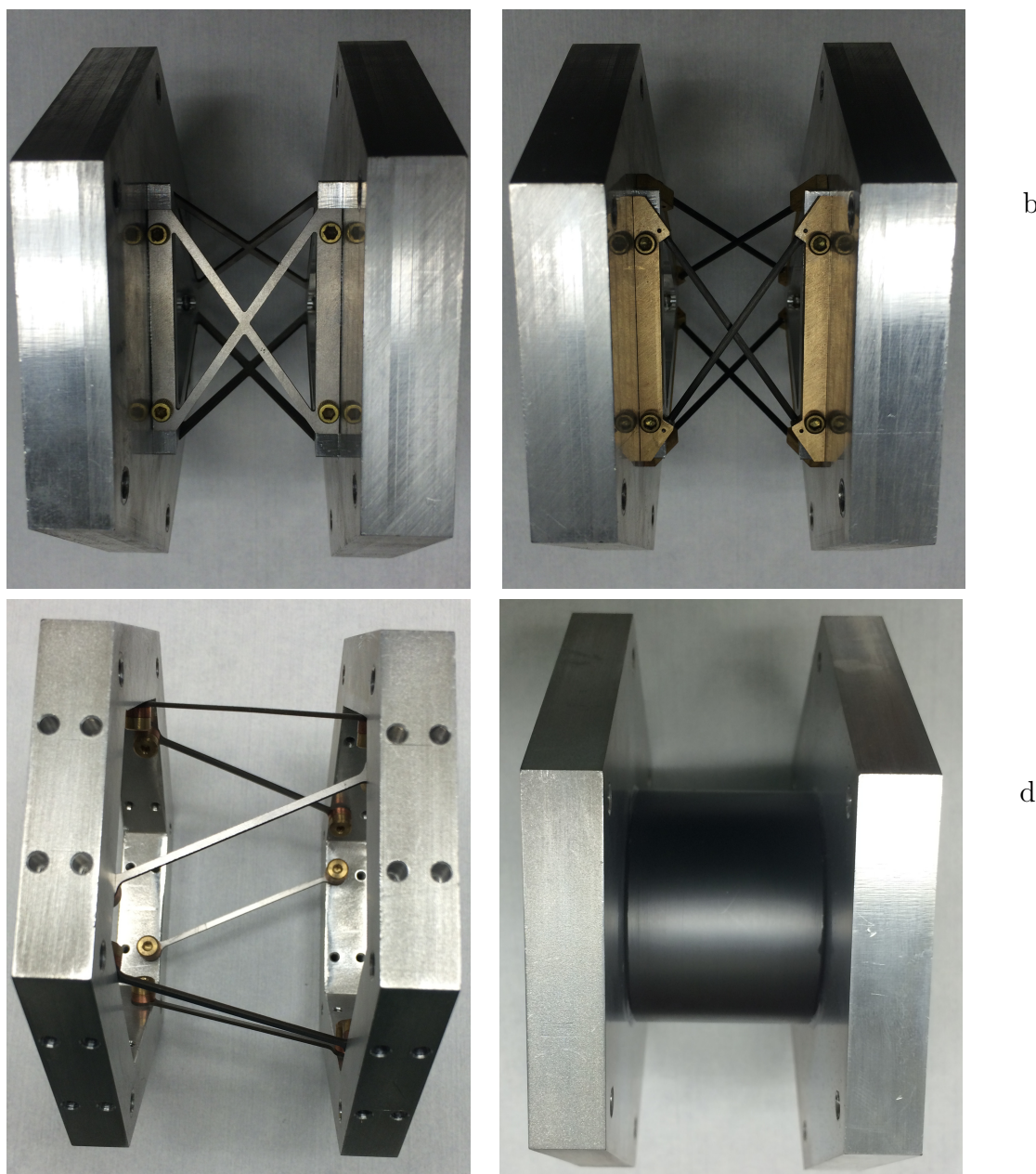
Figure 7.11: Tower standoff test modules. Strength and stiffness measurements of the standoff structures considered were done when the standoff structures installed in aluminum adaptor flanges. The assembly of the structures installed in the flanges are what we call test modules. the orientation positioning of the standoff structures are exactly as it would be if the structures were installed on towers. View a is a Ti 15-3-3-3 X-frame; b is a graphlite X-frame; c is a Ti 15-3-3-3 hexipod; and d is graphite tube. The rods in b have about 0.018 inch of clearance at the crossing point.
