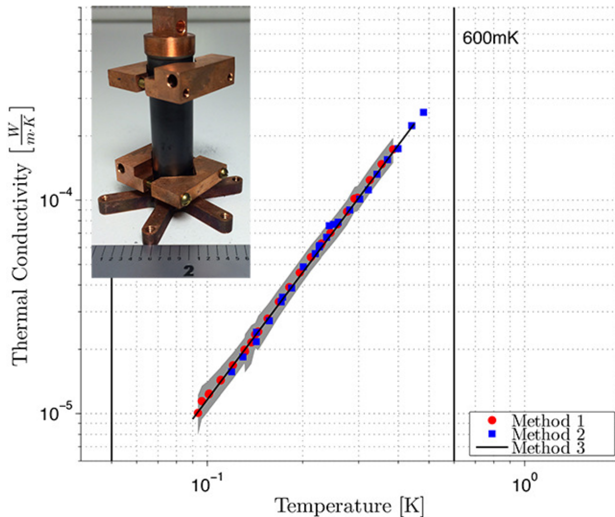
Figure C.7: VespeL SCP-5050 thermal conductivity.
