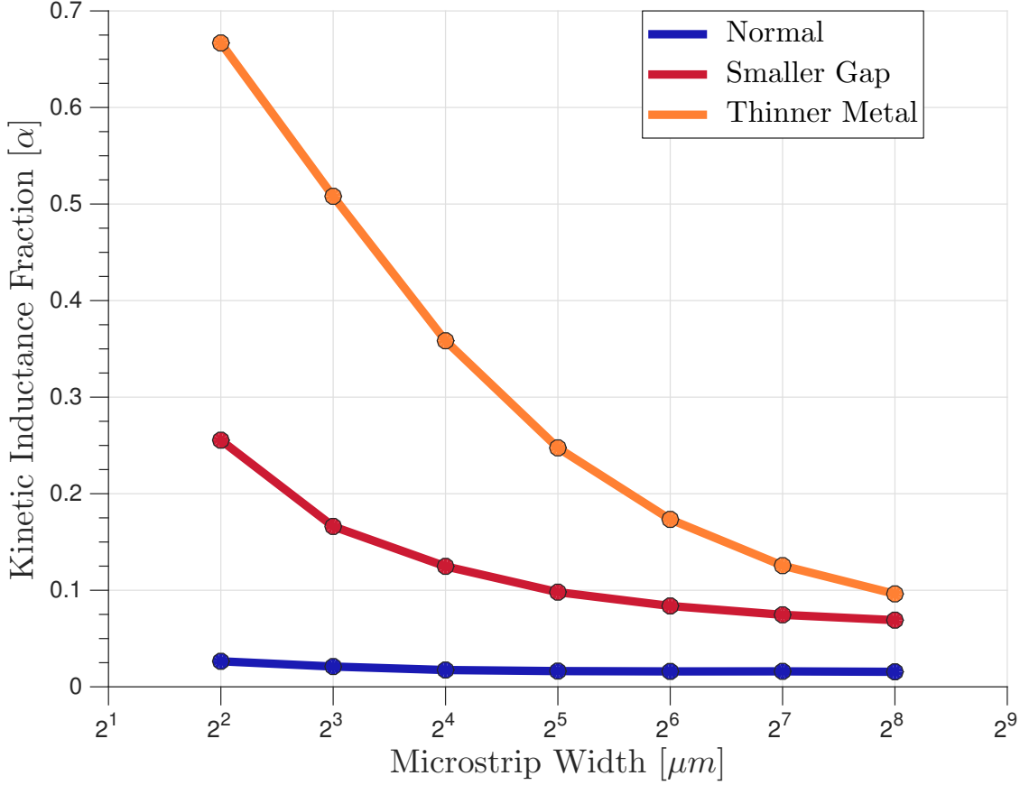
Figure 5.3: We use the procedure described in § 5.3 to calculate the kinetic inductance fractions for the sensor chips on the current test mask under two hypothetical conditions. One – the microstrip gap is held at its true value and the thicknesses of the conductors are reduced by a factor of ten. Two – the microstrip gap is reduced by a factor of ten and the thicknesses of the conductors are held at their true values.
