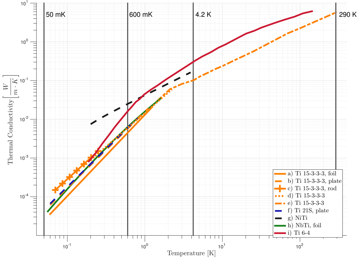
Figure 7.6: Thermal conductivity of selected titanium alloys. Data source, additional sample information and the direction of heat flow (when known) are as follows : a) original data [6, 97], || to face of foil sample;; b) original data [6], || to face of plate sample; c) original data [6], || parallel to the axis of rod sample, annealed condition, sourced from China; d) unpublished data from Runyan and collaborators, annealed ingot manufactured in and sourced from China; e) from Tuttle et al. [183], sample was wire EDM cut from a 1.6 mm thick plate of TIMET manufactured material; f) original data [6], || to plate; g) original data [7], || to foil, and h) from Woofcraft et al. [200]
