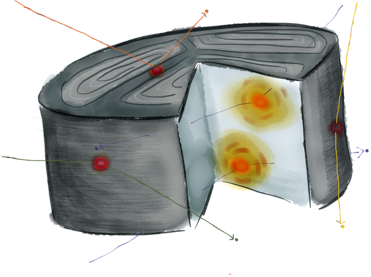
Figure 2.8: Illustration of the particle interactions in the CDMS detector. WIMPs (purple particles and tracks) are expected to interact anywhere within the detector volume. Most other particles, such as muons and phonons, have a greater chance of interacting close to the surface of the detector due to their higher electromagnetic and weak interaction cross sections with standard model particles. A fiducial volume of the detector excludes the surface region where interactions will most likely be due to non-WIMP particles. Event discrimination involves fiducial volume cut to eliminate event outside that volume, as well as a general comparison of the phonon to charge signal strength. The increased number of phonon sensors, as well as an improved sensor design will enhance background discrimination the SuperCDMS SNOLAB detectors. Image from [2].
