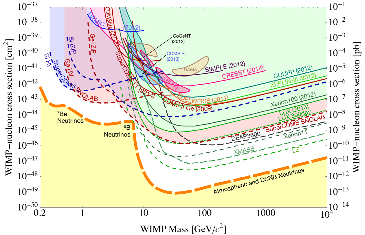
Figure 2.7: Areas of mass-cross section parameter space which lie above the curve drawn for a given experiment are excluded by that experiment's data. Closed curves indicate discover claims at different confidence levels.
