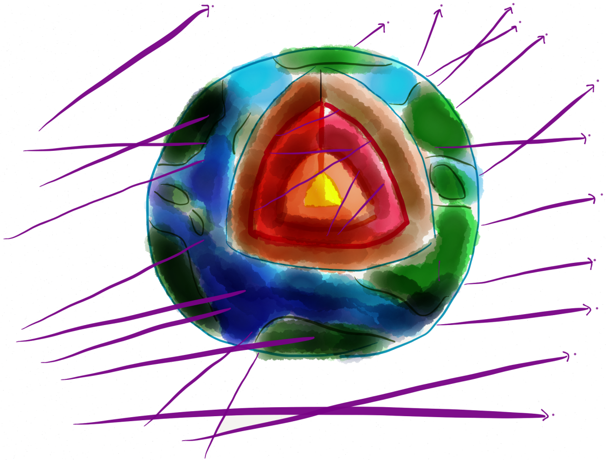
Figure 2.4: Most dark matter experiments exploit the fact that WIMPs (purple particle tracks) interact so infrequently, they can pass through the Earth unimpeded. Underground locations are chosen for these experiments so that other particles are stopped by the overburden of rock. Image from [2].
