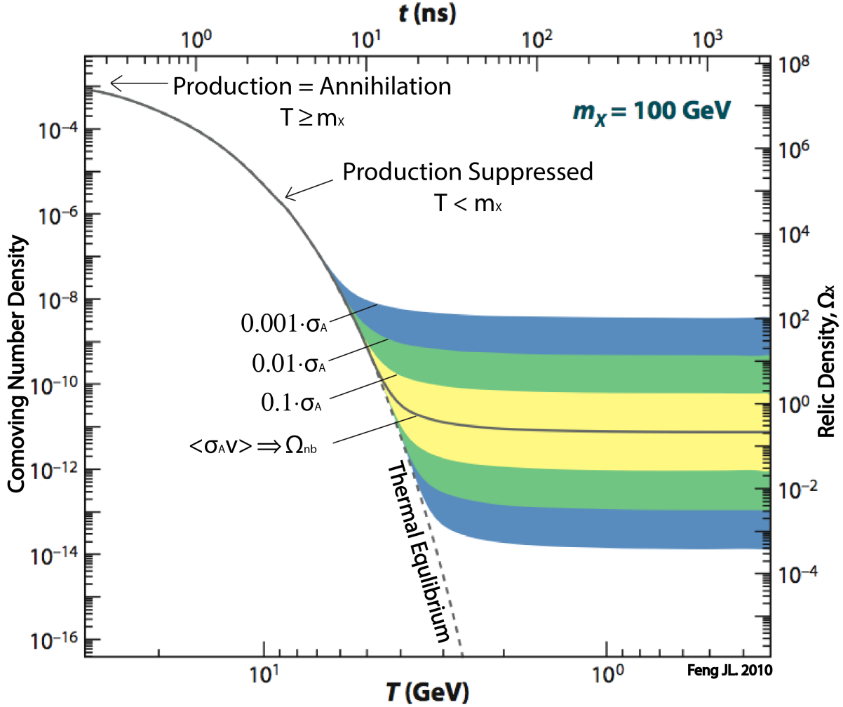
Figure 1.9: WIMP decoupling from the primordial plasma. The solution of the Boltzmann equation gives the comoving number density of the WIMP as a function of temperature or time since the big bang. As the universe cools, the WIMP number density decreases from a constant value (not visible on the plot) as annihilation is more favorable than creation, until the particle departs from thermal equilibrium with the plasma, i.e. ‘freezes out’. Freezes out would have occurred when the expansion rate of the universe surpassed the WIMP annihilation rate. The final value of the number density is determined by \langle\sigma_A v\rangle . Assuming a WIMP mass of 100 GeV, the dark line used the value of \langle\sigma_A v\rangle which yields the correct relic density. The colors separate the relic densities obtained fact of ten changes in \sigma_A . Modified image from [65]
