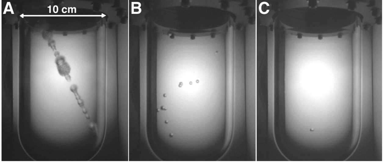
Figure 2.6: Nucleation of bubbles in the COUP experiment. Left, a cosmic ray event. Middle, A neutron multiple scatter event. Right, A neutron single scatter. Image from [28].
