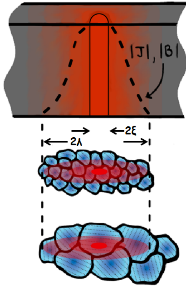
Figure 3.4: We illustrate three scenarios for bulk vortex penetration. On top, a vortex is inside of a thick conductor. The normal metal core of an Abrikosov vortex is about two times the coherence length in diameter. The decay from its critical value at the core of the current density is set by the penetration depth. The situation where the vortex core is much larger than, or about the same size as the grains is illustrated in the center and bottom views, respectively. Illustration from [3]
