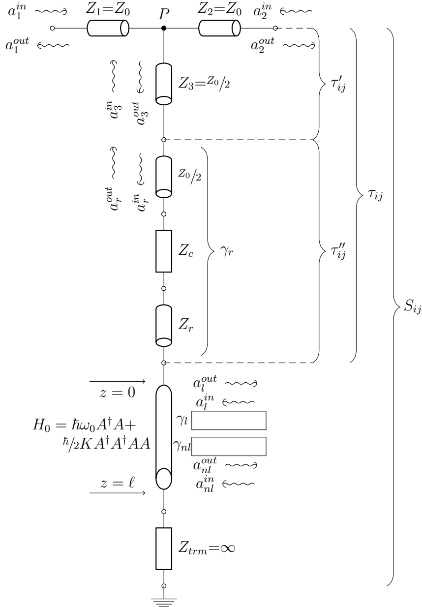
Figure 4.5: Network diagram of nonlinear \lambda/2 resonator shunt-coupled to feedline. The coupler \tau_{ij} , is composed of a three-port junction of three transmission lines, \tau'_{ij} , and a two-port coupling to the nonlinear resonator, \tau''_{ij} . A is the resonator mode and the resonator Hamiltonian includes a non-dissipative Kerr nonlinearity, K . The resonator is coupled to bath modes a_r , a_l and a_{nl} via coupling constants \gamma_r , \gamma_l and \gamma_{nl} allowing exchange of resonator energy with the pump/detector, linear losses, and nonlinear (two-photon) losses, respectively. Z_{trm} is the resonator termination. The a_r are the same as the a_3 except that their directions are reversed. S ports one and two are the same as \tau ports one and two. \tau' port three is \tau'' port 1 and \tau'' port 2 is \tau port 3.
