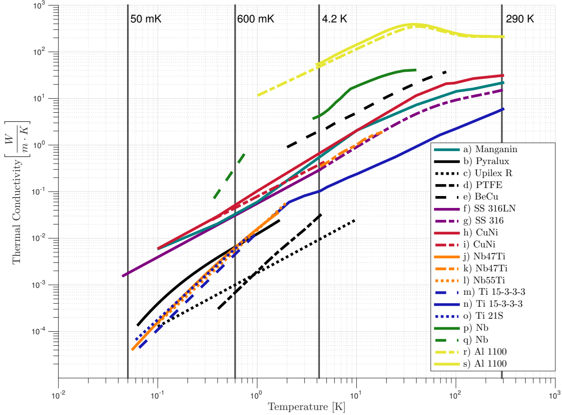
Figure 7.15: Thermal conductivities of materials useful for low temperature flexible circuits and cables. Data sources are : a) from Blake [32]; b) original data [7], || to sheet; c) from Barucci et al. [25], || to sheet; d) from Kushino et al. [107], || axis of tubular sample; e) from Berman [31], alloy containing 2 wt% beryllium was held at 300 °C for 2 h and the resulting hardness was 41 Rockwell units and the electrical resistivity was 8.25 \cdot 10^{-6} \Omega \text{ cm} at room temp, 6.2 \cdot 10^{-6} \Omega \text{ cm} at 77 K, and 5.5 \cdot 10^{-6} \Omega \text{ cm} at 4.2 K; f) from Barucci et al. [26], Stainless steel 316LN is an austenitic SS with 18 wt% Cr and 8 wt% Ni and the addition of 2-3 wt% of molybdenum assures good corrosion resistance; g) from NIST, [11]; h) from Blake [32]; i) from Kushino et al. [107], || axis of tubular sample; j) original data [7], || to foil; k) from Dyachkov et al. [59], wire sample; l) from Olson et al. [141], wire sample; m) original data [6, 97], || to foil face; n) from Tuttle et al. [183], sample was wire EDM cut from a 1.6 mm thick plate of TIMET manufactured material; o) original data [6], || to plate; p) from Reiche et al. [156]; q) from Mendelssohn et al. [131], polycrystalline rod of Johnson Matthey material (JM 4526) of 99.99% purity; r) from Woodcraft et al. [198], commercially pure wrought aluminum 99 wt% minimum, and s) from NIST, [11]
