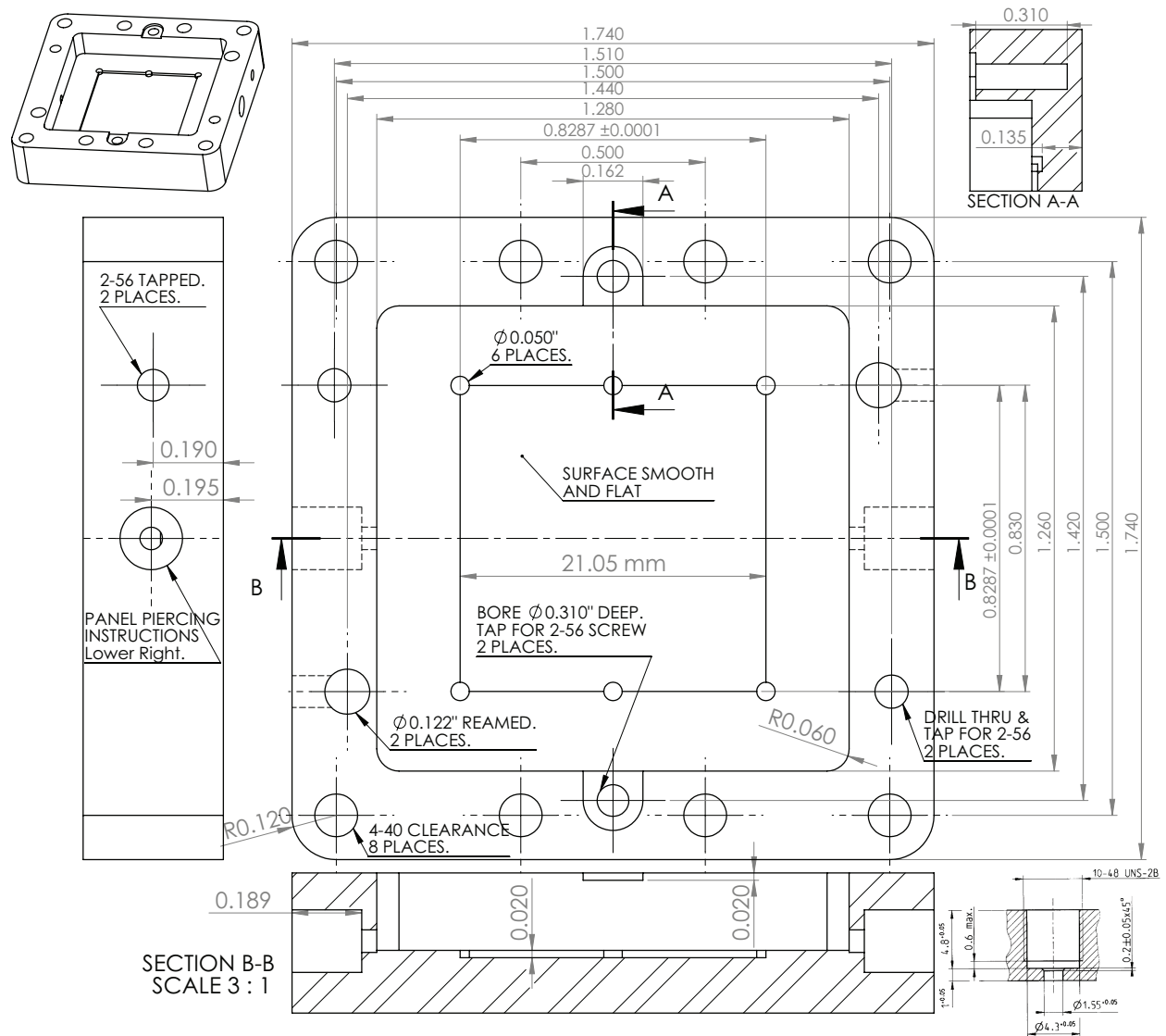
Figure D.4: KIDs test box bottom fabrication drawing. Dimensions are in inches except for the panel piercing instructions in the lower right, which are in millimeters. These instructions are taken from Rosenberger drawing MB_227A and are for their bulkhead SMP plug limited detent 19S105-500L5 connector.
