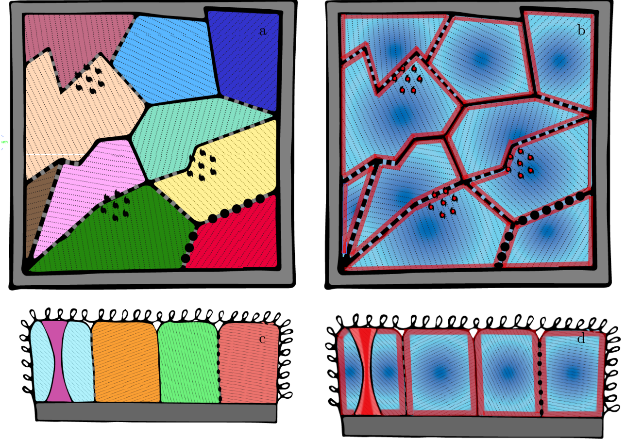
Figure 3.3: Visualization of superconducting grains, their linkages, two-level systems, and how current and vortices interact with them. A superconductor with grains much larger than the penetration depth (i.e. vortex diameter much smaller than grain size) is illustrated. Top views a and b , emphasize the interconnections between grains. Dashed grain boundaries denote the weak lines; dotted grain boundaries denote impurity contamination, e.g. hydrocarbon contamination. b – larger penetration depths near the grain boundaries result in higher current densities there; vortices may exist in the grains or tunnel through the grain boundaries. Cross section views c and d , show two-level systems distributed across the surface of the film and the funnel-shaped profile of a vortex. Illustration inspiration from [82], which discusses the coupled grain model. [3]
