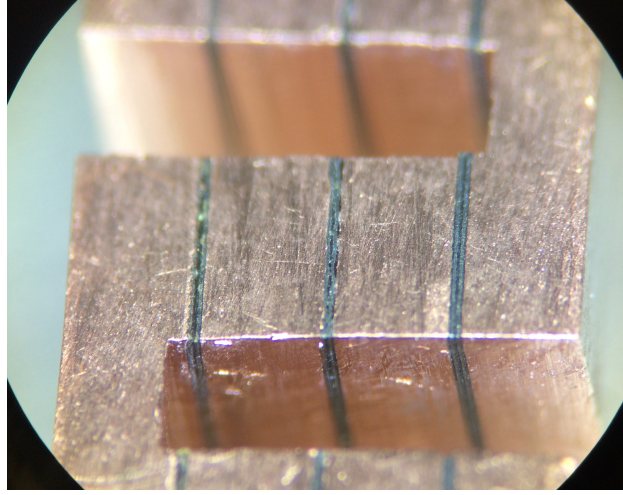
Figure 7.31: A view of a rung on the thermal resistance test device under 20x magnification. Layers appear to be reasonably well separated even after the trauma of milling the slots.
