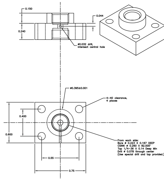
Figure D.10: Coaxial vacuum passthrough fabrication drawing. Dimensions are in inches. Design is from Dr. Peter Day at the NASA Jet Propulsion Laboratory. Material is brass.
