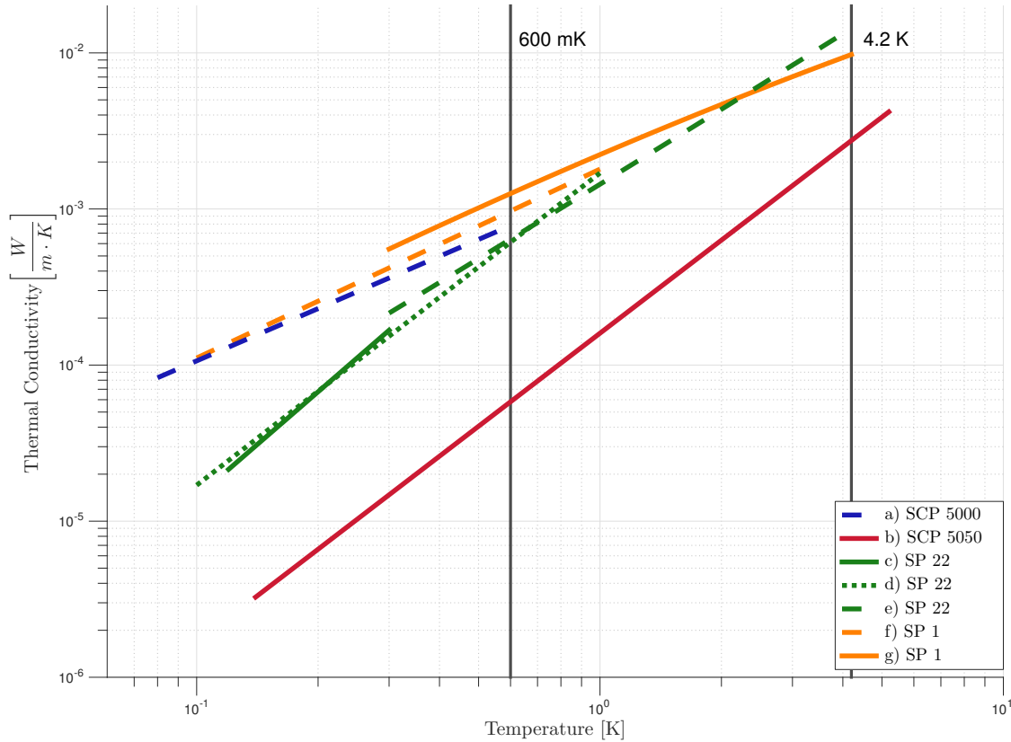
Figure 7.5: Thermal conductivity of vespel-like materials. Vespel is a bulk solid form of polyimide polymer made by DuPont. Data source, additional sample information and the direction of heat flow (when known) are as follows : a) original data [6, 97], || parallel to the axis of rod sample, unfilled polymer; b) original data [6, 97], || parallel to the axis of rod sample, proprietary filler composition; c) original data [6, 97], || parallel to the axis of rod sample, 40 wt% graphite filler; d) data from Locatelli et al. [116], 40 wt% graphite filler; e) from Runyan et al. [162], || parallel to the axis of rod sample, 40 wt% graphite filler; f) data from Locatelli et al. [116], base polyimide resin, and g) from Runyan et al. [162], || parallel to the axis of rod sample, base polyimide resin
