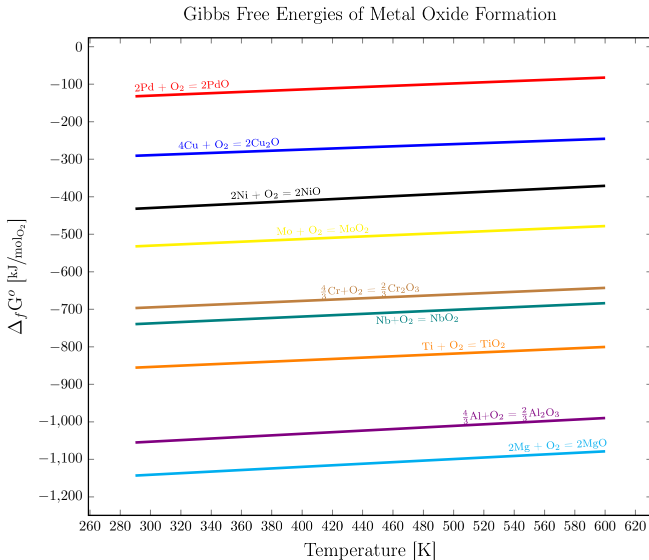
Figure 7.17: Gibbs free energies of metal oxide formation in kilojoule per mole of oxygen. Plot quantifies how energetically favorable it is for various metals to form oxides at a given temperature and at room pressure. Metals may also form oxides that are not present on this plot. This plot is also known as a Ellingham diagram.
