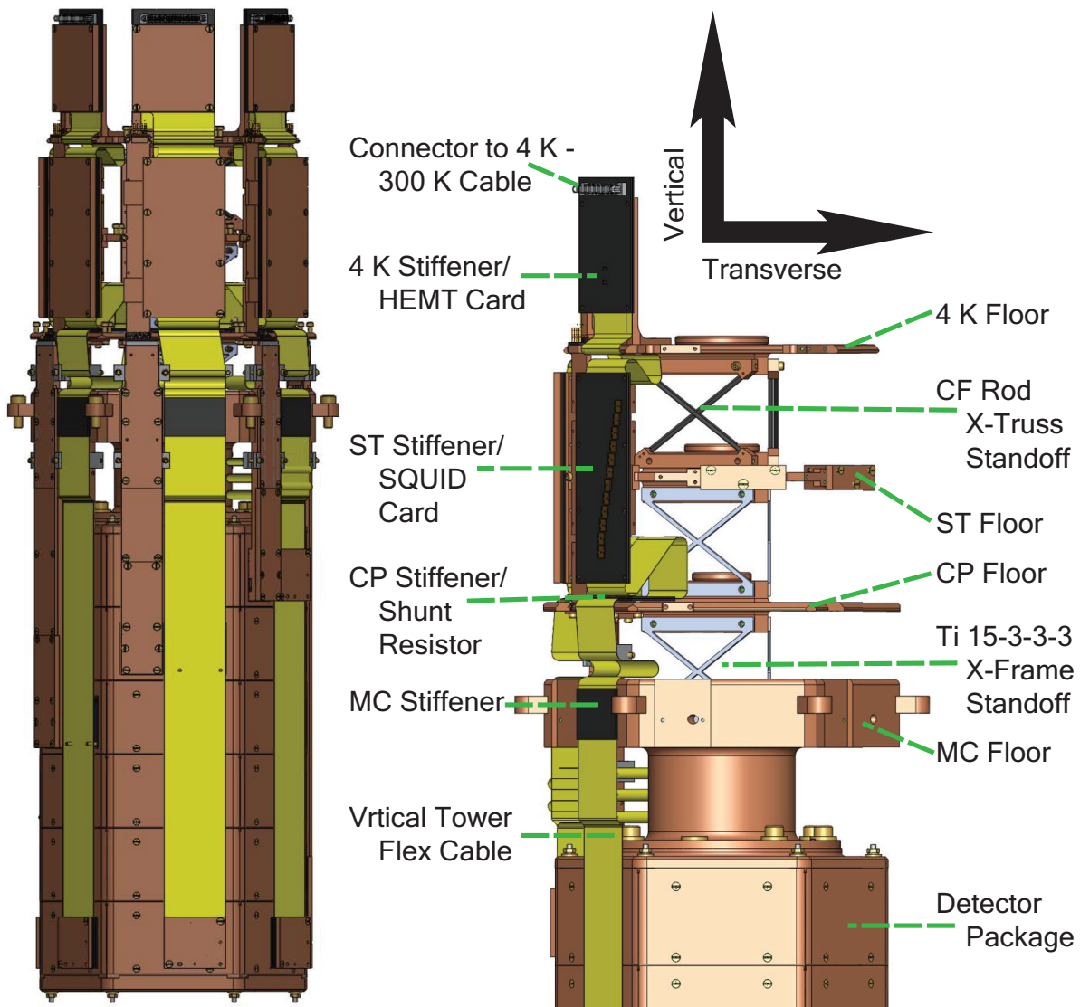
Figure 7.1: The conceptual design of the SuperCDMS SNOLAB tower. On the left, we have the full tower and detector stack assembly. Each tower holds six detectors, which are enclosed on housing packages. One notices the vertical tower flex cables which carry the signaling wires for the phonon channel, LEDs for detector neutralization, thermometry, and several charge channel bias wires. The gate wires which carry the charge signals are routed from the detectors to the HEMT Card through two (upper and lower) vacuum coaxes which can be seen running parallel to the flex cable. On the right, we zoom on on the tower, after removing four of the six phonon and charge cabling. The stiffened sections of the phonon cable are revealed by removing their copper coverings. One see that cold plate (CP) stiffener lies flat on the cold plat floor, making it difficult to see. Carbon fiber (CF) and Ti 15-3-3-3 X-frame standoffs separate the tower floors, which are abbreviated as ST – still, and MC – mixing chamber. The tower’s axial and transverse directions are indicated.
