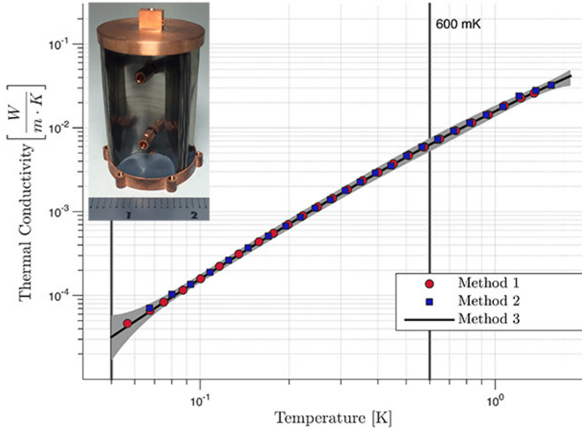
Figure C.14: Nb-47Ti foil thermal conductivity.
