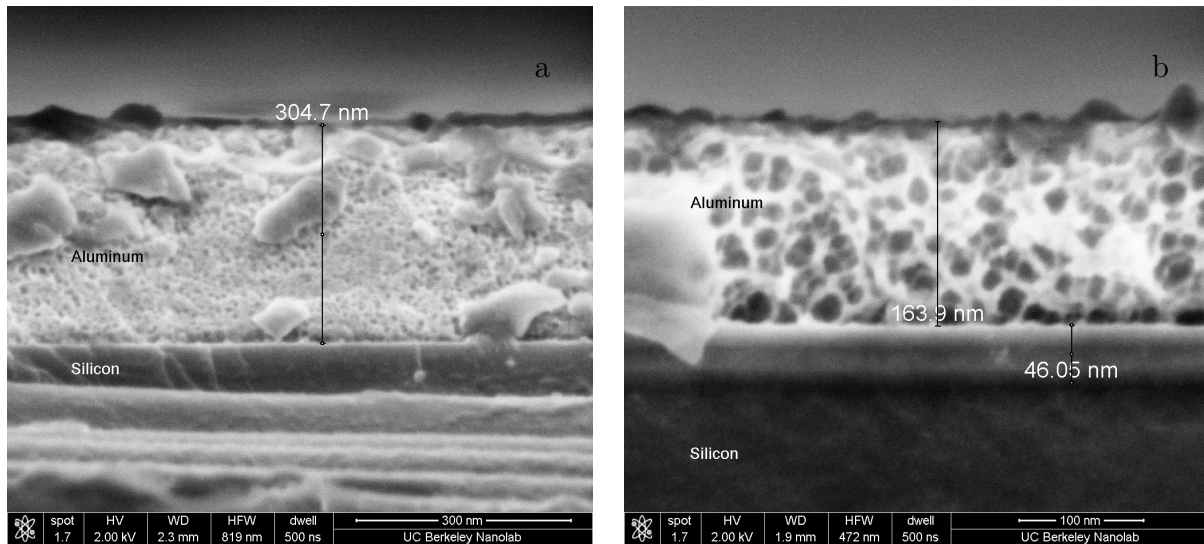
Figure 5.5: Scanning electron microscope views the saw cut surface of aluminum on silicon wafer ground planes. (a) – ground plane DSAT5. (b) – ground plane DSAT6, not used in the KIDs data presented. One notices a 46 nm interface layer perhaps suggesting diffusion processes contribute to the pores.
