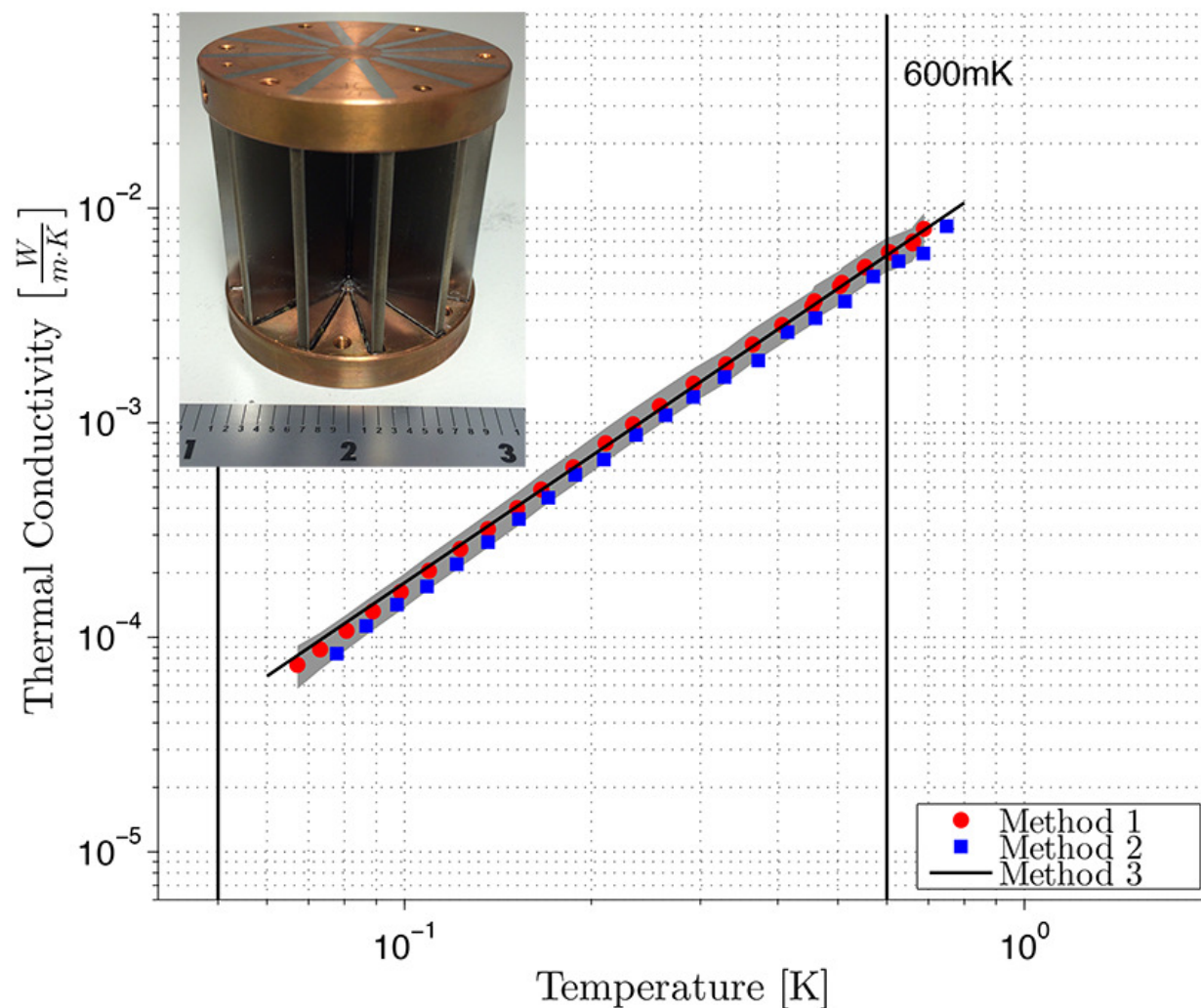
Figure C.13: Ti 21S plate thermal conductivity
