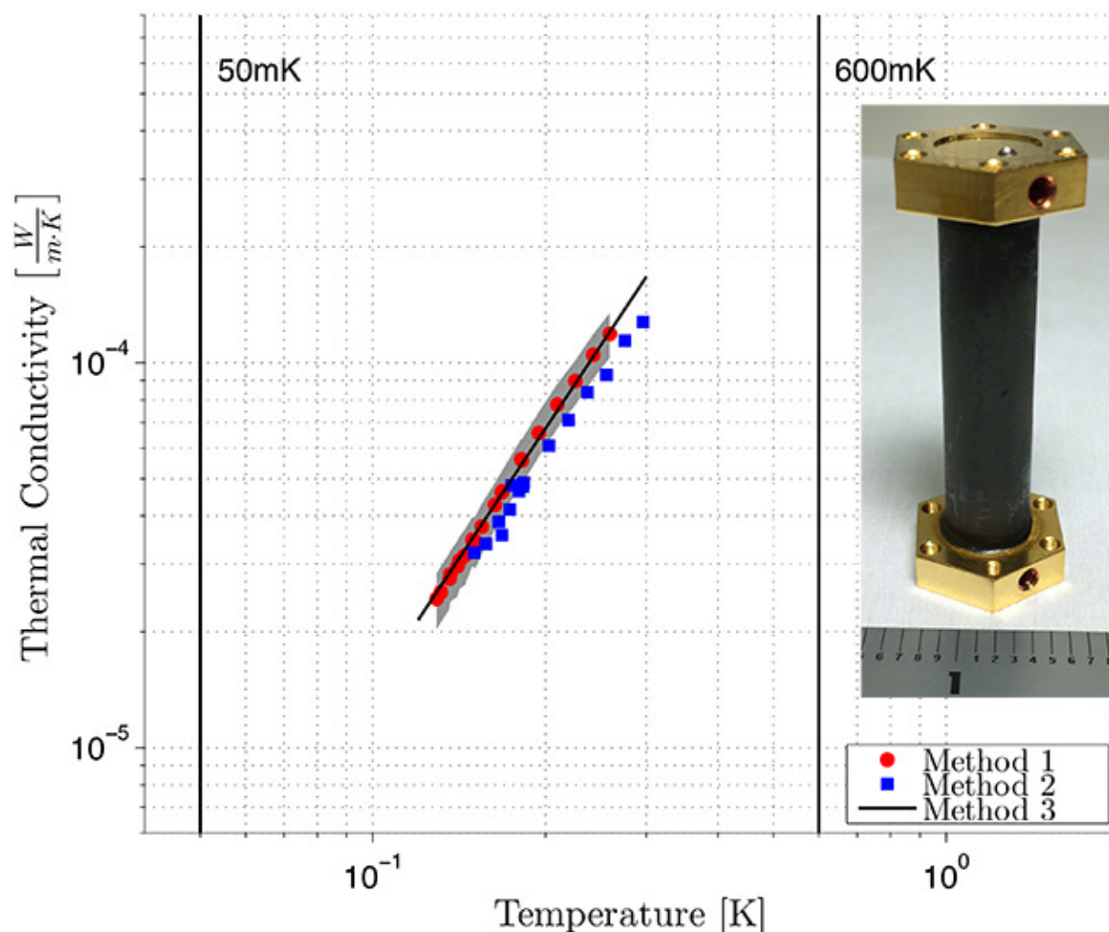
Figure C.5: Vespel SP-22 thermal conductivity.
