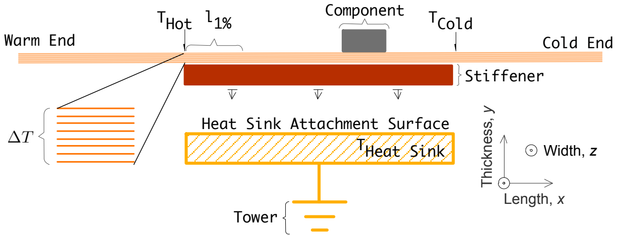
Figure 7.29: A diagram of a heat sink section of the vertical phonon cable. The base of the heatsink, the stiffener, attaches to the heat sink attachment surface of the tower. In addition to the heat coming from the warm end, power dissipation from electrical components (e.g. HEMTs, SQUIDs, shunt resistors) also add to the heat load.
