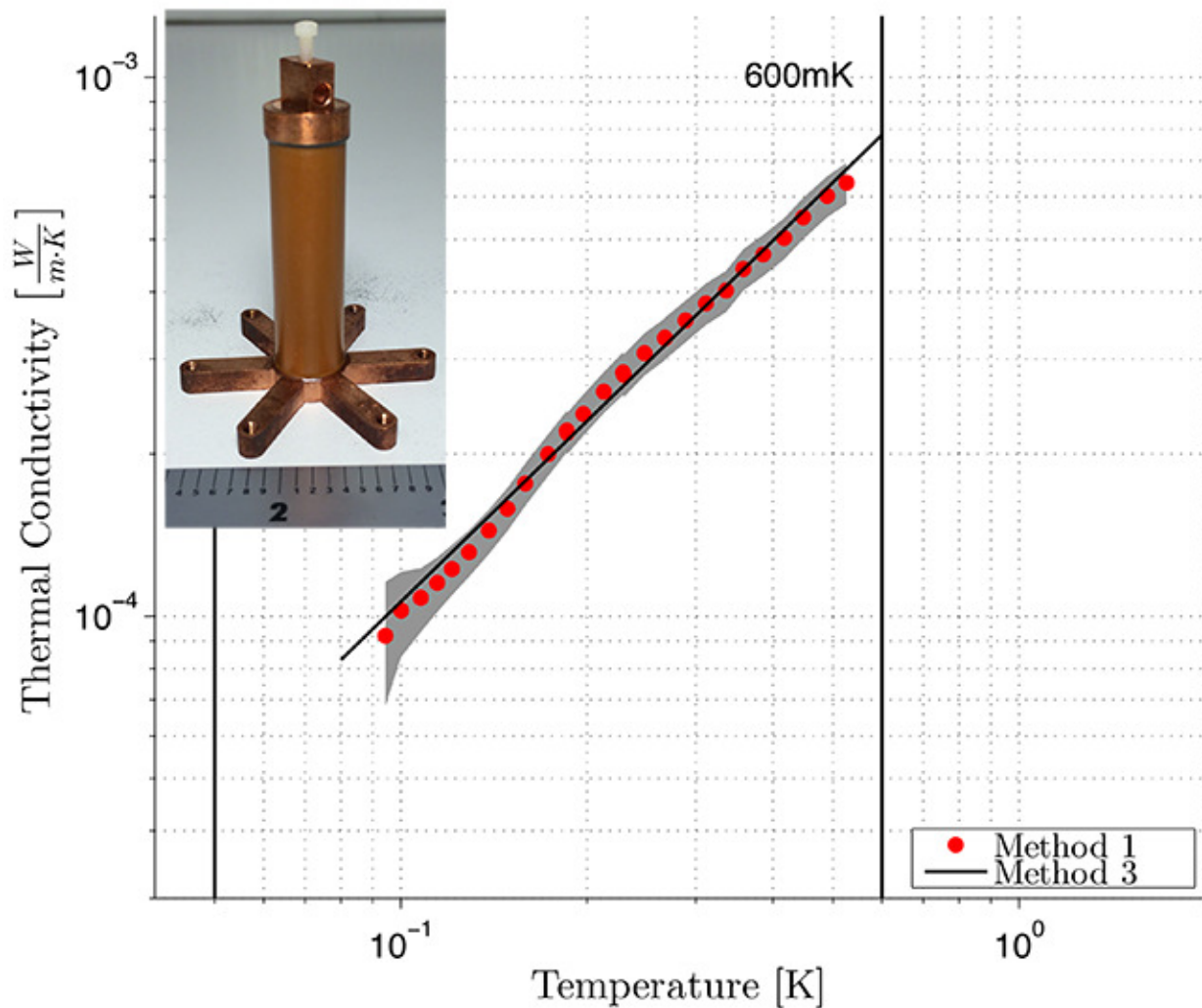
Figure C.6: VespeI SCP-5000 thermal conductivity.
