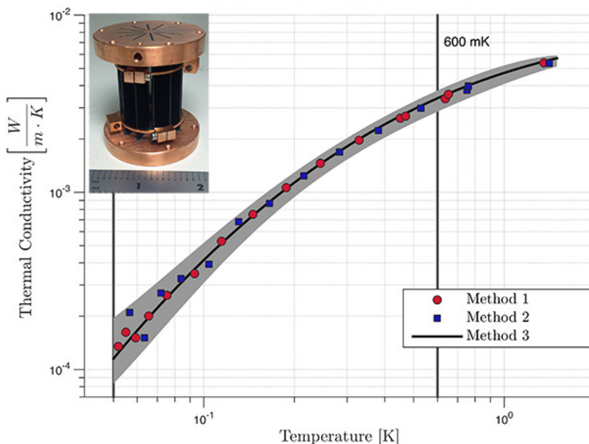
Figure C.4: Cirlex thermal conductivity
