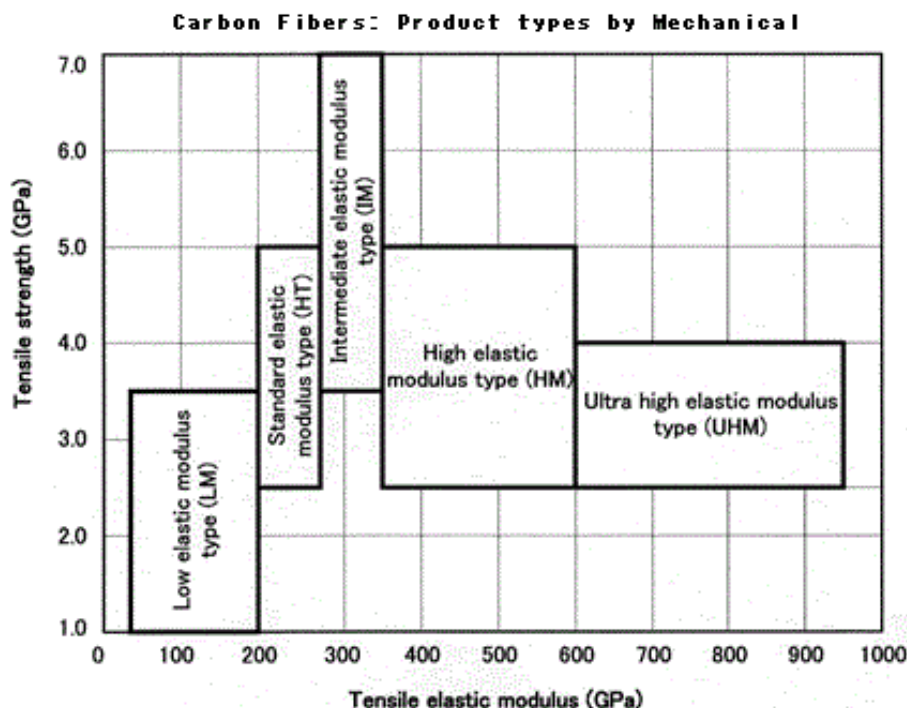
Figure 7.8: Carbon fiber can have a wide range of mechanical properties, which can be selected for the usage application. Image from [9].
