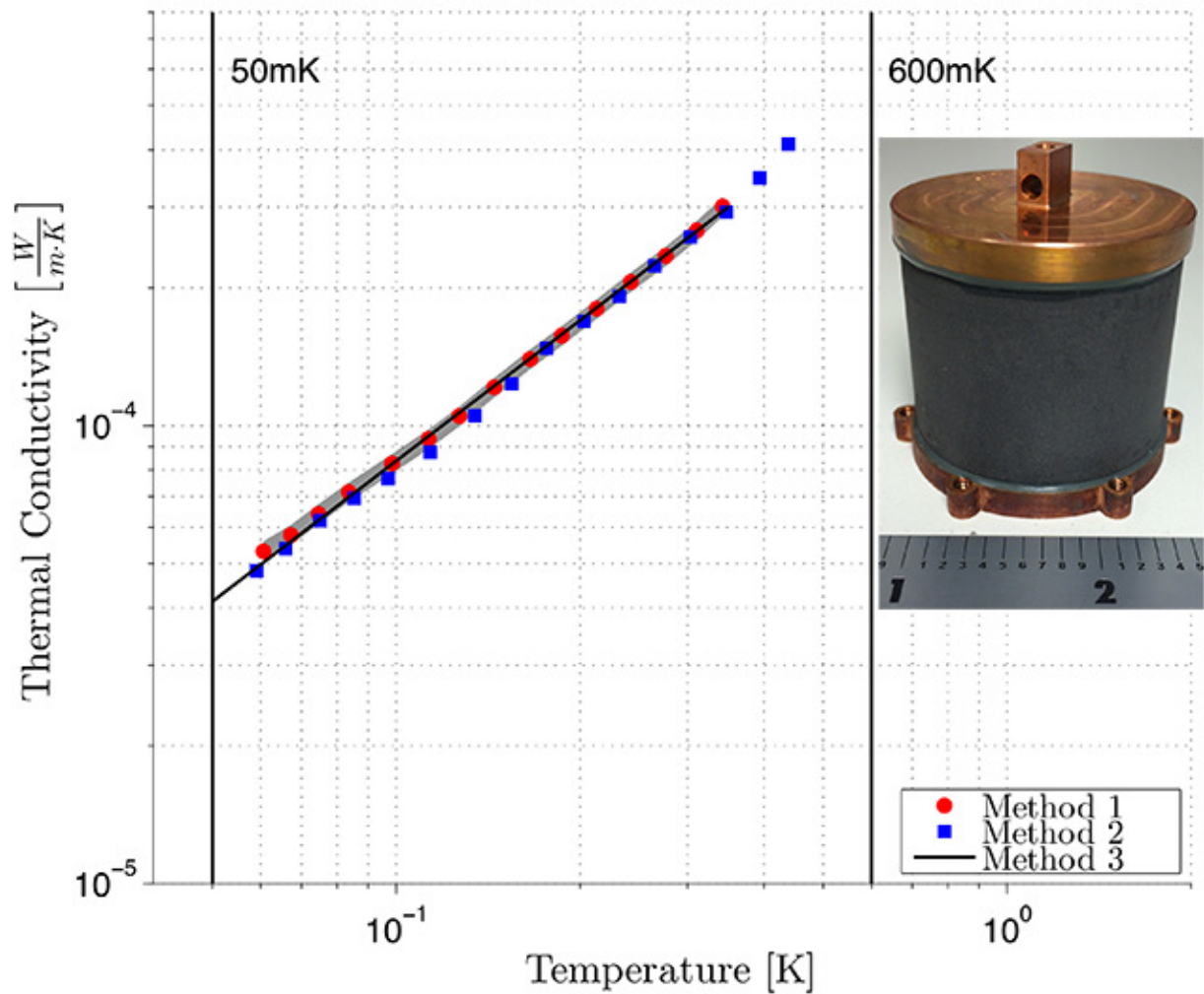
Figure C.17: Mersen 2020 Graphite thermal conductivity. Heat is directed parallel to grain.
