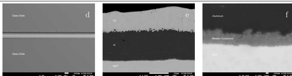
Figure 7.25: SEM micrographs of Nb-47Ti foil plated on both sides with aluminum via ion vapor deposition, and then electroplated copper. The aluminum surface was lightly etched and then zincated to promote the subsequent adhesion of copper. There should only be a few atomic layers of zinc. The bare Nb-47Ti foil is approximately 0.003 inch thick. The plated samples are epoxied between two glass slides and then the stack is polished to expose the metal layers. No heat treatment on the plated sample was used. View magnification increases from left to right with view a and d being the lowest magnification and c and f being the highest. The aluminum surface activation, zincate and copper electroplate have been performed by two different companies. The similarity in the plating microstructure between of the two companies speaks to the reproducibility of this process approach.
