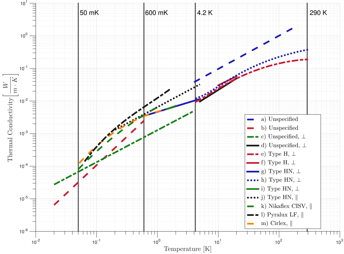
Figure 7.4: Thermal conductivity of polyimide “Kapton” laminates. Kapton is a sheet form of polyimide polymer made by Dupont. These samples are thin sheets. When indicated, \perp means that heat was made to flow perpendicular to the face of sheet (usually a stack of sheets) and \parallel means that the heat was made to flow parallel to the face of the sheet. Data sources and additional sample information (when known) are as follows : a) from Akerib [18] an unpublished CDMS internal report, unspecified kapton type; b) from Akerib [18] an unpublished CDMS internal report, unspecified kapton type; c) from Radebaugh et al. [152], unspecified kapton type; d) from Wipf et al. [197], unspecified kapton type; e) from Rule et al. [161]; f) from Yokoyama et al. [202]; g) from Lawrence et al. [110]; h) from Rule et al [161]; i) from Baudouy et al. [27]; j) from Barucci et al. [25]; k) original data [6, 97]; l) original data [7], and m) original data [7]
