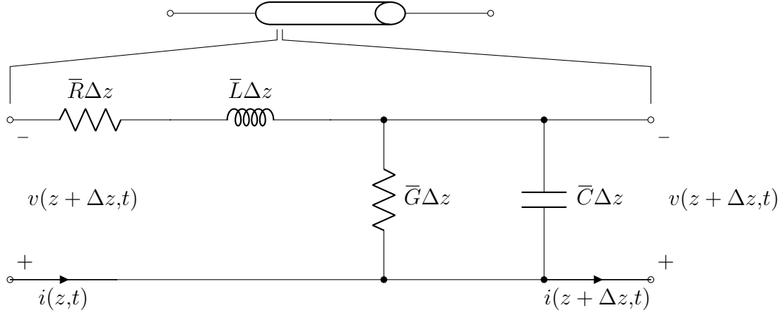
Figure 4.2: A transmission line is the series cascade of infinitesimal circuits whose elements describe the line characteristics, i.e. wave impedance and phase velocity of propagation.
