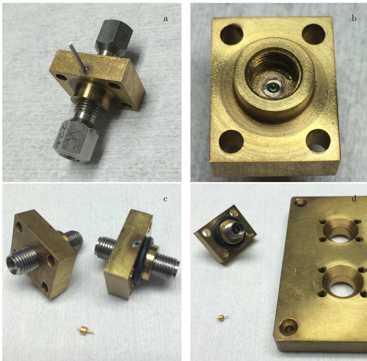
Figure D.11: Coaxial vacuum passthrough in preparation for use. (a) – positioning fixtures for the bead are screwed into place. Solder is loaded in to hole that intersects bead. The assembly is then placed on a hotplate and heated until solder melts, then quickly removed from heat. (b) – the bead is now soldered into place. (c) – SMA “spark plug” connectors are torqued to 16 inchlb. The o-ring fits over the nipple of the passthrough. A glass bead is displayed, and one can see the gold plating of its cylindrical surface, as well the the center pin. (b) – a mating flange is displayed with the passthrough. In this case, the seal is formed with a triangular gland. A standard axial gland is also a choice. These same passthroughs can also be used at cryogenic temperatures. In this case, an indium seal is used and no mating gland is needed.
