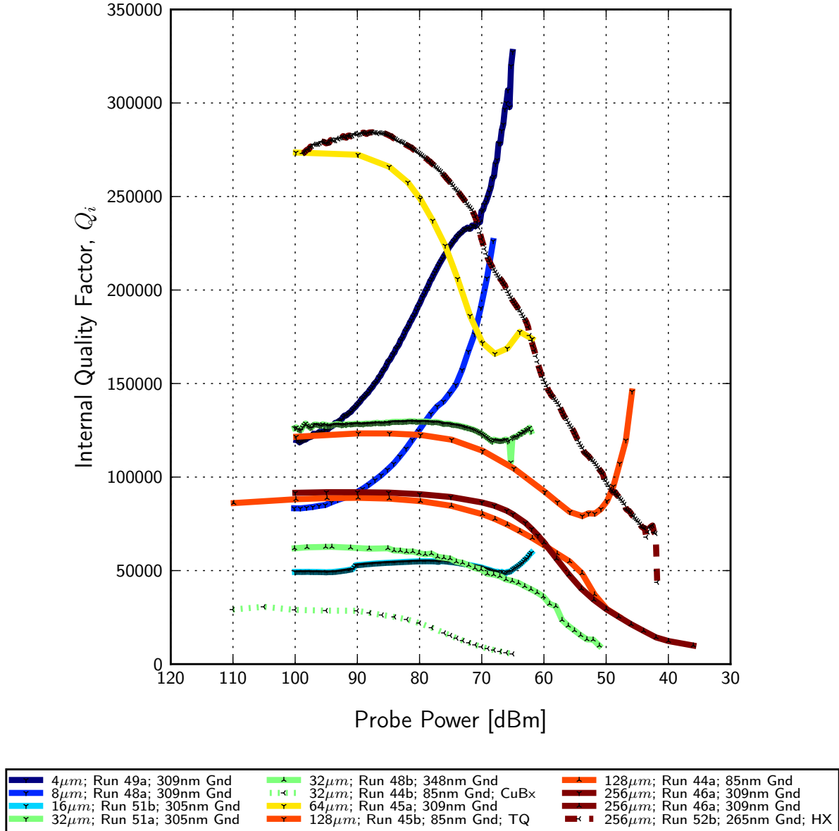
Figure 6.5: Internal quality factor versus probe power is plotted. Data run, microstrip trace ( \mu\text{m} ) and ground plane thickness (nm) are specified in legend. Abbreviations are: CB – copper box (otherwise niobium box), TQ – under-torqued press, HX – hexagonal mesh ground plane.
