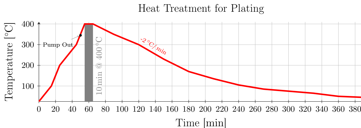
Figure 7.21: Heat treatment process for electroplated copper on Ti 15-3-3-3. The furnace is initially filled with argon gas. About five minutes prior to reaching 400 °C, the argon is pumped out leaving a residual pressure of 1 \cdot 10^{-5} torr for the remainder of the process. After 10 min at 400 °C, heating is turned off and the furnace cools at a rate of approximately -2^\circ\text{C}/\text{min} .
