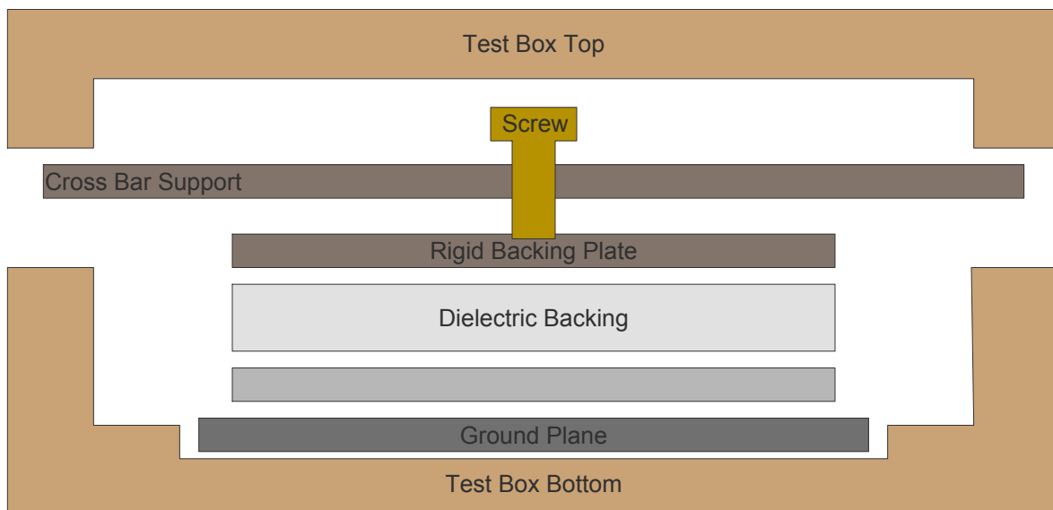
Figure 5.6: Exploded block diagram of device in screw press. The view is in cross section. The box top and bottom are either made of niobium, niobium titanium, or copper. The dielectric backing is made of teflon and is 1524\text{ }\mu\text{m} thick. The screw is usually brass, but could also be aluminum or Ti 6Al-4V. The rigid backing plate and cross bar support are made of Ti 6Al-4V. A rigid backing plate made of machined alumina is sometimes used as well. Although not shown, the cross bar support is screwed to the box bottom. Ti 6Al-4V becomes superconducting at 4.38\text{ K} [158]. The sensor chip is 500\text{ }\mu\text{m} thick
