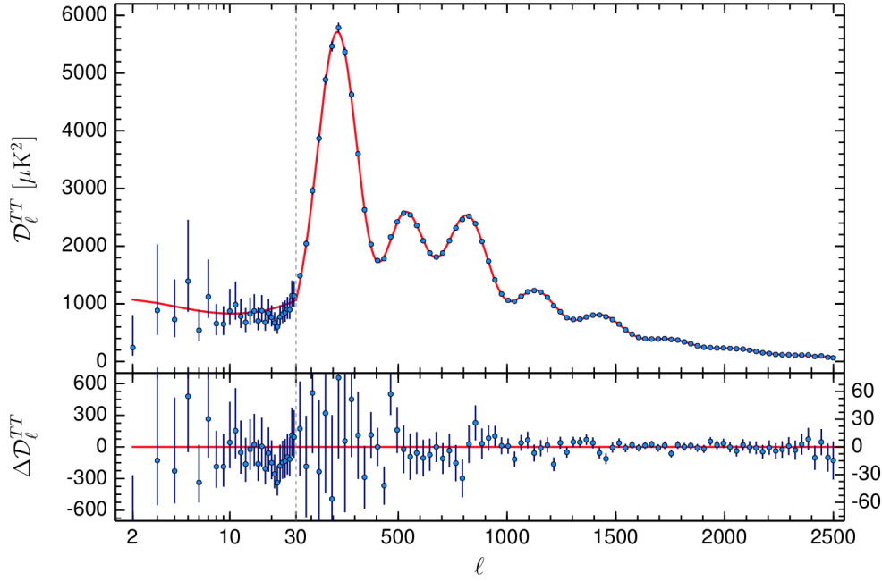
Figure 1.4: Temperature power spectrum of the CMB. Data is from the Planck Collaboration as of February 2015 and is the most accurate measurement of the CMB as of the time of this writing. Image from [148].
