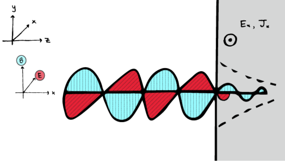
Figure 3.2: An electromagnetic plane wave at normal incidence with conductor. [3]
