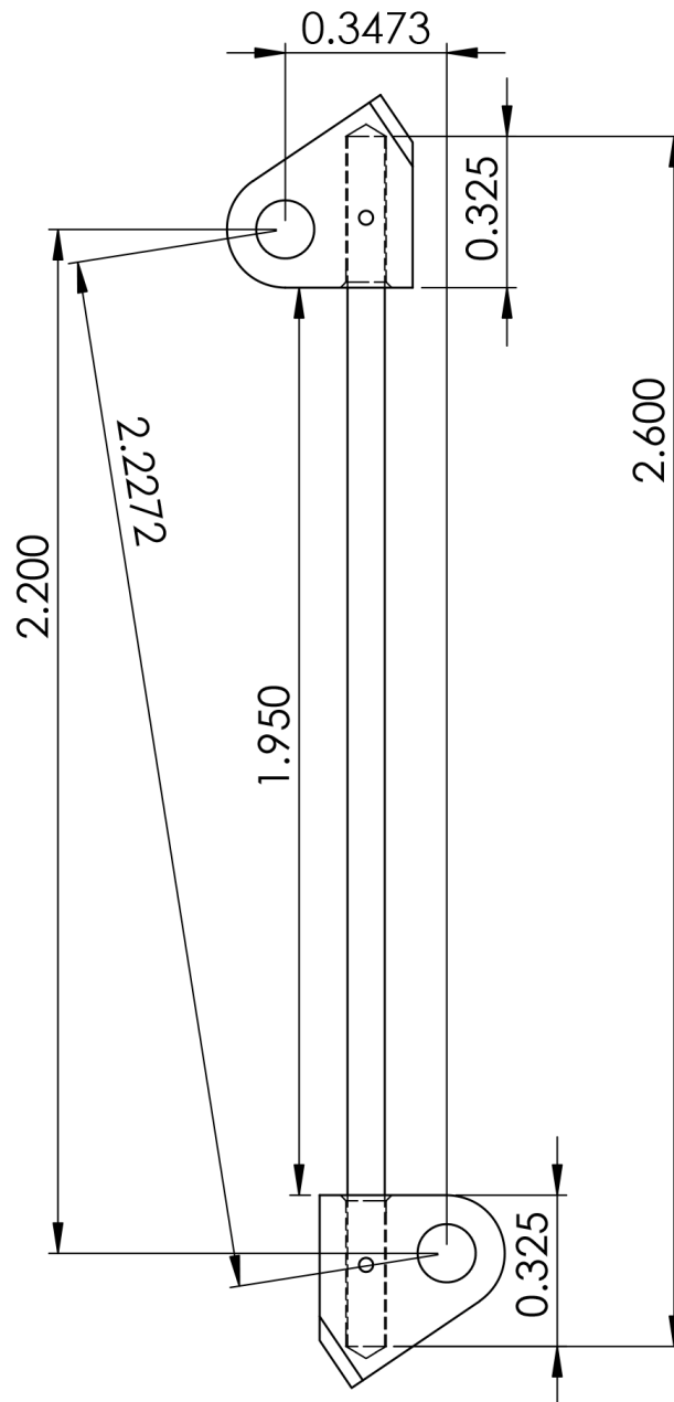
Figure D.9: Graphlite hexipod member fabrication drawing. Dimensions are in inches. Notice that the rod is not aligned with a line connecting the attachment hole centers. This leads to twisting and is a bad design. End caps made of brass. Graphlite rod epoxied into caps using gluing fixture and Stycast 1266.
