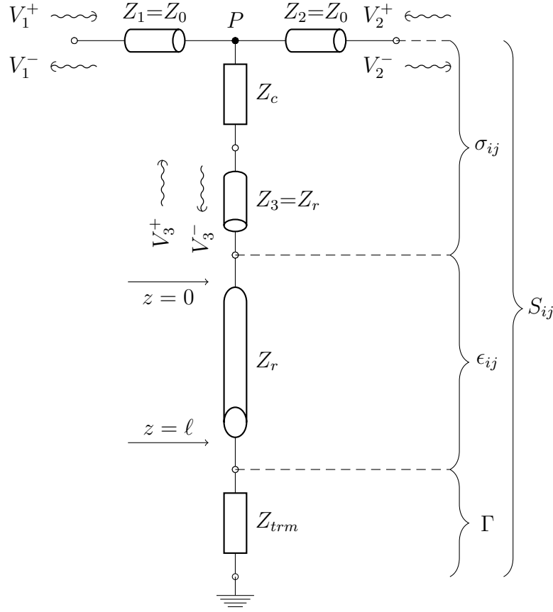
Figure 4.1: Network diagram of \lambda/2 resonator coupled to feedline. \sigma_{ij} , \epsilon_{ij} are the scattering matrices for the 3-port coupler and the 2-port \ell = \lambda/2 resonator section, respectively. The resonator termination, Z_{trm} , is represented as a reflection coefficient, \Gamma , and ideally it is a perfect open, \Gamma = 1 . S ports one and two are the same as \sigma ports one and two. \sigma port three is \epsilon port 1 and \epsilon port 2 is the port of \Gamma .
