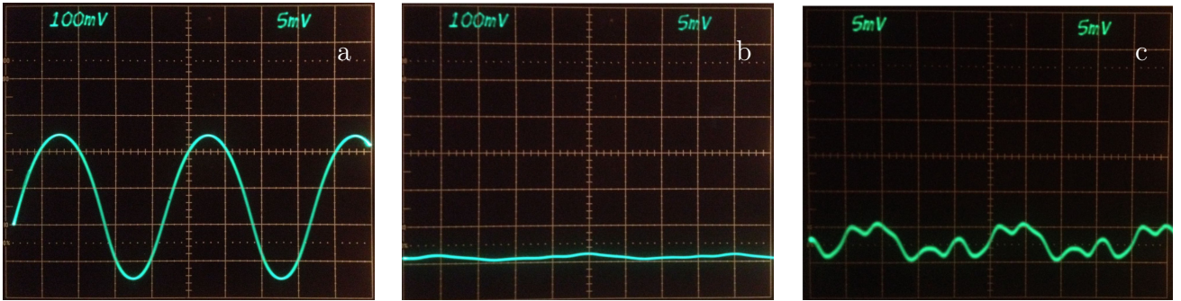
Figure 7.9: The modulation of a SuperCDMS SNOLAB SQUID array in the presence of nickel. View a shows the V - \Phi curve of a SQUID array without nickel; the modulation depth is 4 mV. View b shows the V - \Phi curve of a SQUID array but this time it is mounted on top of a 0.0014 inch thick copper foil that is plated with 0.000 05 inch of nickel. View c is a fine scale view of b . All measurements are done inside a magnetic shield – two-nested cryoperm cans around SQUID. Data from [10]
