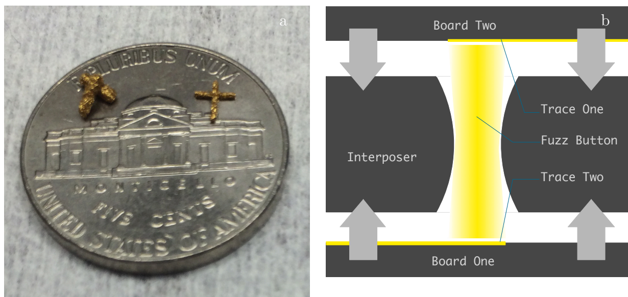
Figure 8.2: Fuzz button connectors are highly customizable. Custom materials can be used to make the. Those depicted in figure (a) are made of a molybdenum alloy. As seen in (b) they are instrumented in an interposer, which can be machined or molded a out of any dielectric material. Traces on the mating boards are aligned and mated together, usually with a screwable fastener simultaneously accomplishing both functions, such that the fuzz button is compressed and forms an electrical connection.
