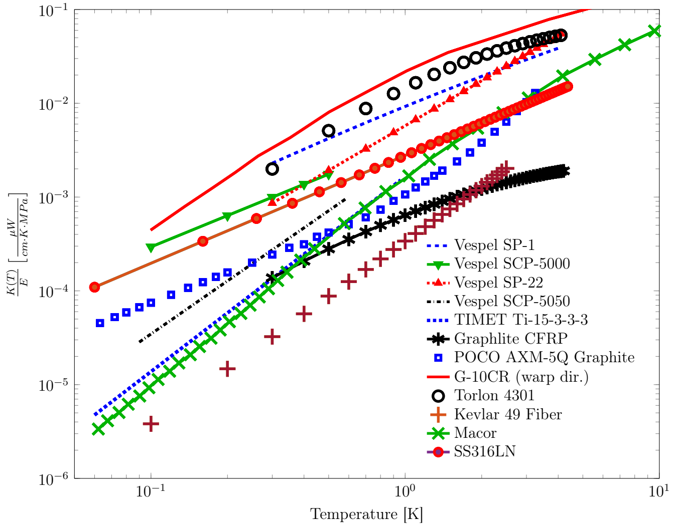
Figure 7.7: A selection of useful materials with their thermal conductivity normalized by their room temperature Young's modulus. Lower values are desirable as support materials. Thermal conductivity references: Vespel SP-1, Vespel SP-22, Graphlite CFRP, and Torlon 4301 from Runyan [162]; Vespel SCP-5000, Vespel SCP-5050, and Ti 15-3-3-3 from our original data [97]; AXM-5Q, G-10CR, and Macor from Woodcraft[199, 200]; Kevlar 49 from Ventura [187]; Stainless Steel 316LN from Barucci[26]. Young's moduli from Table 7.3
