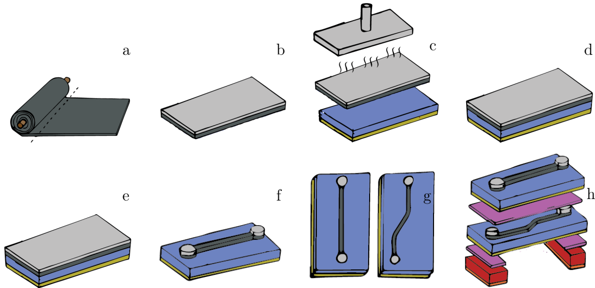
Figure 8.1: An alternative flex cable fabrication route is depicted. This route does not involve copper plating of the titanium foil and plates it with aluminum on only one side.
