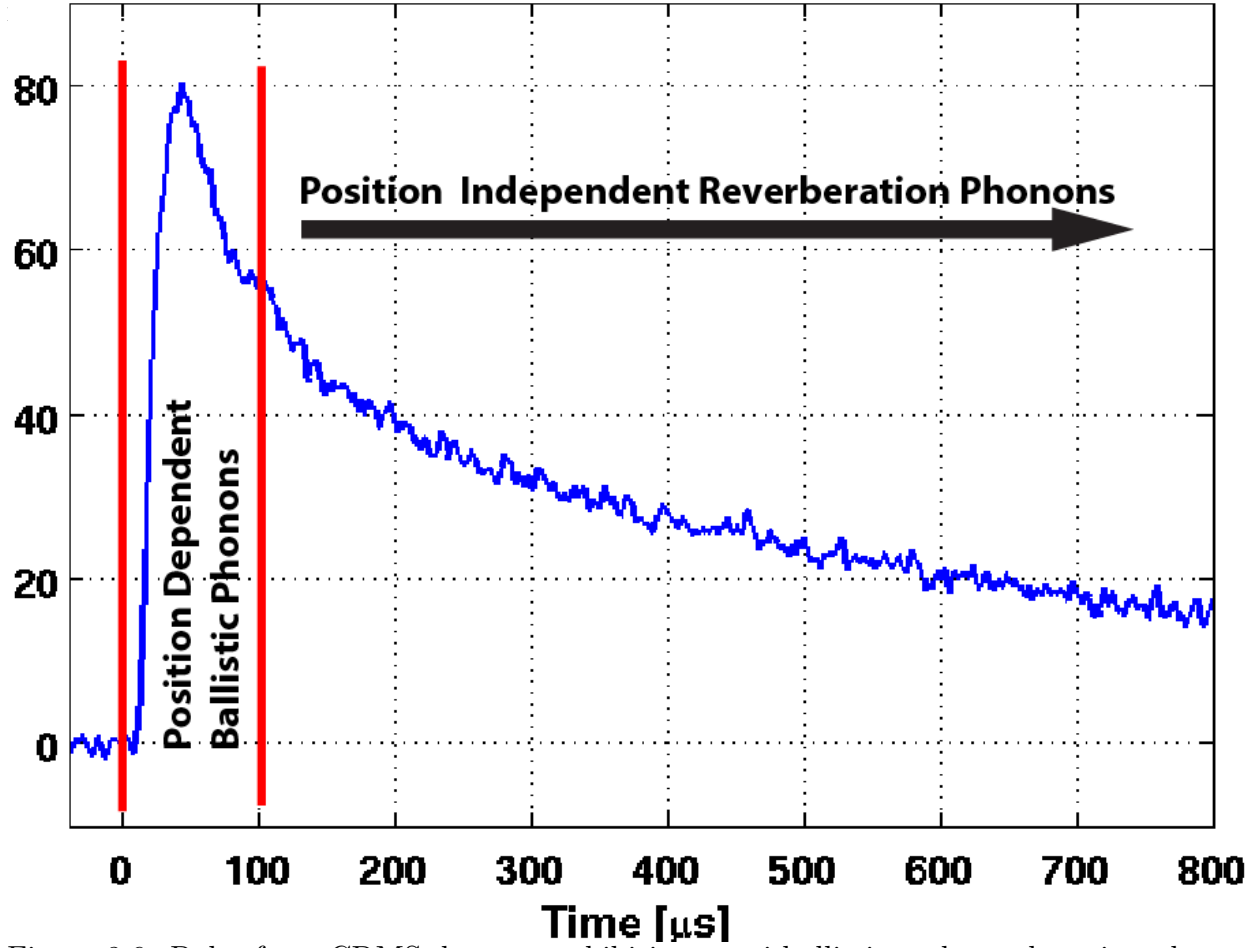
Figure 8.6: Pulse from CDMS detector exhibiting quasi-ballistic and reverberating phonon contributions.
