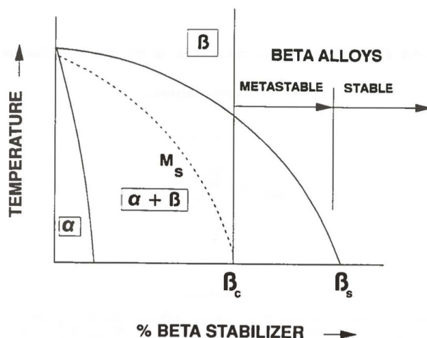
Figure C.9: The addition of beta stabilizing constituents suppress the beta transus of titanium alloys. For concentrations of beta stabilizing constituents, within a certain range, the alloys is metastable. Image from [23].
