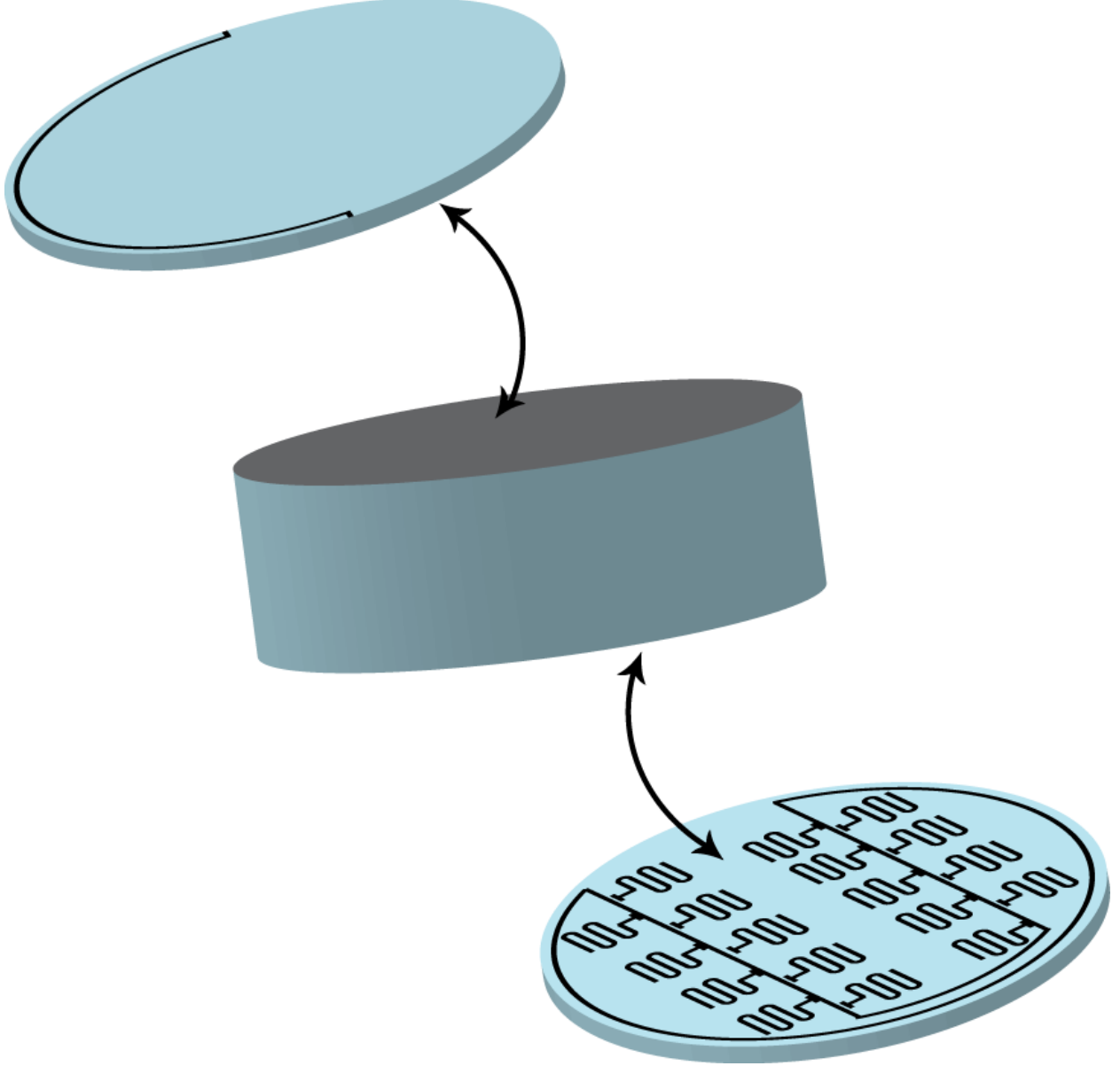
Figure 3.1: Our envisioned implementation of kinetic inductance phonon sensors for our dark matter detectors has the sensor function separated from the absorber function. Separate, standard sized, sensor wafers are attached to both faces of the germanium absorber. The sensor wafers carry the trace of a microstrip resonator, whose ground plane is directly deposited into the surface of the absorber. When an event occurs, the phonons impinge upon the ground plane and change its impedance. The change in impedance is detected as a change in the resonance by room temperature electronics. Position sensitivity is achieved by looking at the relative responses of all the sensors across the detector surface. The event will have occurred closest to the sensor (resonator) exhibiting the greatest response.
