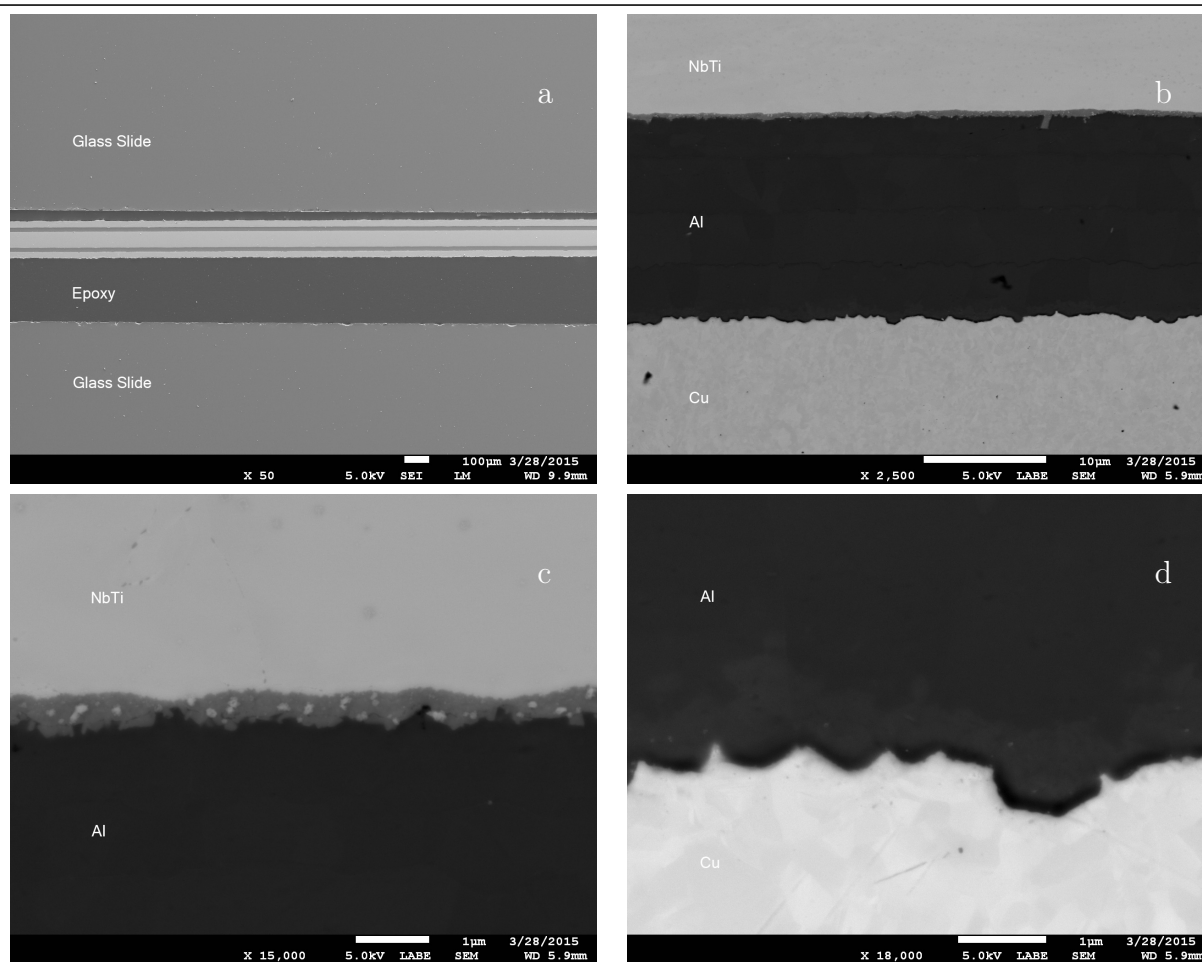
Figure 7.24: SEM micrographs of Nb-47Ti foil plated on both sides with aluminum via ion vapor deposition, and then electroplated copper. The bare Nb-47Ti foils is approximately 0.003inch thick. The plated samples are epoxied between two glass slides and then the stack is polished to expose the metal layers. No heat treatment on the plated sample was used. Views increase in magnification from a , to d .
