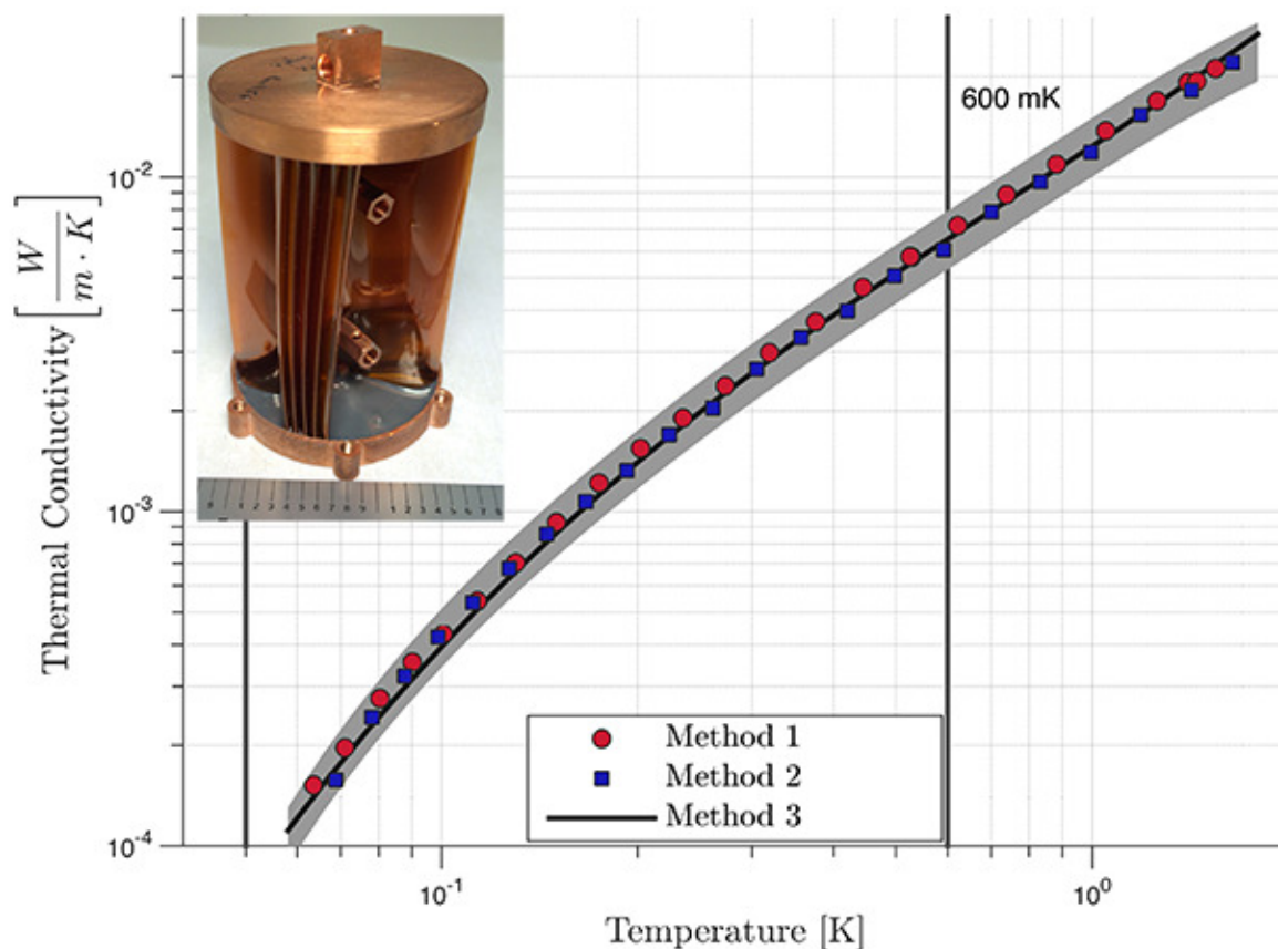
Figure C.2: Pyralux LF thermal conductivity.
