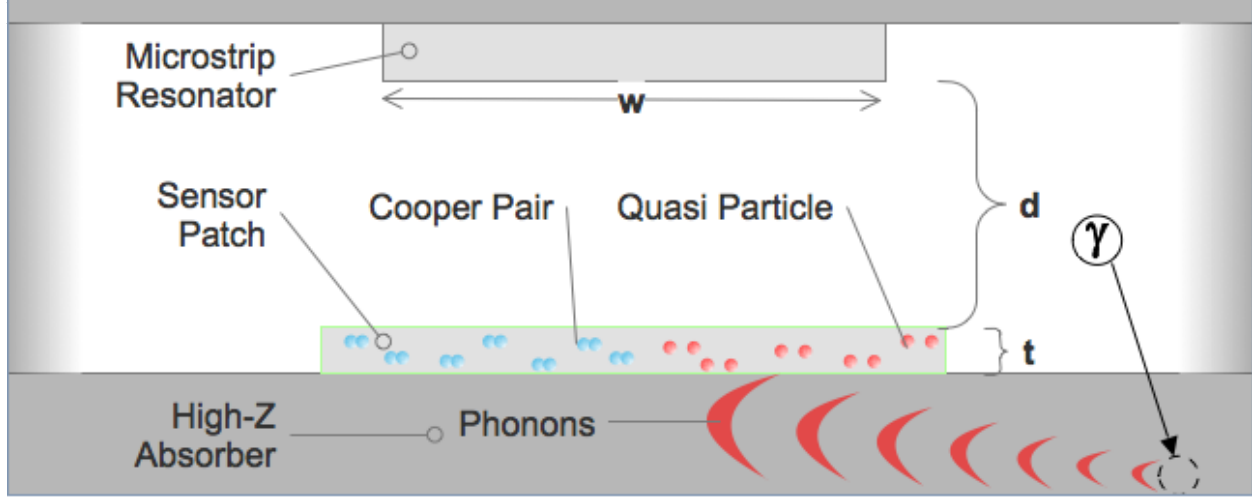
Figure 8.4: Magnified cross section of detector concept utilizing vacuum gap microstrip resonators to sense phonons. A patch of low gap superconductor (e.g. Al or TiN) is located beneath each resonator. Phonons impinging on the patch emanating from within the superconductor absorber break Cooper pairs and change its surface impedance which alters the resonance. Likely dimensions are w = 200 \mu\text{m} ; t = 200 \text{ nm} ; d = 3 \mu\text{m} .
