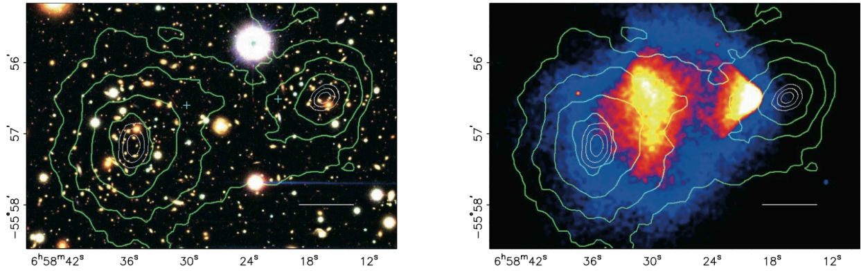
Figure 1.7: Observations of 1E 0657-558 ( z=0.296 ) the ‘bullet cluster’. On the left is cluster observed in visible light. On the right is the cluster observed in x-ray light. The contour lines overlaid on both images are map of the cluster’s gravitational potential obtained from a weak gravitational lensing analysis. One can see the ram pressure shock wave of the colliding cluster gas in the x-ray image. There is clear separation between the gravitational potential well and the cluster gas. Image from [44]
