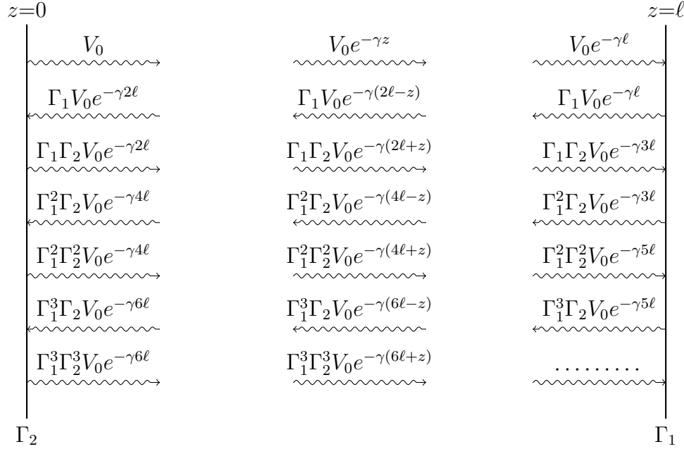
Figure 4.4: Inside the \lambda/2 resonator, the total voltage amplitude at any point z along the length is the sum of contributions from reflected waves.
