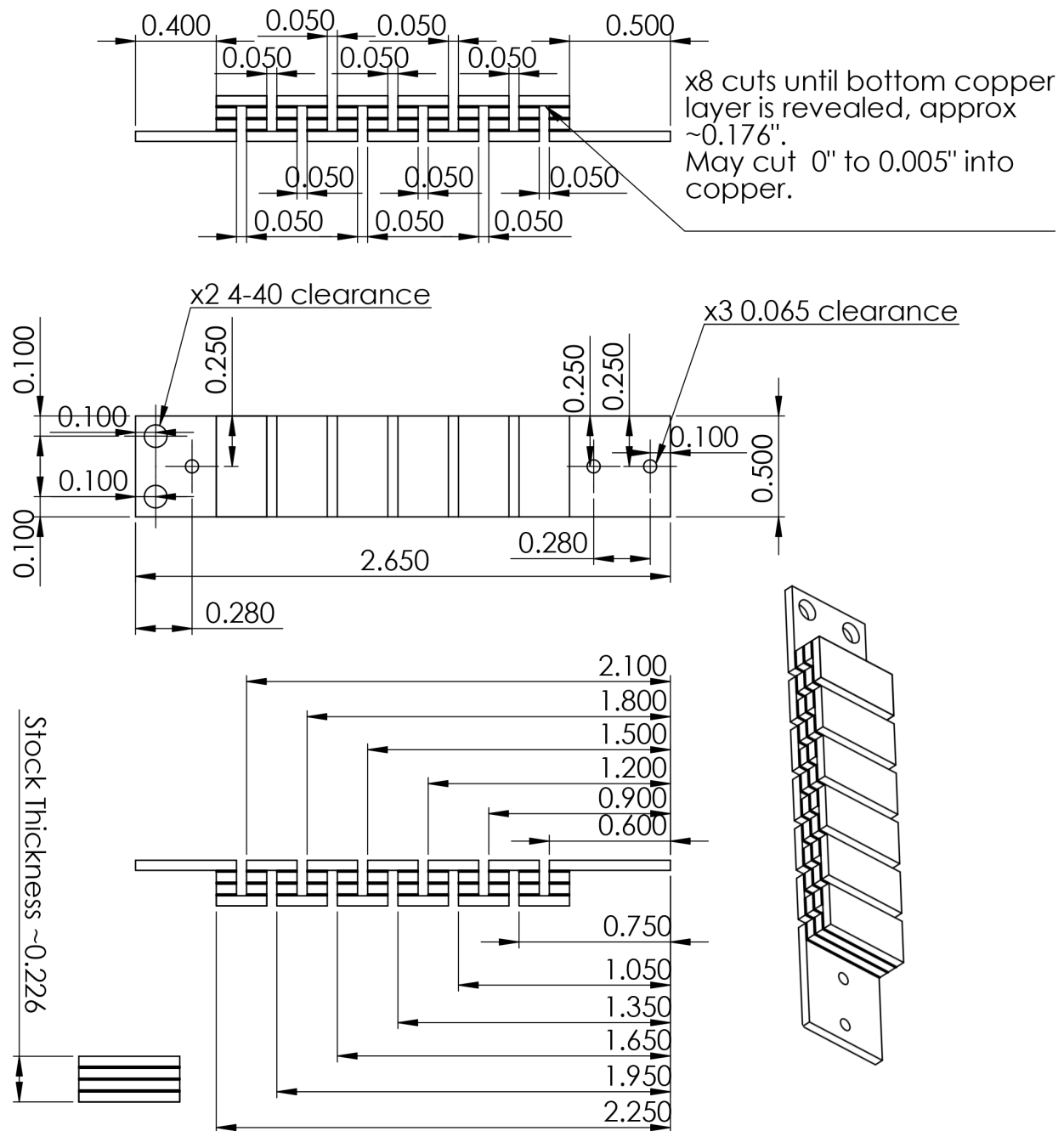
Figure D.1: Thermal resistance sample fabrication drawing. Dimensions are in inches.
