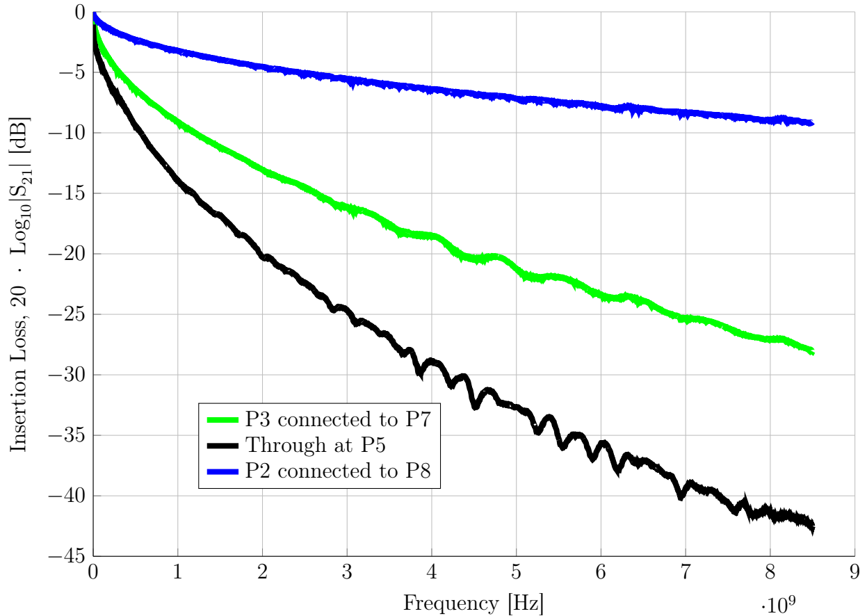
Figure 5.8: Measured round trip insertion loss of three portions of the readout system cabling. P2, P3, P5, P7, P8 are indicated on Figure 5.7 (a). Assuming that the cabling is symmetric in its loss characteristic on the inbound and outbound routes to the fridge, one way losses can be determined by halving the measured quantities. The losses of cabling segments can be determined by subtraction of the measured quantities. The fridge was at base temperature for the measurement of curves “P3 connected to P7” and “Through at P5”.
