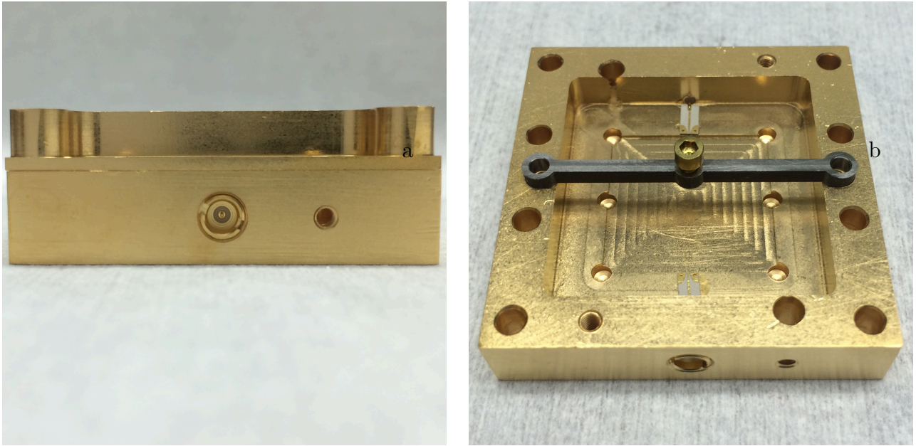
Figure D.5: View if a fabricated KIDs test box, made of copper plated with gold, no nickel diffusion barrier plate. (a) – One sees the SMP blind mate connector. (b) – The titanium cross bar for the press and the transition pads are in place.
