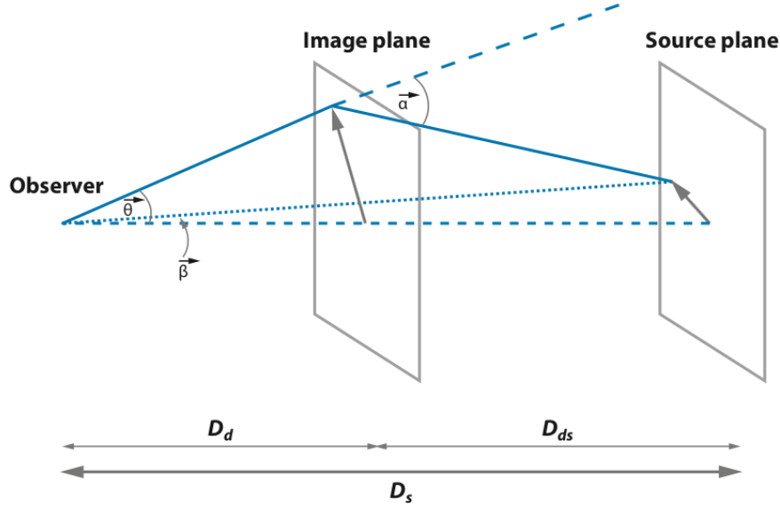
Figure 1.5: Gravitation lensing diagram. The image plane is positioned between the observer, and the source plane. The true source at \beta is off set for the position of its image, \theta , due to the gravitational lensing effect. Image from [182]
