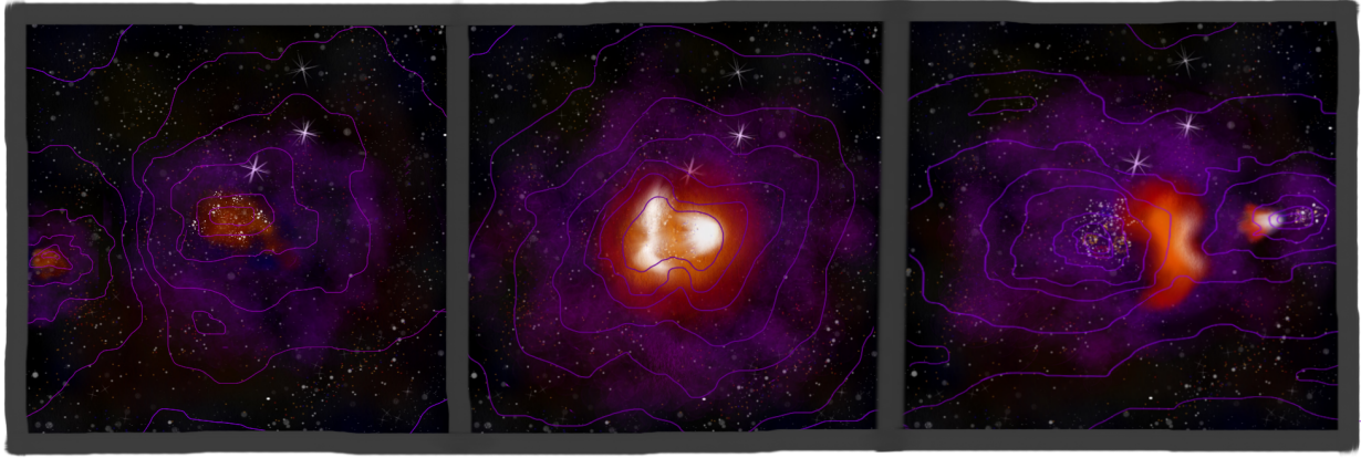
Figure 1.8: An artist's visualization of before, during an after the bullet cluster collision. Telescope images of the bullet cluster is currently observed it the stage illustrated in the right most comic strip view. In the left most view, the background light sources establish a reference frame which has the smaller cluster on the left moving toward the larger cluster in the center. The dark matter distribution is shown by weak lensing dark matter distribution contours and purple haze. In the center view, white to orange coloring emphasizes strong x-ray emission from colliding cluster gasses. In the view, we see the dark matter and compact objects moving unimpeded by the collision while the gas, indicated by the x-ray emission, lags behind due to substantial interactions in the collision. [2]
