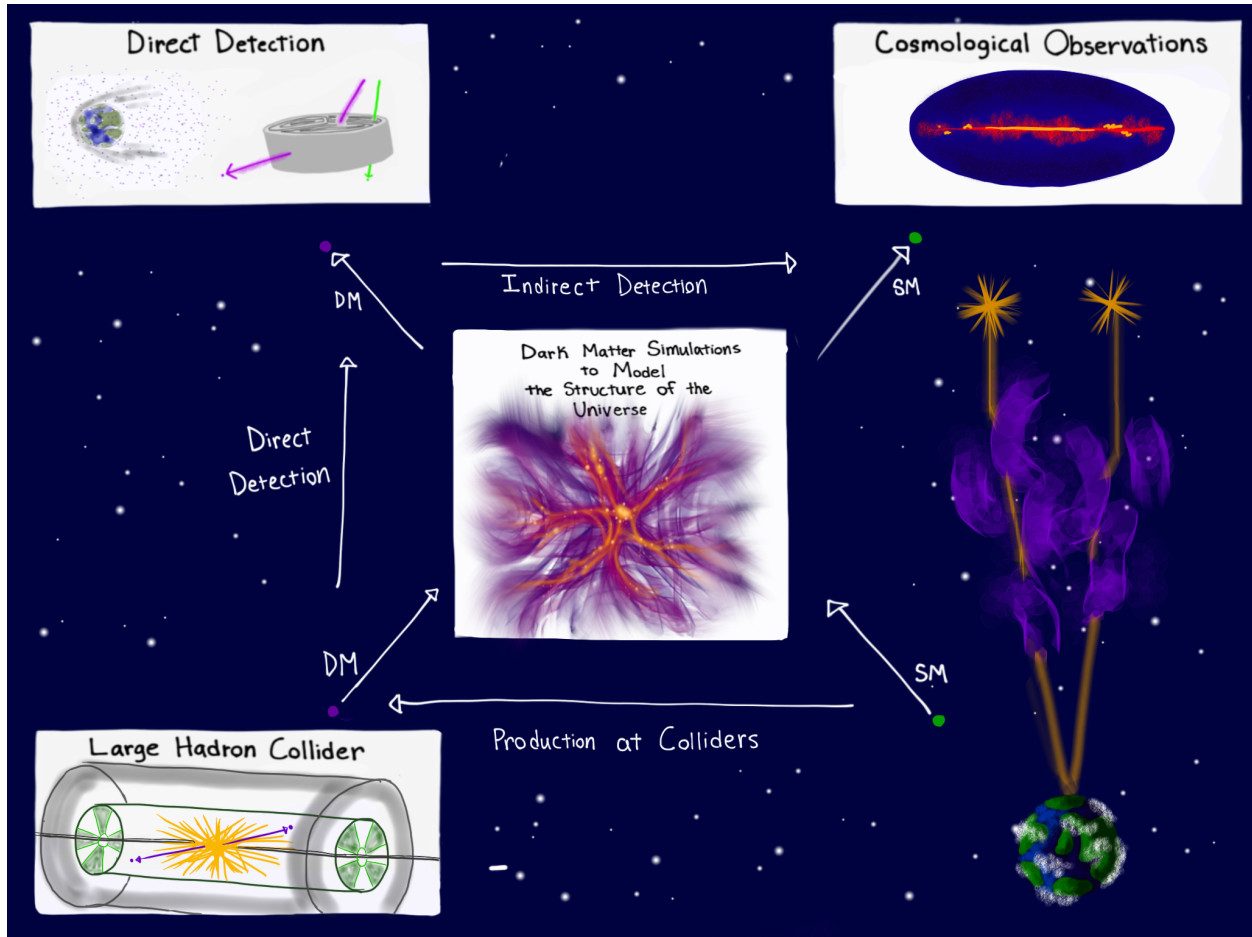
Figure 2.1: Illustration of the complementarity between dark matter detection approaches and simulations. Each of these activities benefit from the successes of the others and progress in any contributes to our understanding of the universe. At the center of the illustration we place the efforts to understand dark matter by computer simulation, though this is not meant to imply they are any more important than the three detection approaches. We also indicate how the interaction of dark matter (DM) particles with standard model (SM) particles is associated with the detection approaches, for example collider detection entails production of dark matter from standard model particles, while indirect detection, such as annihilation entails dark matter particles producing standard model particles. The notable exception is lensing, which depends on fundamental physics that are not yet sorted out. Image from [2].
