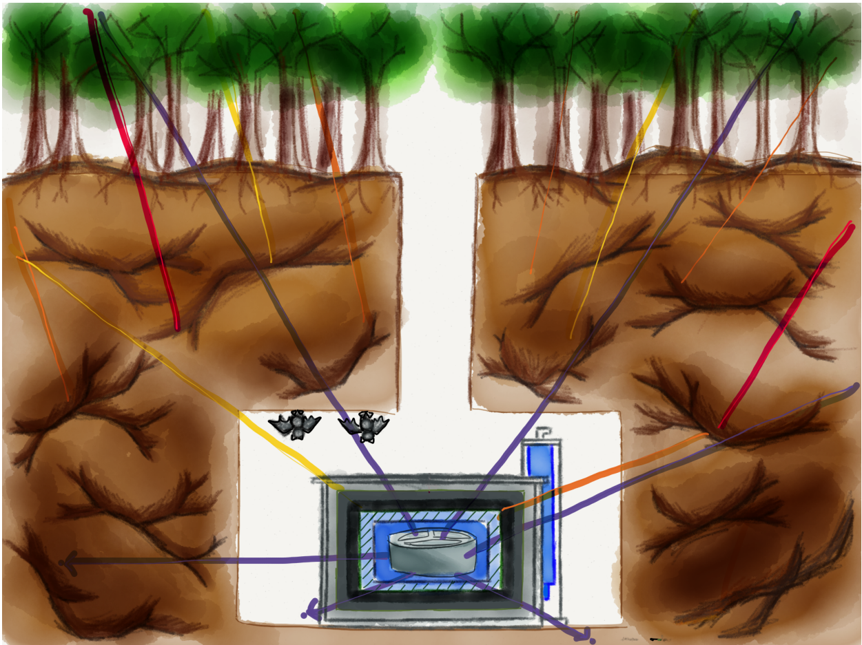
Figure 2.3: Illustration of dark matter detector deployed in an underground laboratory. The overburden of rock shields the detector from most cosmic radiation but WIMPs (in purple) would have no problem reaching the detector. The illustration depicts the CDMS detector, with its pattern of charge and phonon sensors visible, in the Soudan Underground Laboratory, which is located in Northern Minnesota. Bats are frequent visitors to the experimental chambers which are nearly a half mile underground. Image from [2].
