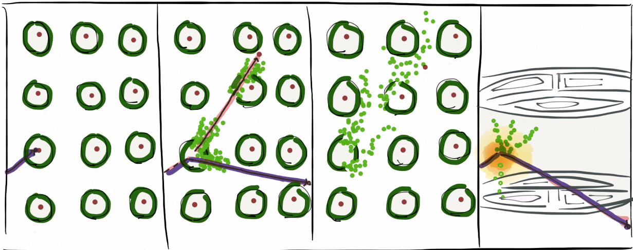
Figure 2.2: Comic strip illustration of the principle of direct detection in a semiconductor absorber. A WIMP of cosmic origin collides with an atomic nucleus in a semiconductor absorber. In this case we have a germanium crystal in mind. The recoiling nucleus produces phonons, in orange, and ionization in the form of electrons and holes, green dots. WIMP interactions are so rare that it is exceedingly unlikely the same WIMP will interact twice in the detector. However the recoiling nucleus may be ejected several atomic spaces and interact with other atoms in the lattice as it recoils. The ionization is pulled to the surface of the detector by an electric field. Holes and electrons travel with different trajectories with respect to the field. The phonons eventually reach the surface too. Image from [2].
