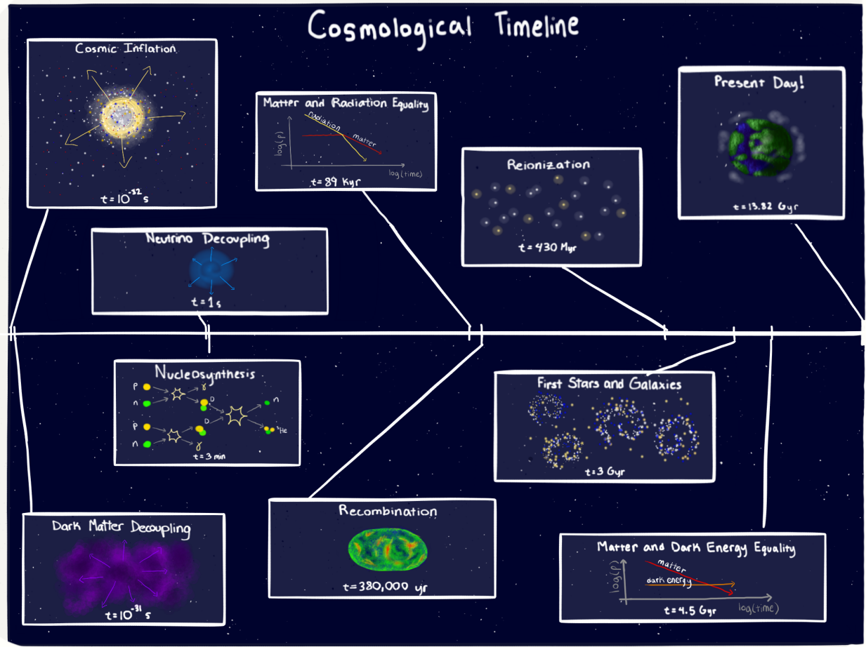
Figure 1.1: A summary of the major events that occurred between present time and the Big Bang, presented in chronological order. We see that the dark matter, which our objective is to detect and characterize, should have been around since very shortly after the big bang. [2]
