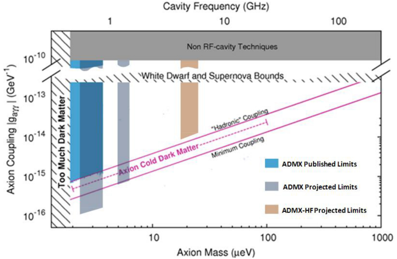
Figure 2.9: Areas of mass-coupling constant parameter space which lie within the colored regions for a given experiment are excluded by that experiment's data. Image from [171].
