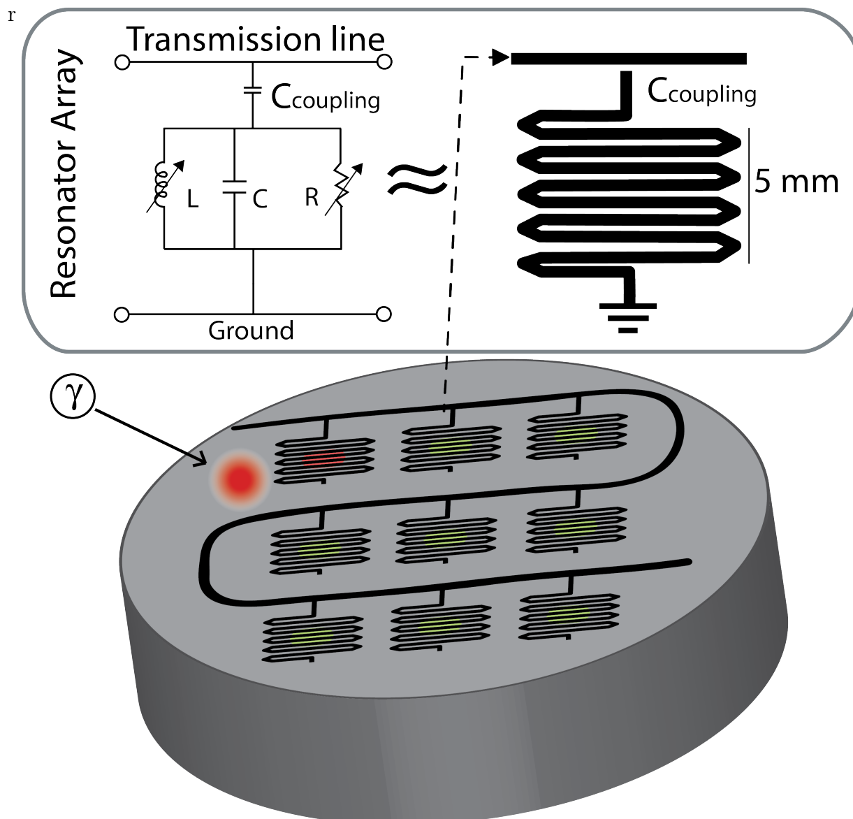
Figure 8.5: The idea of a KIDs phonon sensor array fabricated on a large absorber is depicted. Gamma rays deposit energy in the absorber. The energy is radiated away from the interaction location by phonons. The phonons arrive at the surface of the detector where they create quasi-particles in patches of low gap superconductor there are patterned onto it. The patches are part of the ground plane of a superconducting resonant circuit and the quasi-particles affect a change in quality factor and resonant frequency for of the resonant circuit, which is detected by room temperature electronics. The interaction location can be reconstructed from analysis of the responses of all the resonators. E.g the resonator that is closet to the interaction location will have the greatest response.
