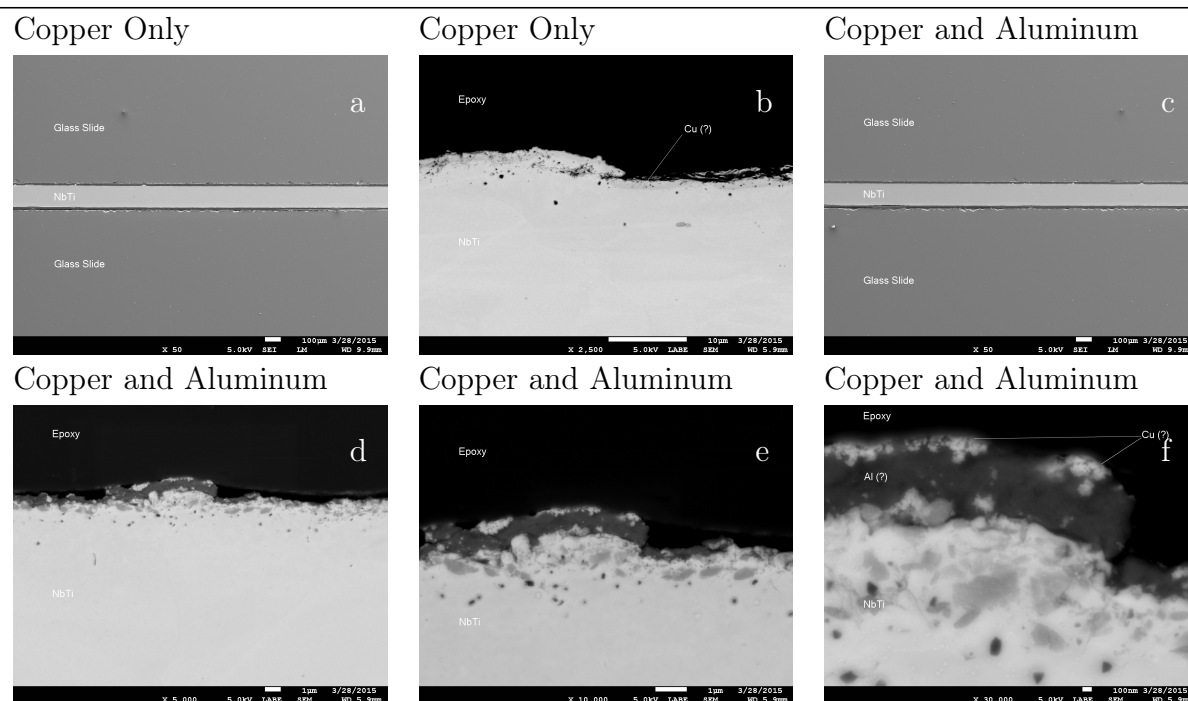
Figure 7.23: SEM micrographs of Nb-47Ti foil with aluminum and copper evaporated onto plated on both sides. Two samples are shown. The first, views a and b , is copper plated only with a target thickness of about 1.6\mu\text{m} . The second, views c through f , is plated with 0.8\mu\text{m} aluminum, then 0.8\mu\text{m} copper. For both samples the platings are not clearly evident. Perhaps this is because the layers are so thin, or because adhesion may not be good. The is likely a combination of both. The plated samples are epoxied between two glass slides and then the stack is polished to expose the metal layers. No heat treatment on the plated sample was used. Views increase in magnification from a to d , and from c to f , which a and c the lowest magnification.
