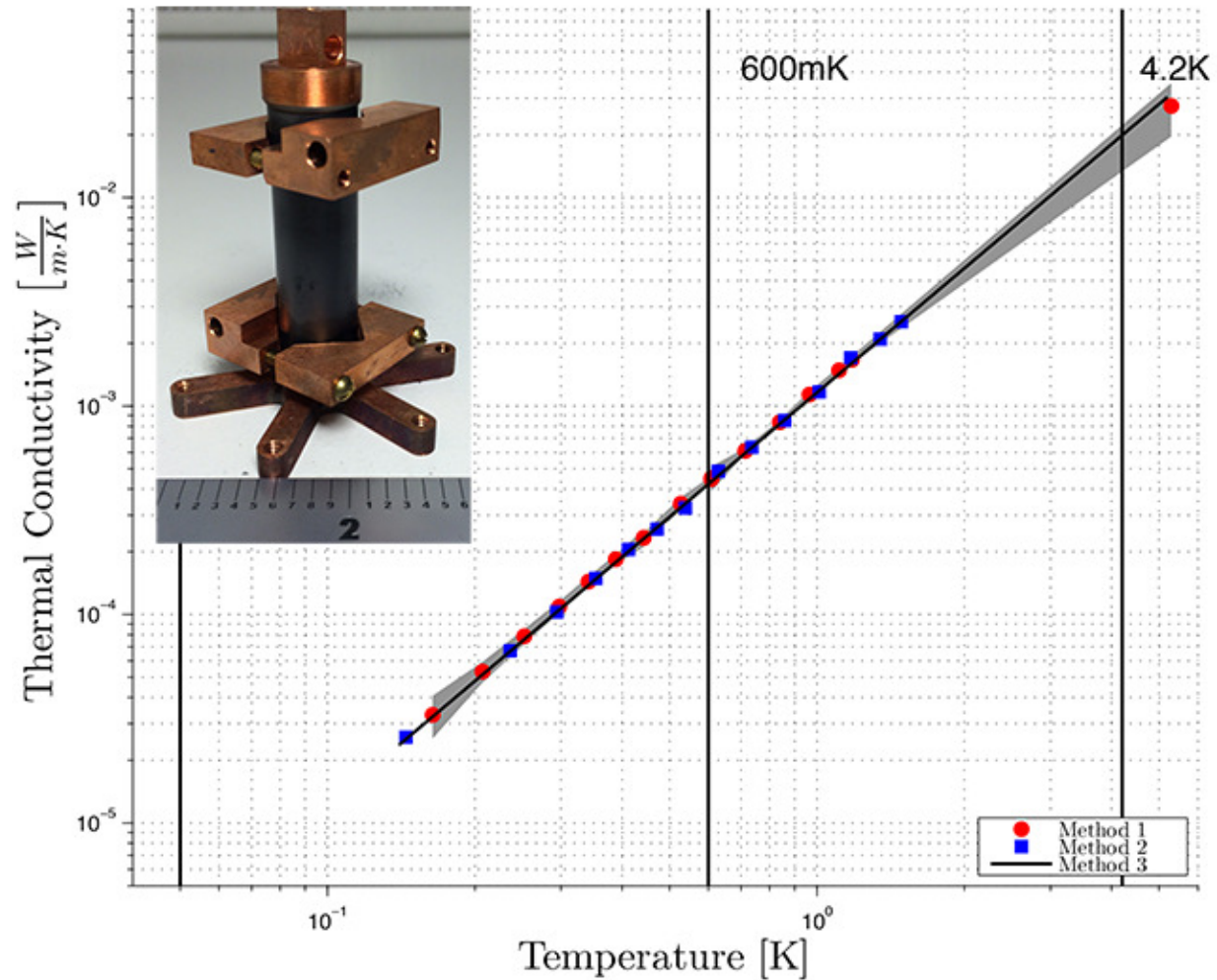
Figure C.8: Vespel SCP-5050 thermal conductivity. A second data set with extended temperature range.
