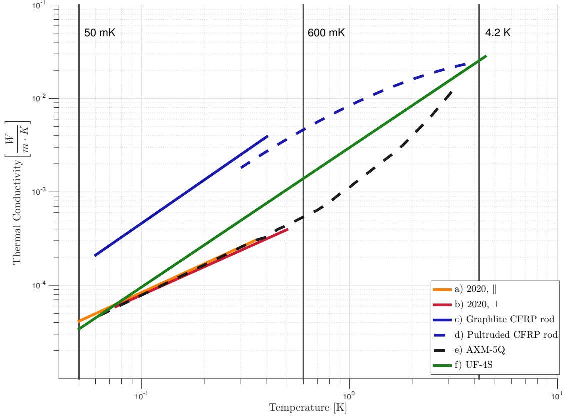
Figure 7.3: Thermal conductivity of graphite-like materials. Data source, additional sample information and the direction of heat flow (when known) are as follows : a ) original data [6], \parallel to grain structure in bulk rod sample material manufactured by the Mersen Corporation; b ) original data [6, 97], \perp to grain structure in bulk rod sample material manufactured by the Mersen Corporation; c ) original data [6, 97], \parallel parallel to the axis of rod sample, carbon fibers aligned to this axis on average and made by Avia Sport Composites; d ) from Runyan et al. [162], \parallel parallel to the axis of rod sample, carbon fibers aligned to this axis in average; e ) from Woodcraft et al. [199], industrial grade petroleum coke based fine-grained isotropic moulded graphite, graphitized at 2500 °C by the Poco Corporation, and f ) from Leman et al. [113] an unpublished CDMS internal report, \parallel to axis of tubular sample from material manufactured by the Mersen Corporation
