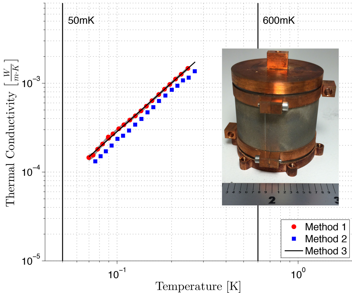
Figure C.12: Ti-15V-3Cr-3Sn-3Al rod thermal conductivity.
