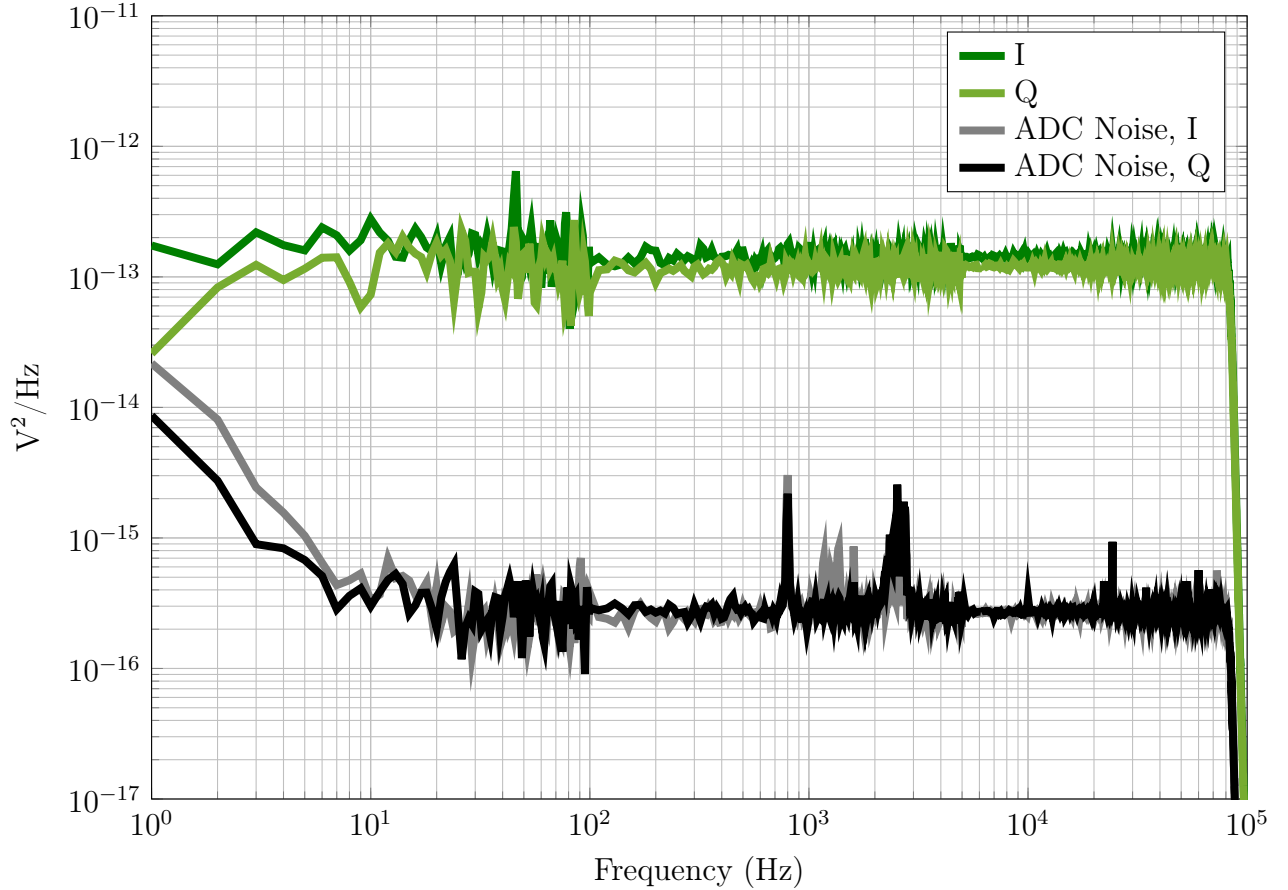
Figure 5.9: The noise of the readout system diagrammed in Figure 5.7 where (a) is connected to (d), the NI Digitizer configuration, at the output of the digitizer. I and Q noise is measured when the probe signal entering primary LNA is approximately -90 dBm at a frequency of 690 MHz. The digitizer noise is measured with 50\ \Omega terminators in parallel to the digitizer input (which has an impedance of 1\ \text{M}\Omega ). The noise is measured while the fridge is at base temperature.
