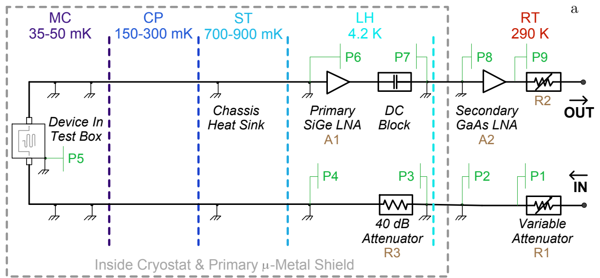
Figure 5.7: KIDs readout system configurations used to measure data. a – The “device end” portion of the readout system that does not change. The cryostat is a customized Oxford 75 \mu W helium dilution fridge. The \mu -metal shield is a cylinder with one end open and one end capped and it is on the exterior of the cryostat. Chassis ground symbol denote heat sinking of the coax (and test box) shell to the fridge chassis. Points of interest, P1 through P9 are discussed elsewhere.
