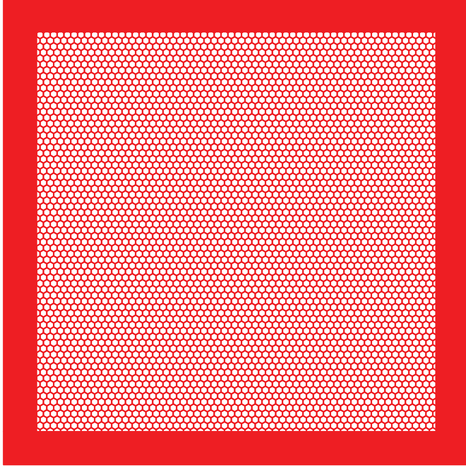
Figure 5.4: Lithography mask pattern for a hexagonal mesh ground plane fabricated in a vacuum microstrip KID. The red part is metal. The hexagon voids in this particular ground plane are 292\text{ }\mu\text{m} inscribed diameter; the metal mesh is 16\text{ }\mu\text{m} wide; and the metal area fraction is 5%.
