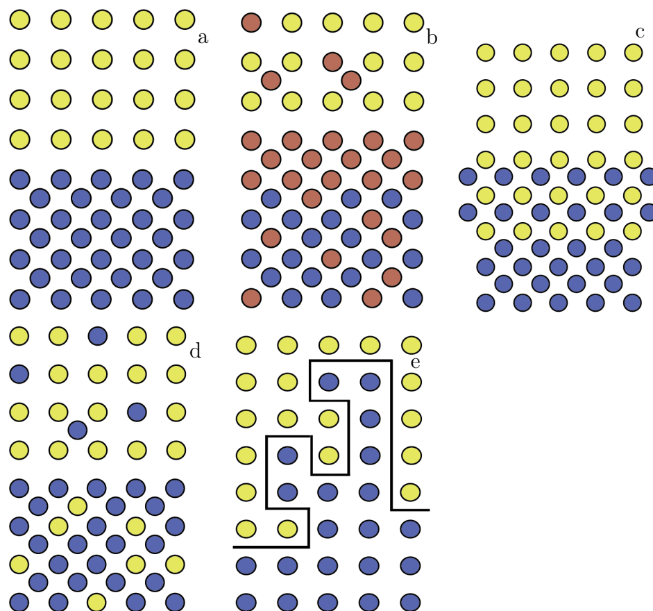
Figure 7.16: The five images depict different types of interfaces involved in the adhesion between different materials. (a) – an abrupt interface where the first material transitions to the second in the length of a few atomic separations. Adhesion would be weak in this case. (b) – The two materials attach to a common third material interfacial layer, such as oxygen or a reactive metal. Adhesion has the potential to be excellent here because the third material can be chosen to be very reactive with the other two. (c) – the two materials form a chemical compound (e.g. an intermetallic) at the interface. The adhesion can be good if the compound has good mechanical properties. (d) – the two materials diffuse in to each other. Adhesion can be great if the two materials are mutually soluble and if the materials have similar mobilities into the other. Kirkendall voiding can occur if the mobilities are not similar. (e) – mechanical interlocking of the two materials at the interface enhances adhesion. Roughening of the surfaces can thus be used to enhance adhesion through this mechanism. Mechanical interlocking is important for the adhesion of vacuum metallized and electroplated layers. Interfaces (b), (c), (d) can be influenced by heat treatment. Illustration by [3] and inspired by [137, Figure 12-22].
