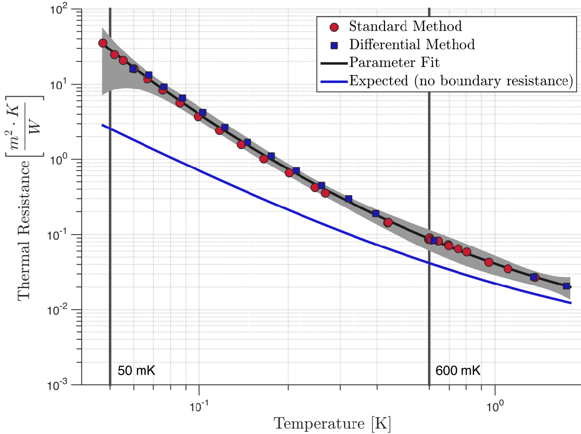
Figure 7.32: The measured total thermal resistance of the vertical cable heat sink compared to the expected total thermal resistance if no boundary resistances are present. The shaded region represents the measurement uncertainty at the 60% confidence level. We use the three different analyses described Appendix C to obtain the data point, except that we solve for R(T) = \frac{t}{\kappa(T)} , where the thickness t takes the place of length l .
