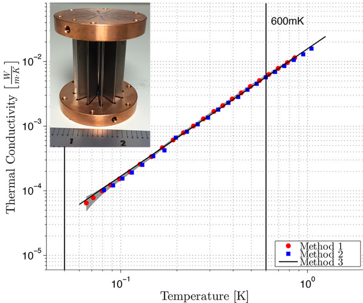
Figure C.10: Ti-15V-3Cr-3Sn-3Al plate thermal conductivity
