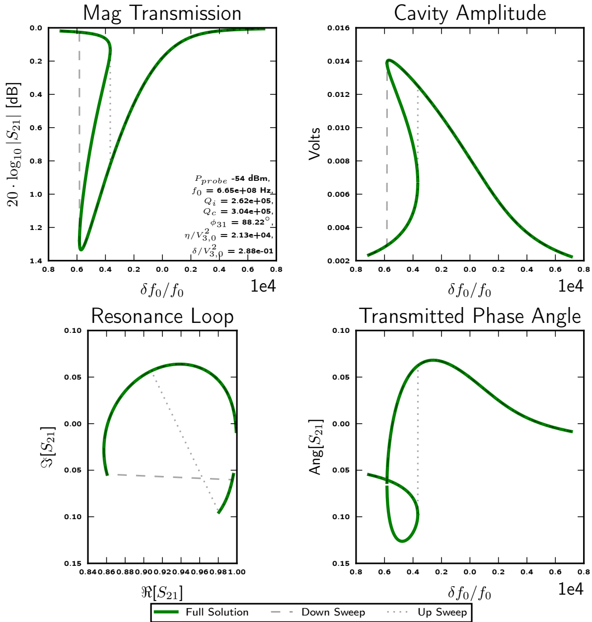
Figure 6.11: The power sweep for Run 45a, a 64 \mu\text{m} resonator, is fit to extract the nonlinear parameters, which are called out in the upper left plot. Additional electrical parameters are obtained from Table 5.1. The nonlinear model equations, described in § 4.2.2, are solved for P_{probe} = -54 dBm using the method described in the current section. Dotted and dashed lines indicate the direction of the frequency sweep. The data presented throughout this chapter uses an upward frequency sweep, unless explicitly stated otherwise.
