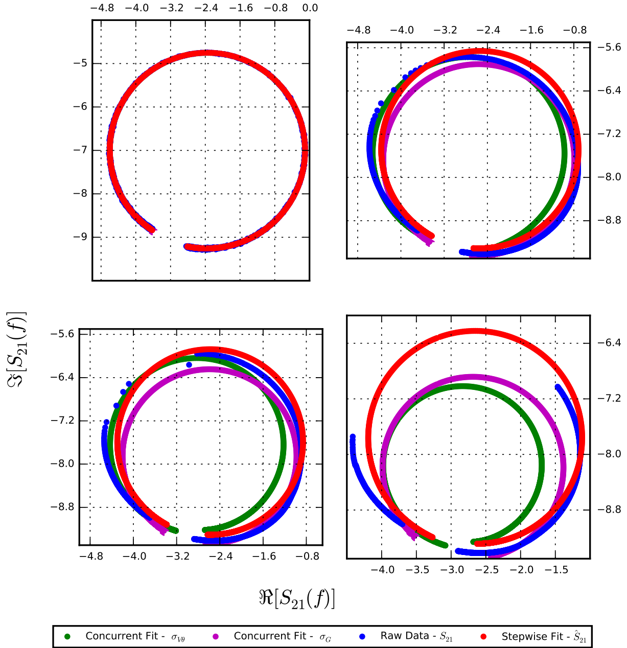
Figure 6.4: The S_{21} loops for the magnitude curves shown in Figure 6.1 are plotted along with the results from the primary fit and the secondary fit. Upper left plot is P_{probe} = -100 dBm, upper right is P_{probe} = -72 dBm, lower left is P_{probe} = -70 dBm, and lower right is P_{probe} = -66 dBm.
