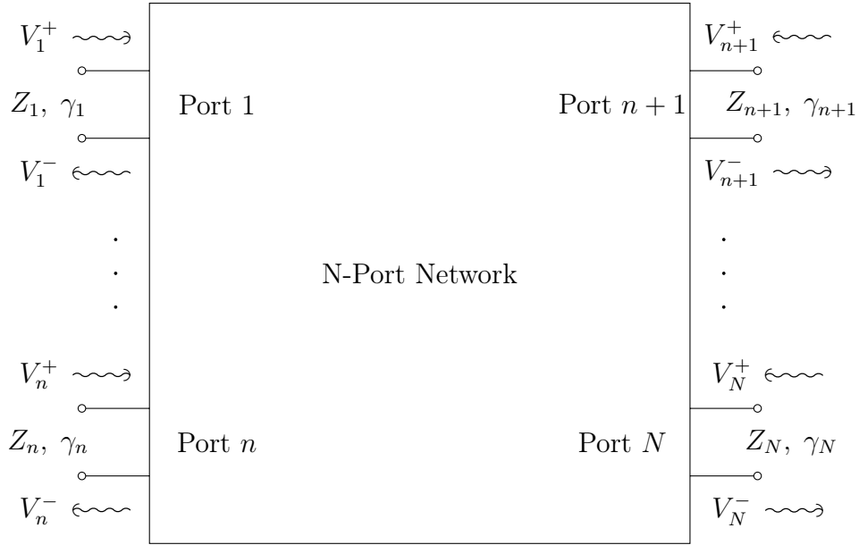
Figure 4.3: An N -port microwave network has a Z_n and \gamma_n at each port, which are imagined as zero to finite length transmission lines.
