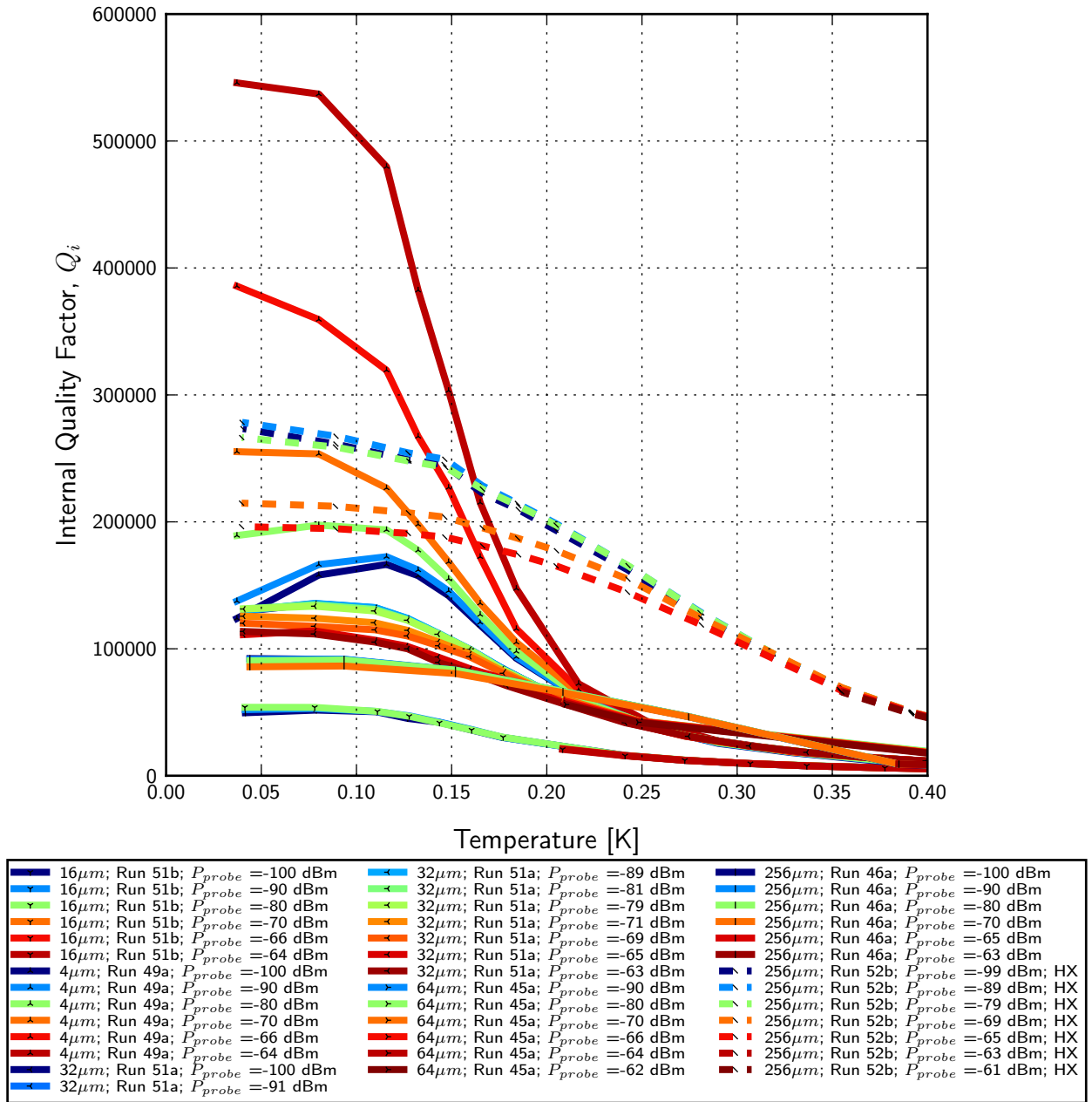
Figure 6.10: Internal quality factor versus probe power and temperature. The parameter generally decreases with temperature, as expected. Data run, microstrip trace width ( \mu\text{m} ) and ground plane thickness (nm) are specified in legend. Abbreviations are: CB – copper box (otherwise niobium box), TQ – under-torqued press, HX – hexagonal mesh ground plane.
