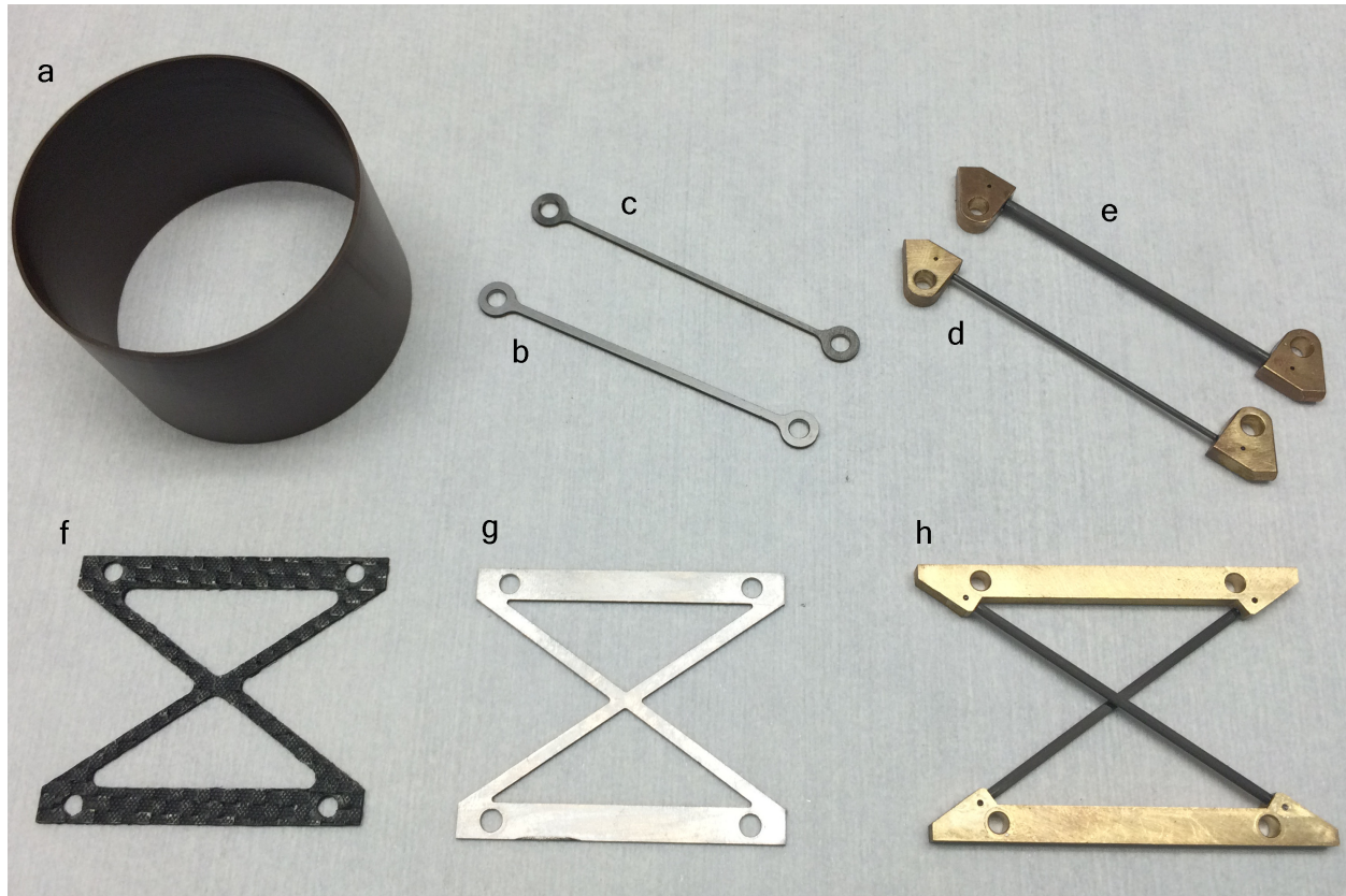
Figure 7.10: Structures considered for tower standoffs. All structures would be fastened by screws to the tower floors, except the tubes which would be glued. The standoffs are: a – tubes, made of either vespel, graphite or Ti 15-3-3-3; b (and c ) – Ti 15-3-3-3 hexipod truss member 0.04 inch thick by 0.04 inch (0.06 inch) wide; d (and e ) – graphlite rod hexipod truss member \varnothing 0.08 inch ( \varnothing 0.04 inch); f (and g ) – carbon fiber reinforced epoxy (Ti 15-3-3-3) X-frame member 0.04 inch thick by 0.083 inch; and h – graphlite X-frame using \varnothing 0.062 inch rods
