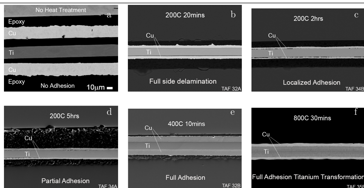
Figure 7.22: SEM micrographs of Ti 15-3-3-3 foil electroplated on both sides with copper viewed in cross section. In all images, the Ti 15-3-3-3 foil is approximately 0.0008 inch thick. The plated samples are epoxied between two glass slides and then the stack is polished to expose the metal layers. The heat treatment occurs in a vacuum atmosphere, 10^{-5} torr, which is initially back filled with argon to remove the air. The peak temperature and time at this temperature for each heat treatment process is indicated on the images. Dark voids between the Ti 15-3-3-3 and the copper can be seen in images a , b , c and d indicated lack of adhesion. Image f has full adhesion, but the duration and temperature of the heat treatment resulted in a transformation of the Ti 15-3-3-3 microstructure; \alpha -titanium precipitate is visible. Image e has full adhesion and no discernible transformation; this heat treatment process is successful.
