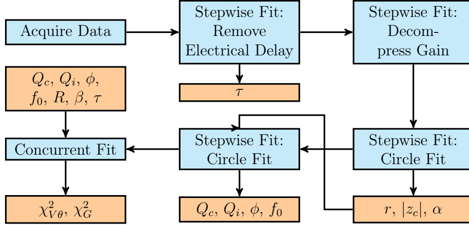
Figure 6.2: A flow chart of the procedure used to fit resonances that are in the linear regime. The fit parameter outputs and inputs are indicated for each step. One sees that the output of the circle fit is the circle center and radius, r = Q/Q_c . The concurrent fit uses parameter values determined by the stepwise fit as its initial guess. It also, optionally, uses a reduced data set, post-cuts, rendered in the phase fit. It is performed in two different ways. One which looks at readout system component induced errors in the magnitude and phase of the measured signal and another which derives an error from the noise in the measured scattering parameter data. z_c = |z_c|e^{i\alpha} is the vector to the loop center.
