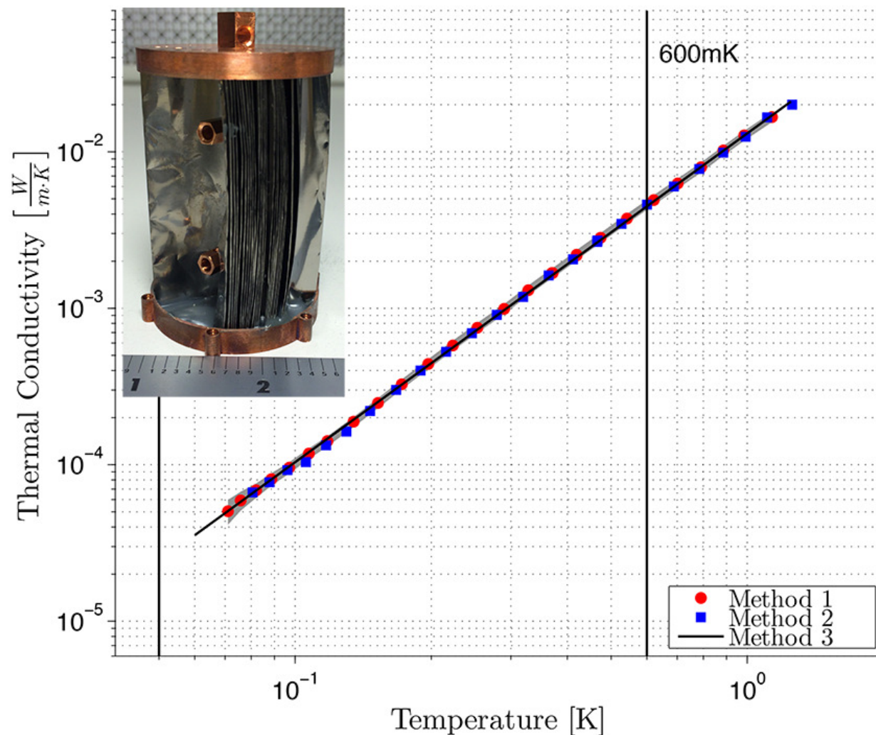
Figure C.11: Ti-15V-3Cr-3Sn-3Al foil thermal conductivity.
