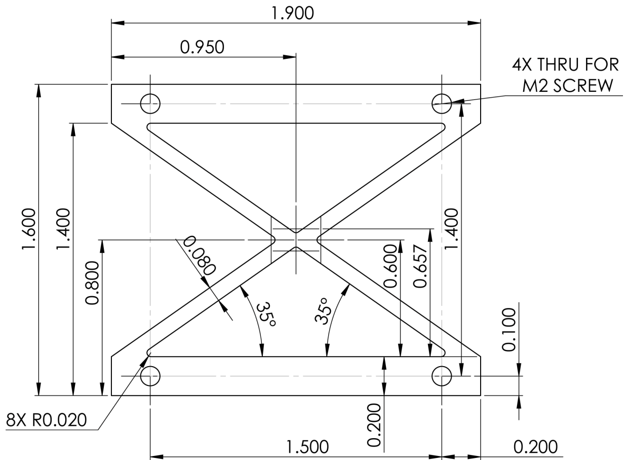
Figure D.6: Ti 15-3-3-3 X-frame fabrication drawing. Dimensions are in inches.
