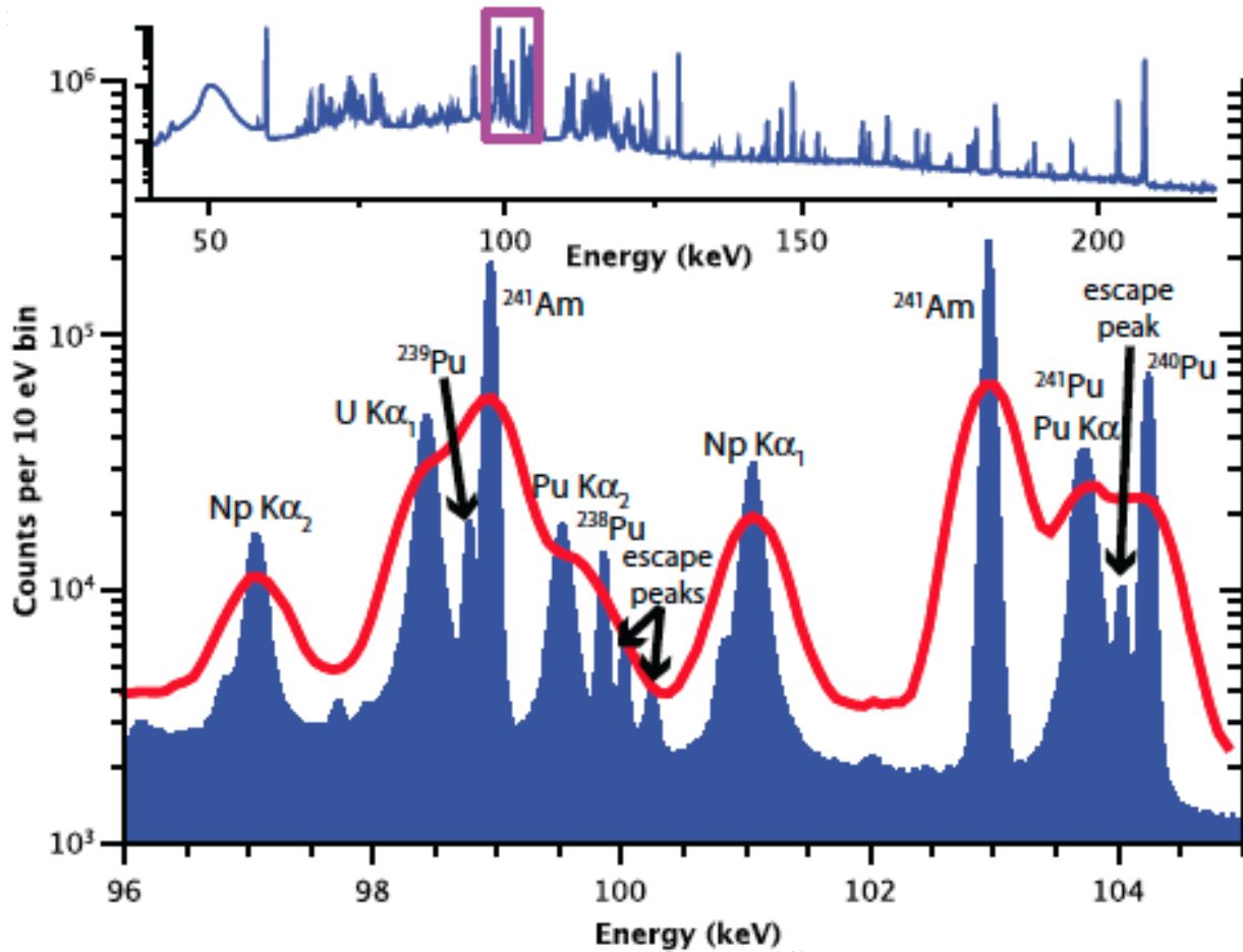
Figure 8.3: Gamma ray spectrum of \sim 0.4 g of ^{239}\text{Pu} + ^{240}\text{Pu} from 40 keV to 220 keV (inset) as measured by the microcalorimeter array developed by [30] (blue) and a leading edge HPGe detector (red). Data is magnified in the the 100 keV region. The proposed detector would produce an spectrum competitive with the microcalorimeter array. Image taken from [30].
