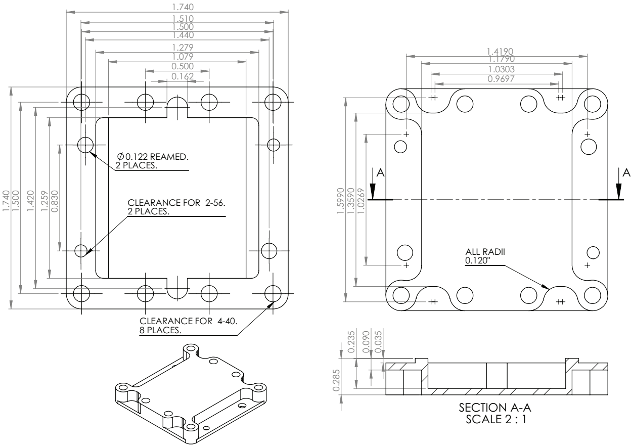
Figure D.3: KIDs test box top fabrication drawing. Dimensions are in inches.
