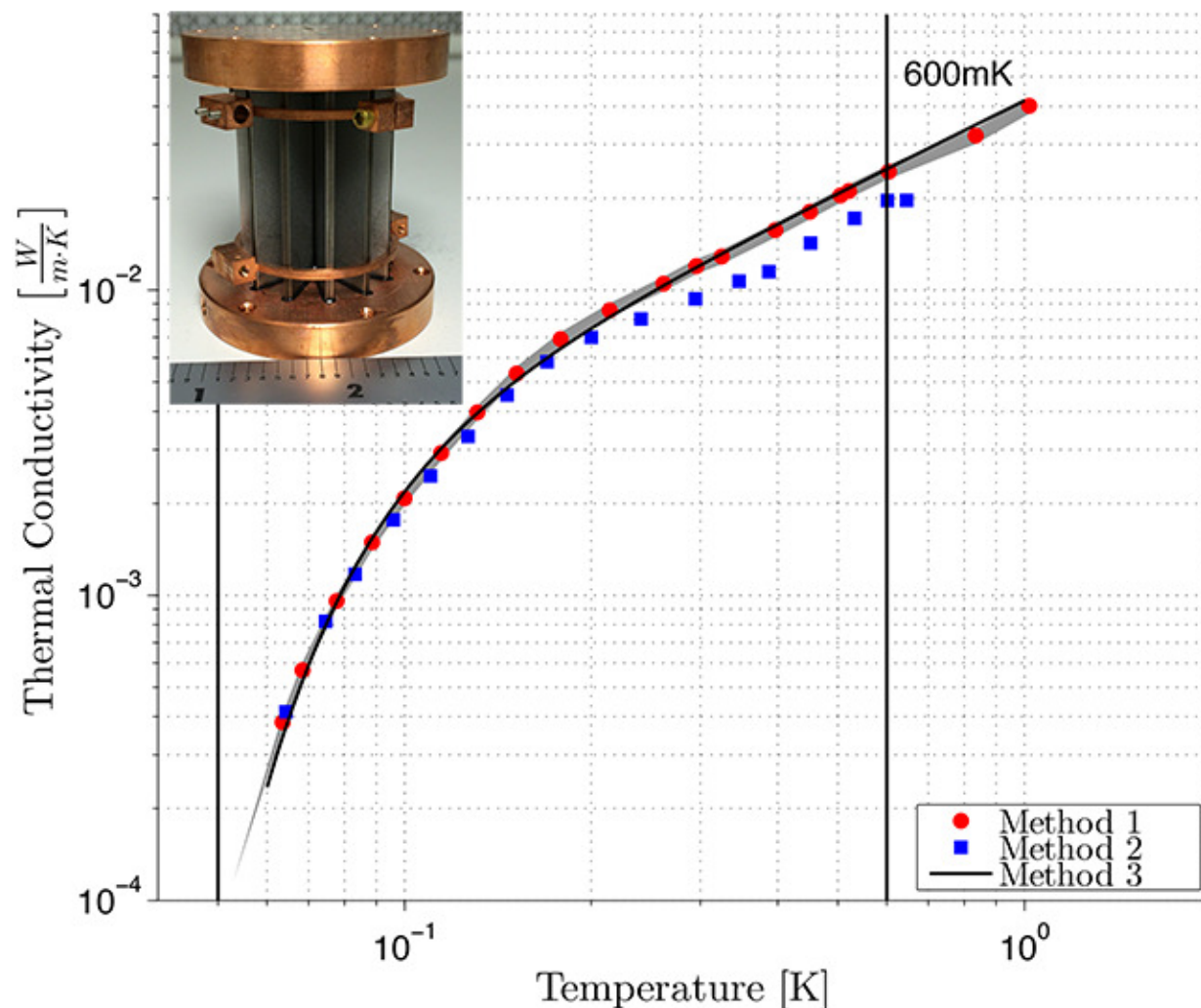
Figure C.15: Thermal conductivity of Nitinol alloy. Specimen in plate form and superelastic at room temperature.
