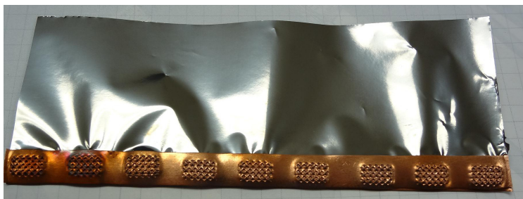
Figure 7.27: An attempt to join a copper foil to a Ti 13-3-3 foil by ultrasonic welding. The tool head is waffle patterned for focused ultrasonic contact. Weld attempts using fine patterned ultrasonic tool heads were unsuccessful. Process parameters, including the coarseness of the tool head, were dialed up until a successful weld was made. The welded foil, however, is unusable due to the deep waffle pattern imparted by the weld.
