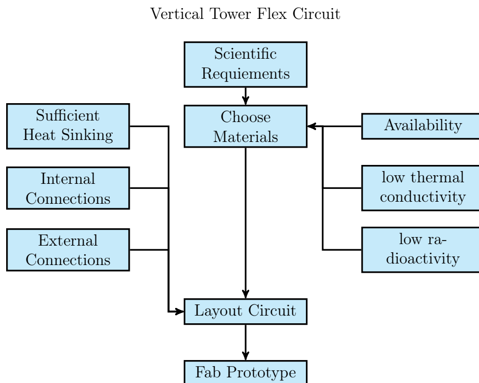
Figure 7.14: A flow chart representing the considerations and steps involved in designing the tower flex cable for the SuperCDMS SNOLAB experiment.
