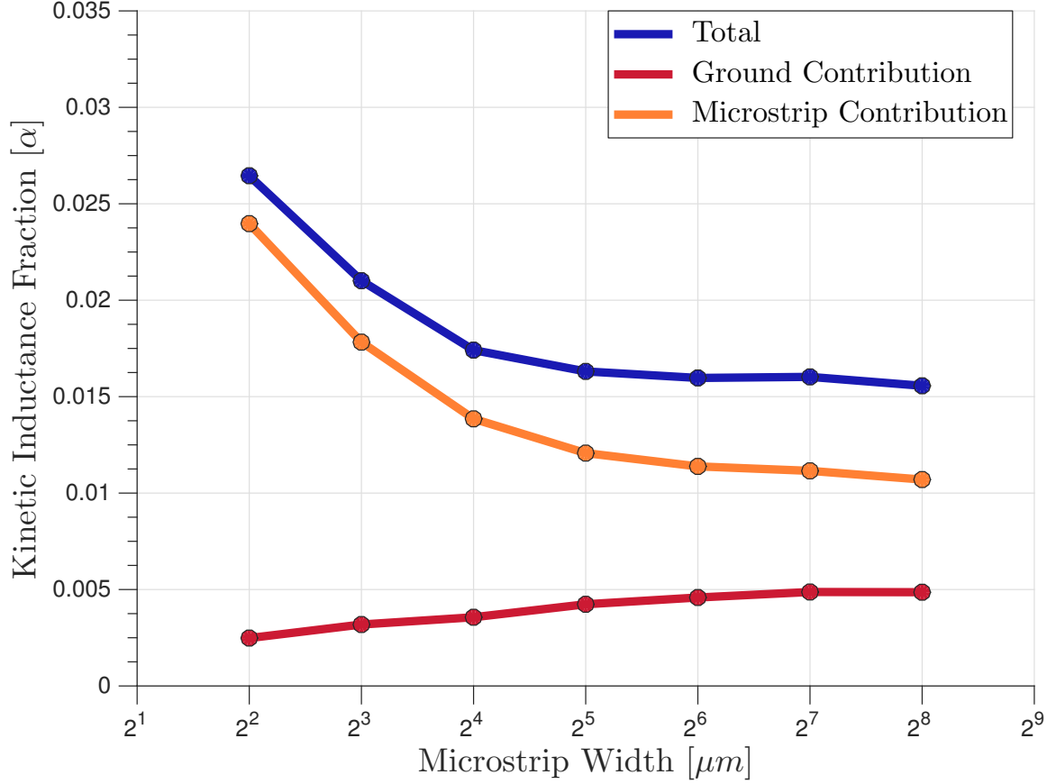
Figure 5.2: We use the procedure described in § 5.3 to calculate the kinetic inductance fractions for the sensor chips on the current test mask, calling out the contributions from the trace and the ground plane. We assume local and dirty electrodynamics; ground plane thickness 300 nm; ground plane penetration depth 39 nm; trace thickness 200 nm; trace penetration depth 16 nm; gap height 3000 nm. These values are also included in Table 5.1.
