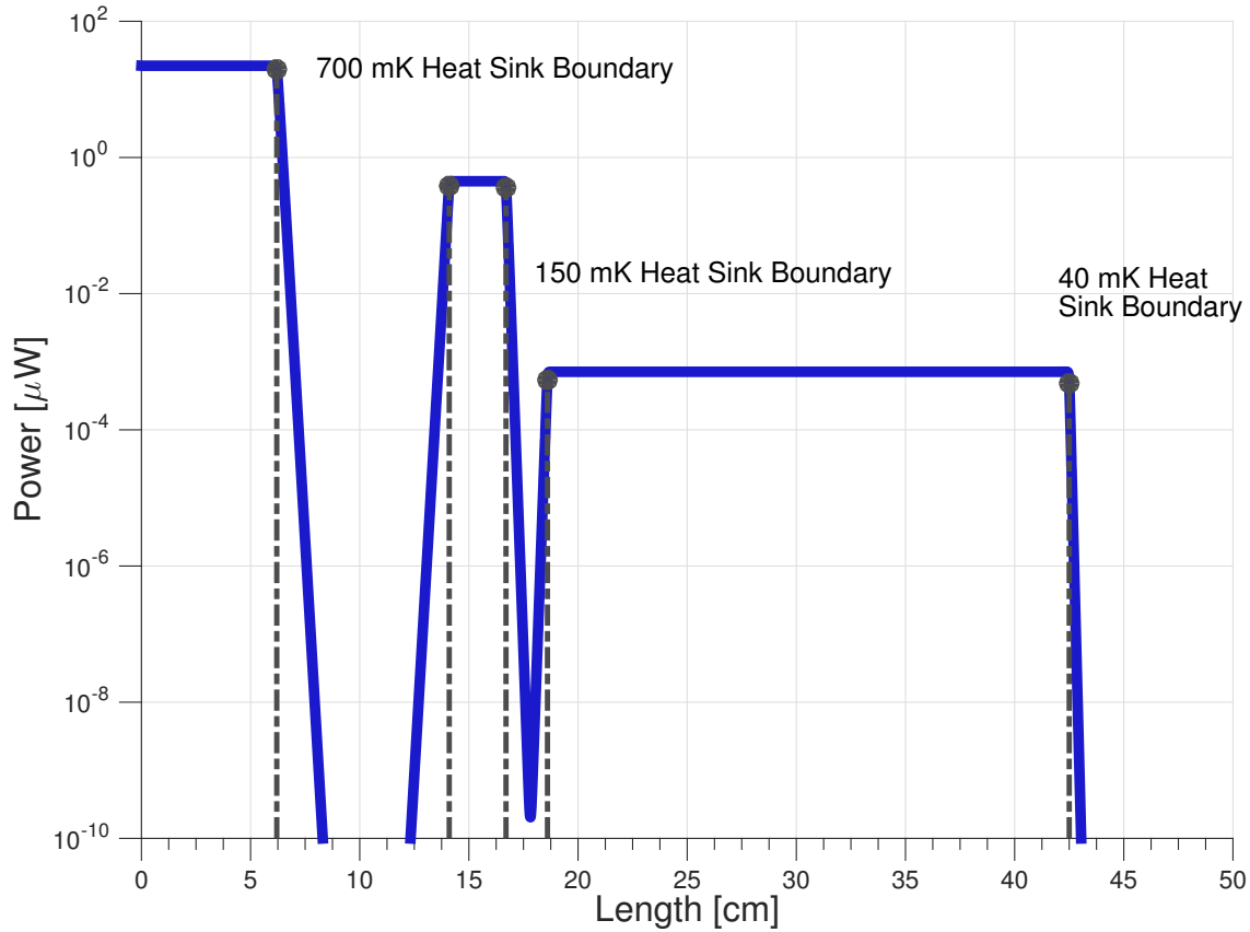
Figure 7.34: The thermal power profile of phonon cable. The power flow is constant in the insulated portions of the cable, but drops rapidly to toward zero in the heat sink portions of the cable. Power flows out of the heat sinks and into the cable at the cold end of each heat sink.
