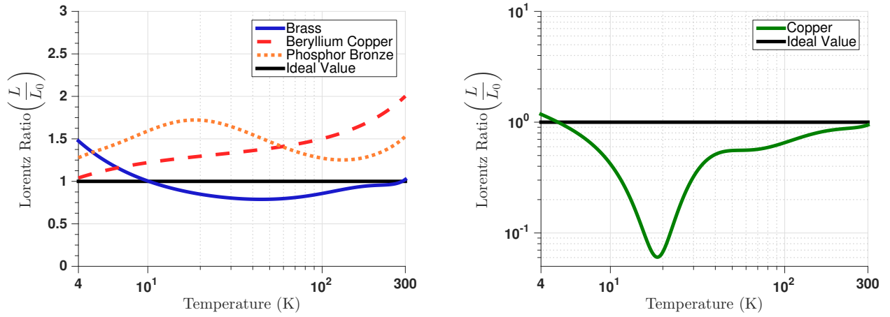
Figure 7.2: Temperature and material dependence of Lorenz number used in the Wiedemann-Franz-Lorenz law. Ideally the number should be temperature and material independent. However we observe significant temperature variation. This underscored the necessity to use measured values of thermal conductivity when making heat conduction calculations. Copper is presented by itself due to larger temperature variation in its Lorenz number. Data from [93]
