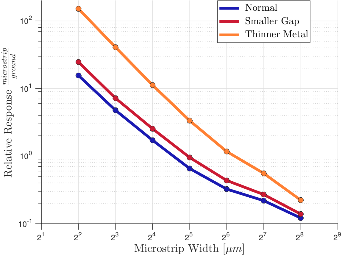
Figure 5.10: The response, |\delta S_{21}| , to quasiparticles in the microstrip trace relative to quasiparticles in the ground plane using probe chips “S2” through “S8” as radiation detectors. We also show the effect on the relative response which the use of a smaller gap and thinner metal would have. Taking the dimensions called out for Figure 5.2 as a baseline, the smaller gap is ten times smaller than baseline, and the thinner metal is ten times thinner than baseline.
