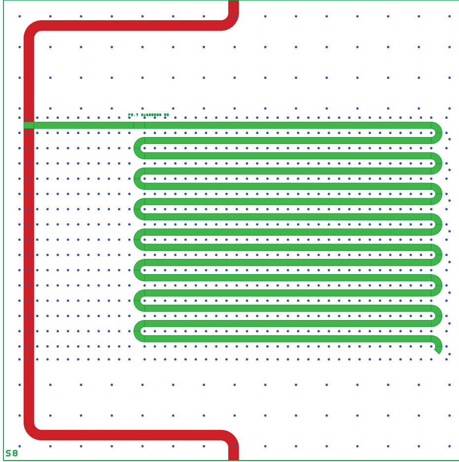
Figure 5.1: Lithography mask pattern for sensor chip “S8”. Each of the three colors represents a different mask layer. The pillars are in blue. The resonator is in green and the feedline is in red. The pillars and the resonator are on one side of the wafer and the feedline is aligned to them on the other side of the wafer. In interspersions of pillars within the meandered area of the resonator is an important design feature which prevents the resonator trace from shorting to the ground plane. When fabricated, the resonator and feedline traces are made of niobium.
