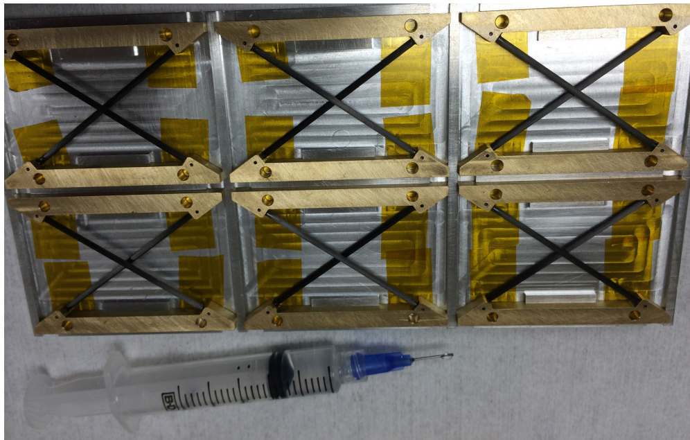
Figure D.8: Graphlite rod X-frame fabrication drawing and gluing fixture. Dimensions are in inches. The rods are cut to 2.221 inch long by \varnothing 0.02 inch (nominal stock diameter). Stycast 1266 epoxy is applied into holes using a syringe. X-frame base is made of copper (in the SNOLAB experiment) or brass.
