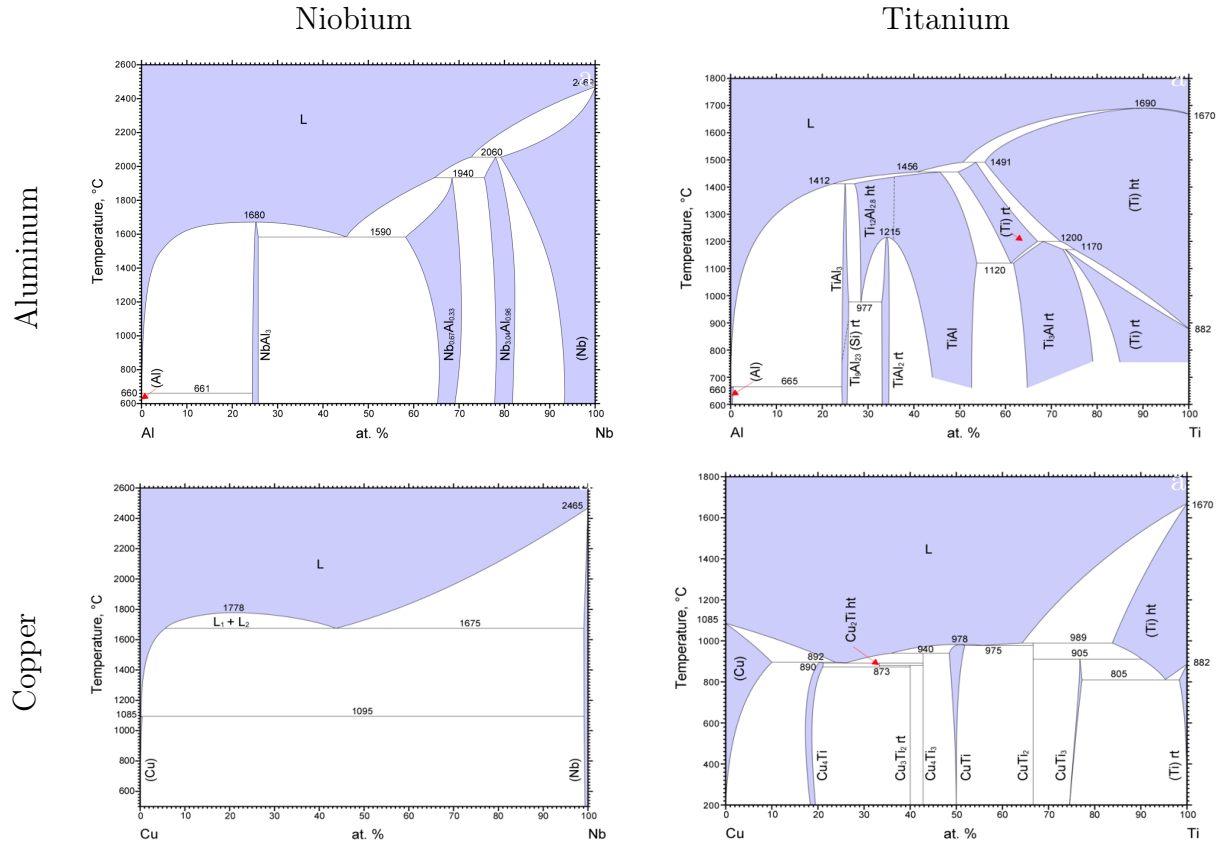
Figure 7.19: Equilibrium binary phase diagrams for: Nb-Al (1990 Kattner U.R.; exp.), Ti-Al (2006 Schuster J.C.; exp.), Nb-Cu (1984 Terekhov G.I.; exp.) and Ti-Cu (1996 Kumar K.C.H.; calc) from [1]. Diagrams are either calculated (calc.) or experimentally determined (exp.). We immediately notice the at Nb-Cu are immiscible. Ti-Cu forms several intermetallic compounds, while Ti-Al and Nb-Al form solid solutions.
