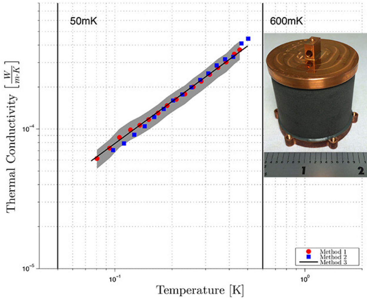
Figure C.16: Mersen 2020 Graphite thermal conductivity. Heat is directed perpendicular to grain.
