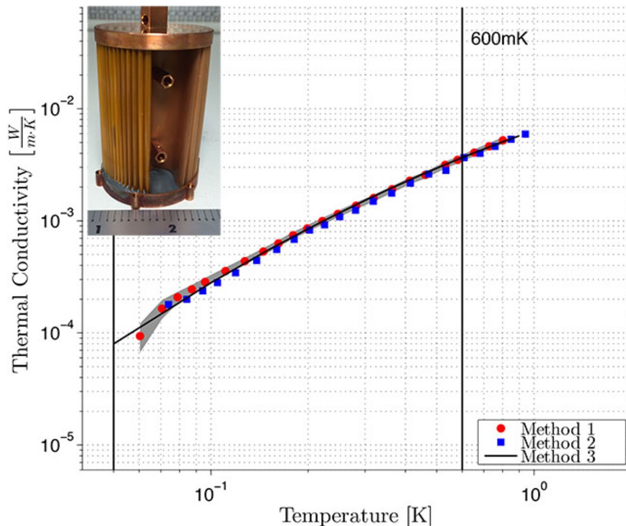
Figure C.3: Nikaflex CISV thermal conductivity.
