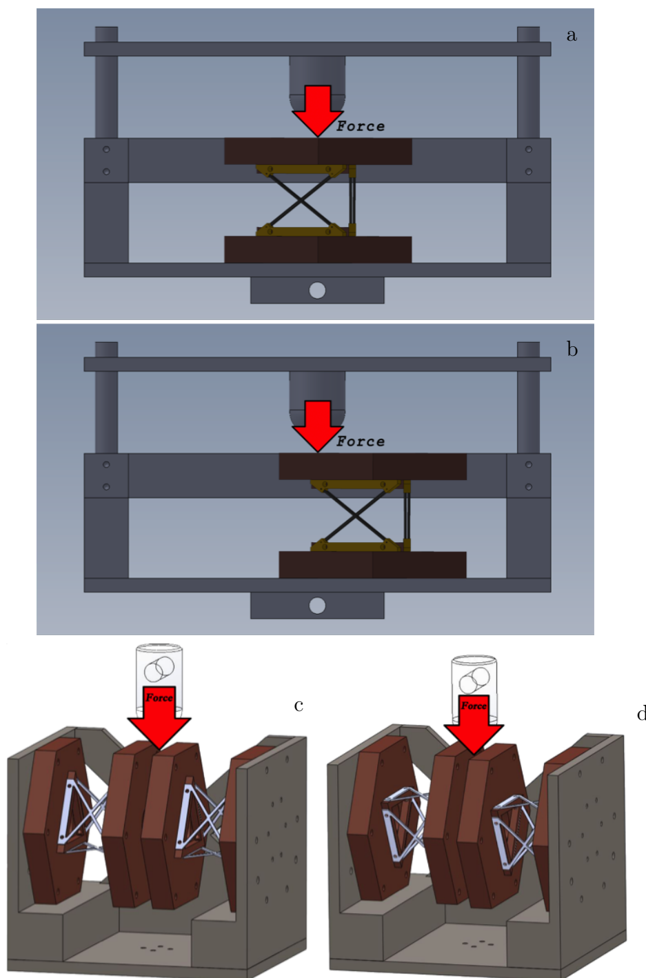
Figure 7.13: Loading conditions for the tower standoff mechanical testing. a – on axis compression, b – off axis compression, c – bending point up, d – bending point down. Adjustments are made to the data to correct for the weight of the press, in the case of the compression test frame, and the factor two multiplier from the symmetric module arrangement, in the case of the bending test frame.
