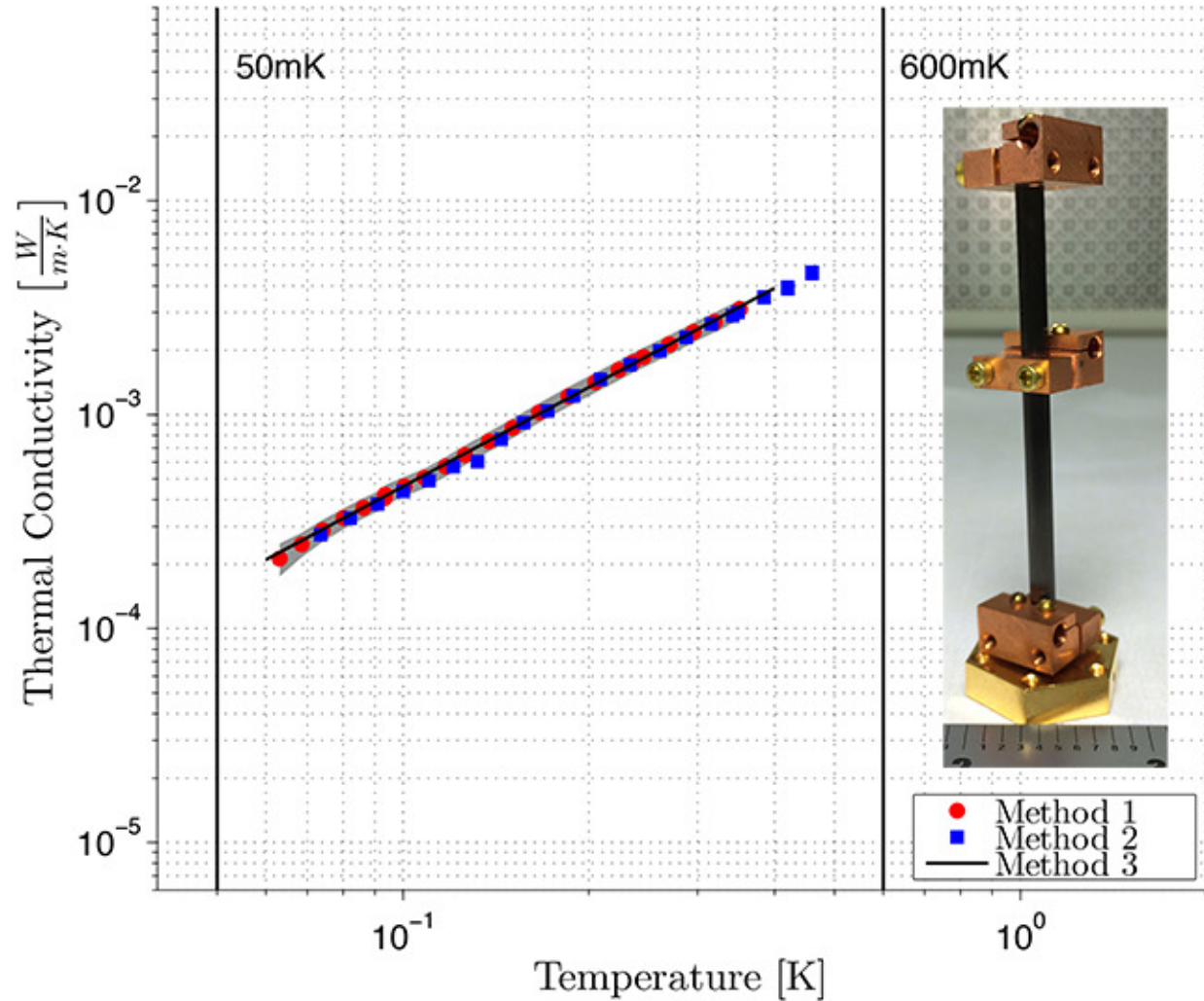
Figure C.18: Graphite CFRP thermal conductivity.
