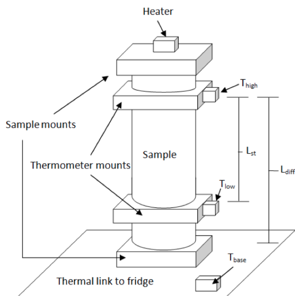
Figure C.1: This is a typical set up for our thermal conductivity measurement. This apparatus is placed inside of a 75 \mu\text{W} helium dilution refrigerator.
