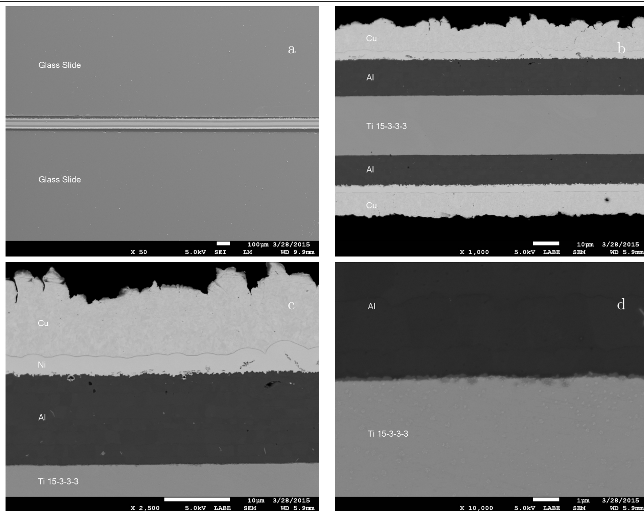
Figure 7.26: SEM micrographs of Ti 15-3-3-3 foil plated on both sides with aluminum via ion vapor deposition, and then electroplated copper. In order to promote copper adhesion, the aluminum surface was lightly etched, then zincated, then a thin layer of electroless nickel was applied. There should only be a few atomic layers of zinc, so it should not be visible in the micrographs. The bare Ti 15-3-3-3 foil is approximately 0.00084 inch thick. The plated samples are epoxied between two glass slides and then the stack is polished to expose the metal layers. No heat treatment on the plated sample was used. View magnification increases from view a to d .
