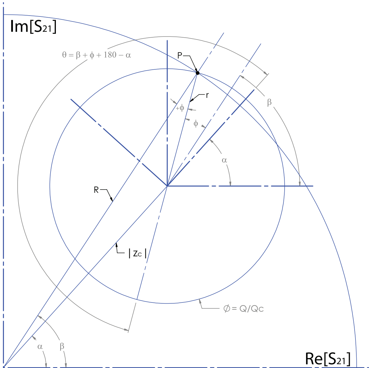
Figure 6.3: Angle and distance relationships for a resonance loop that has a rotation of +\phi is diagrammed. Note that the \phi rotation amounts to pivoting the loop at the point, P , where an unrotated resonance loop would tangentially intersect the outer loop. As depicted, the rotation can make a part of the resonance loop cross outside of the outer loop. This is the reason why some resonances, when plotted in magnitude frequency space, can have an upturn on one side of the dip.
