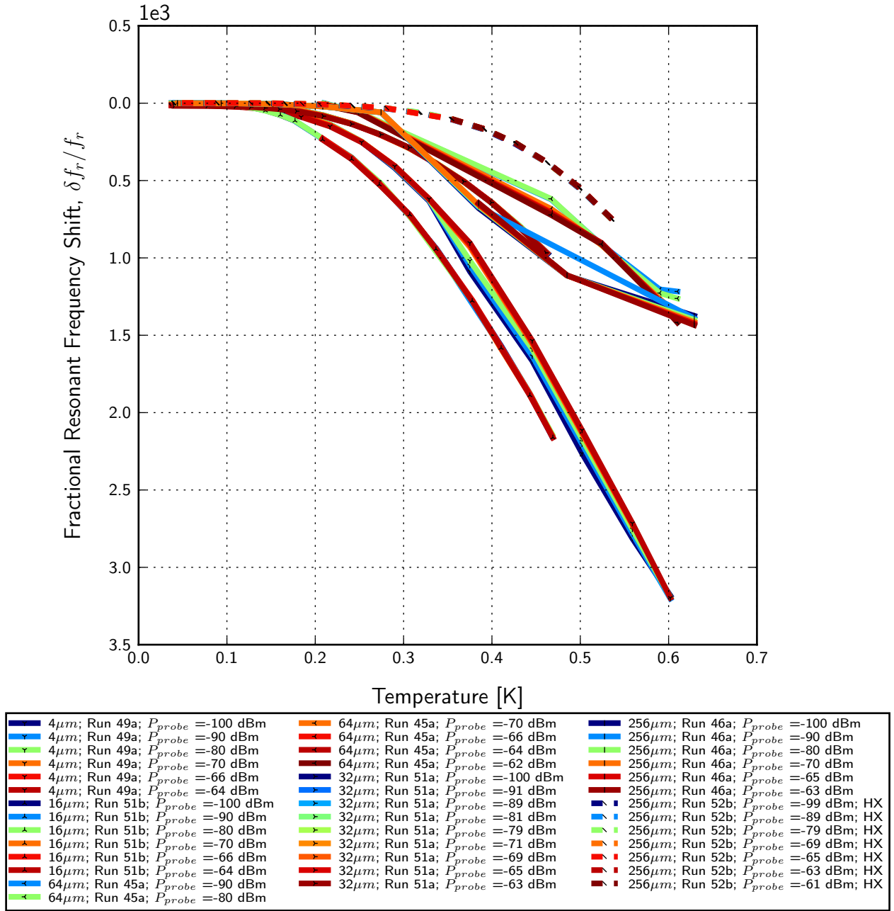
Figure 6.9: Fractional frequency shift versus probe power and temperature. Data run, microstrip trace width ( \mu\text{m} ) and ground plane thickness (nm) are specified in legend. Abbreviations are: CB – copper box (otherwise niobium box), TQ – under-torqued press, HX – hexagonal mesh ground plane.
