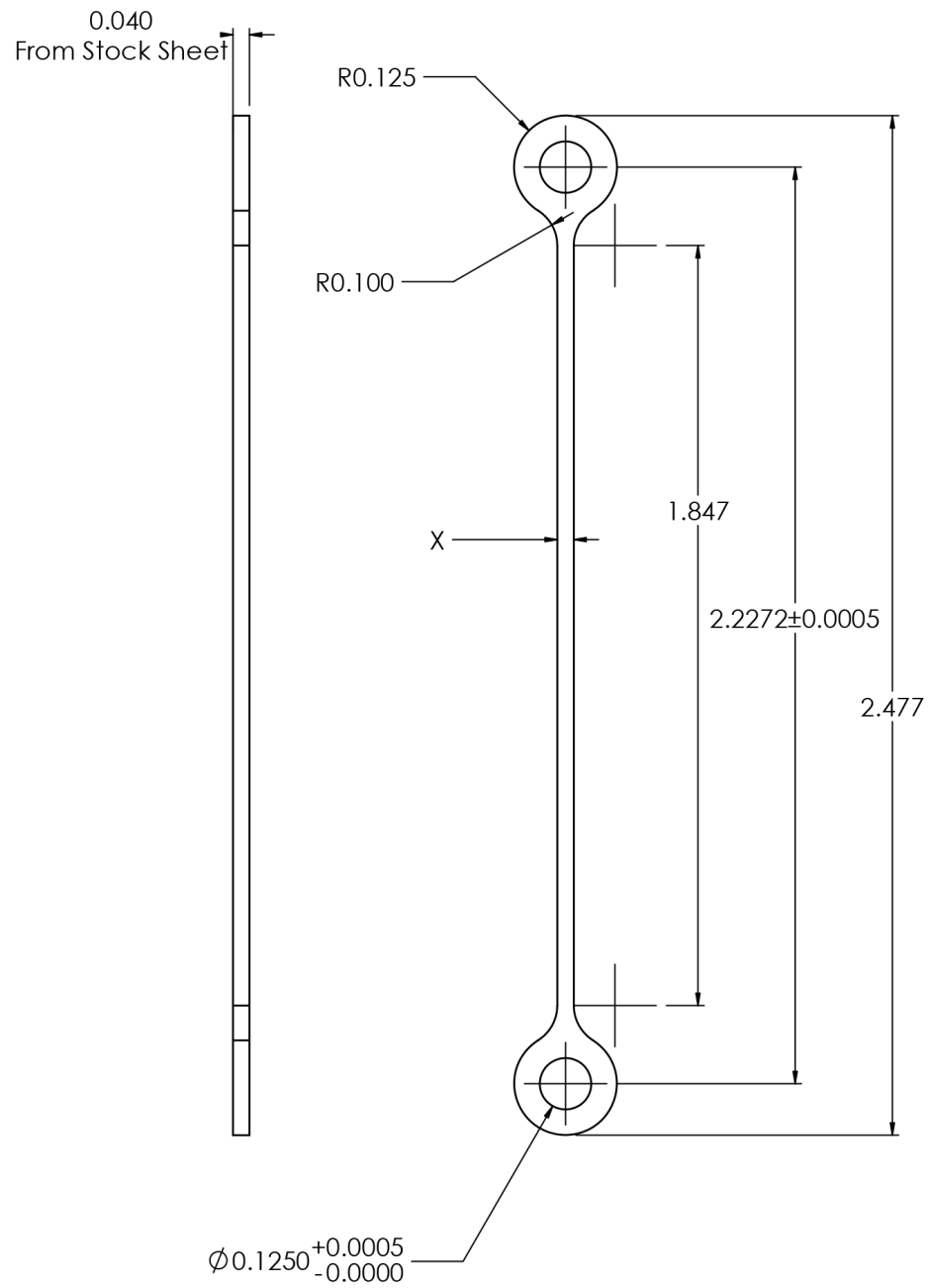
Figure D.7: Ti 15-3-3-3 hexipod member fabrication drawing. Dimensions are in inches. The dimension X is either 0.06 inch or 0.04 inch
