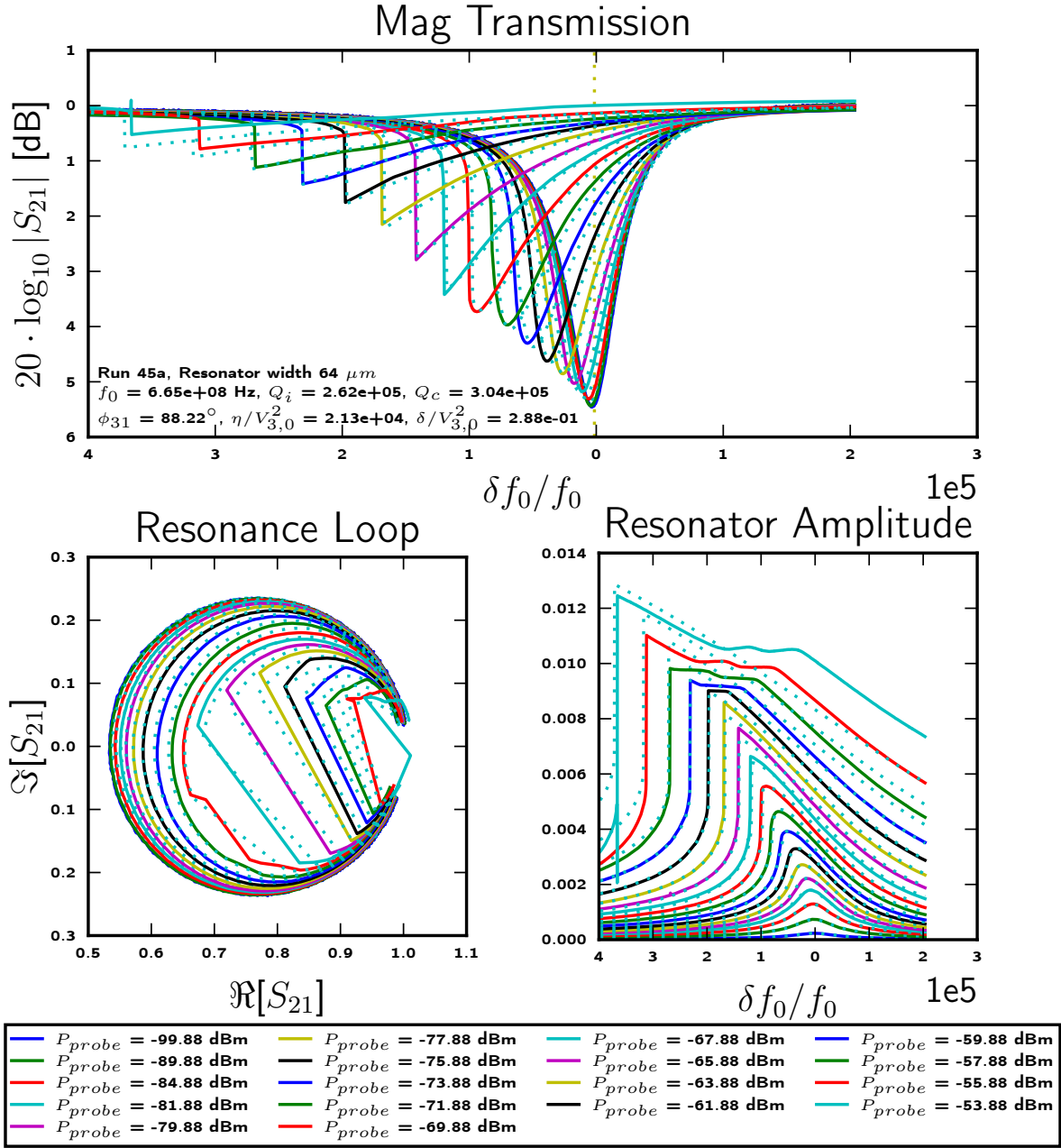
Figure 6.12: Fit to power sweep of Run 45a, a 64 \mu m resonator, as it becomes nonlinear. Dotted lines indicate the fit and the legend calls out the probe powers. Transmission magnitude (top), resonance loop (lower left) and the amplitude at the input of the resonator (right) are plotted. This is the same run from which the data in Figure 6.1 came. \delta f_0 / f_0 uses f_0 for the lowest power resonator as fit with the stepwise procedure for linear resonators. The vertical yellow dotted line is drawn at the resonant frequency determined by the nonlinear fit.
