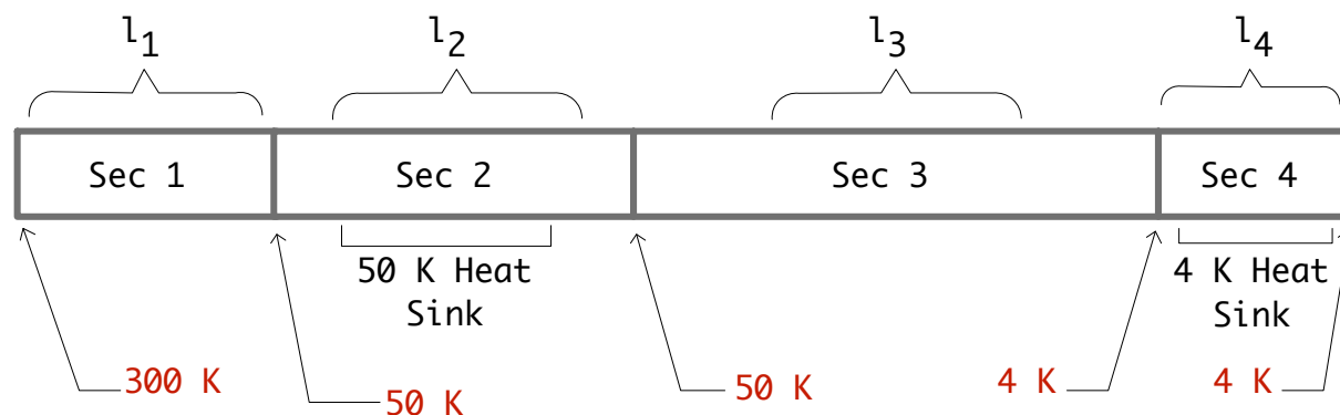
Figure 7.35: Block diagram of 4 K to 300 K cable. Section one and three are a low thermal conductivity trace material; sections two and four are copper. Section two is a circuit board that is heat sunk on its top and bottom faces. There is a heat sink in section four, but its dimensions are not determined. Approximate lengths are as follows: l_1 = 20\text{--}25 inch, l_2 = 3.5\text{--}10 inch, l_3 = 255\text{--}283 inch, and l_4 = 12\text{--}36 inch.
