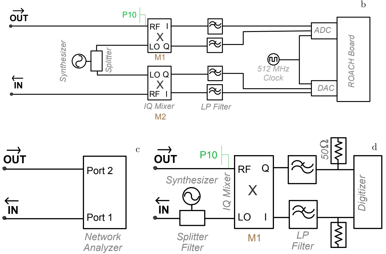
Figure 5.7: KIDs readout system configurations used to measure data. The three “digitizer end” configurations of the system are diagrammed. b – Readout system based around the ROACH reconfigurable computing platform [159]. This is a work in progress and used infrequently. c – Readout system based around an Agilent vector network analyzer. This configuration is used to perform temperature and power sweeps. d – Readout system based around a National Instruments 6120 digitizer. This configuration is mainly used to measure noise. Also splitters, filters and mixers are passive components. The \overleftarrow{\text{IN}} and \overrightarrow{\text{OUT}} ports of a and connected to the \overleftarrow{\text{IN}} and \overrightarrow{\text{OUT}} ports of b , c , and d to utilize any of those configurations. (continued from page 121)
