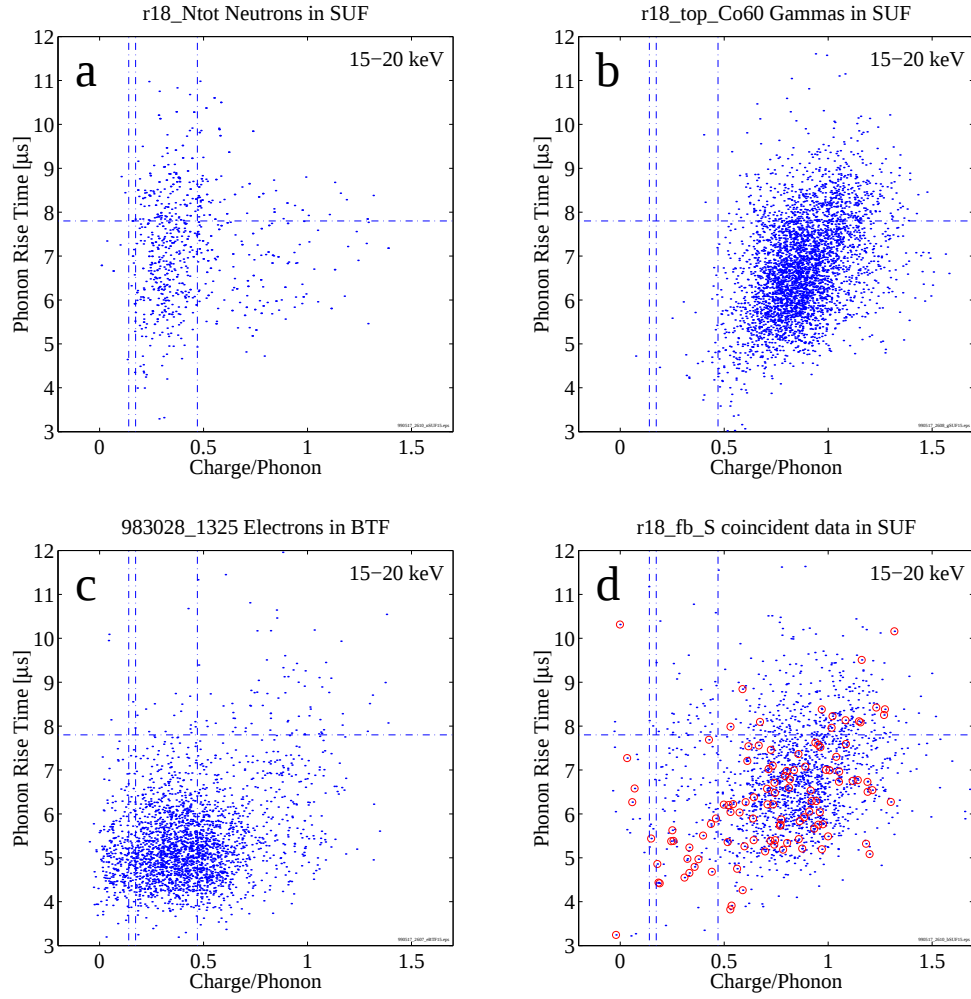
Figure 6.9: 4 sets of phonon rise time vs. Q/P 15–20 keV. The optimal phonon rise time cut is 7.8 \mu\text{s} , the optimal Q/P value is 0.5. \beta_r = 0.02 and \beta_y = 0.002 . The total efficiency for this energy range is 17%. Note: a) Neutron calibration run in SUF with a ^{252}\text{Cf} source; b) Photon calibration in SUF with a ^{60}\text{Co} source; c) Electron calibration in BTF with a ^{14}\text{C} and an ^{241}\text{Am} source; d) Low background data with muon anti-coincident events highlighted with small circles.
