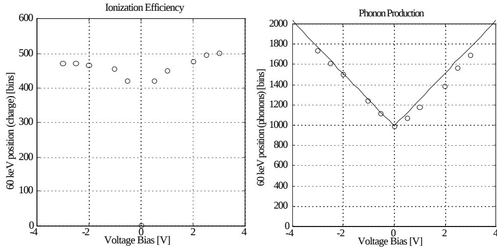
Figure 5.5: A plot of the positions of 60keV events measured by the ionization and phonon peaks vs. applied voltage. The plot on the left shows that the ionization efficiency does not degrade until V < 2 . On the right, the phonon peak increases with applied voltage as one would expect if the absorption coefficient were equal for intrinsic and 'Luke' phonons. These data were taken in a previous calibration run performed without an electron source.
