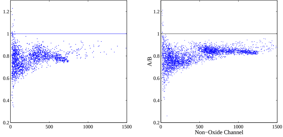
Figure 7.7: The signal height ratio of oxide over non-oxide versus height in non-oxide sensor for 0 volts (left side) and 3 volts (right side). The smear in the 60 keV photons is from down conversion of phonons in the perimeter metal layer.
