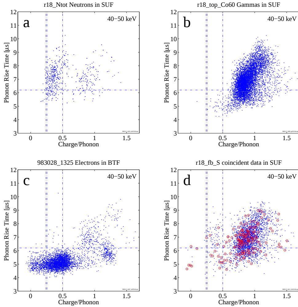
Figure 6.6: 4 sets of phonon rise time vs. Q/P 40-50 keV. The optimal phonon rise time cut is 6.2 \mu\text{s} , the optimal Q/P value is 0.5. \beta_r = 0.03 and \beta_y = 0.001 . The total efficiency for this energy range is 44%. Three events survive all cuts in this energy range. Note: a) Neutron calibration run in SUF with a ^{252}\text{Cf} source; b) Photon calibration in SUF with a ^{60}\text{Co} source; c) Electron calibration in BTF with a ^{14}\text{C} and an ^{241}\text{Am} source; d) Low background data with muon anti-coincident events highlighted with small circles.
