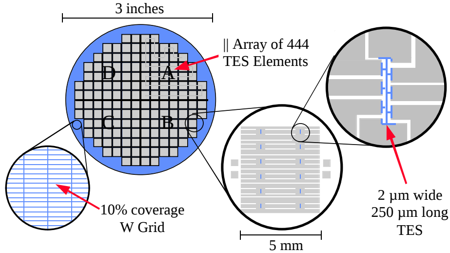
Figure 3.1: A diagram of the phonon sensor side of the Alex design. The surface is divided into active area and an outer W grid. The active area consists of 4 independent readout channels each composed of 37 - 5 X 5 mm individual dies. Each of the dies has 12 QET elements each leading quasiparticles to a 2 \mu\text{m} wide W TES.
