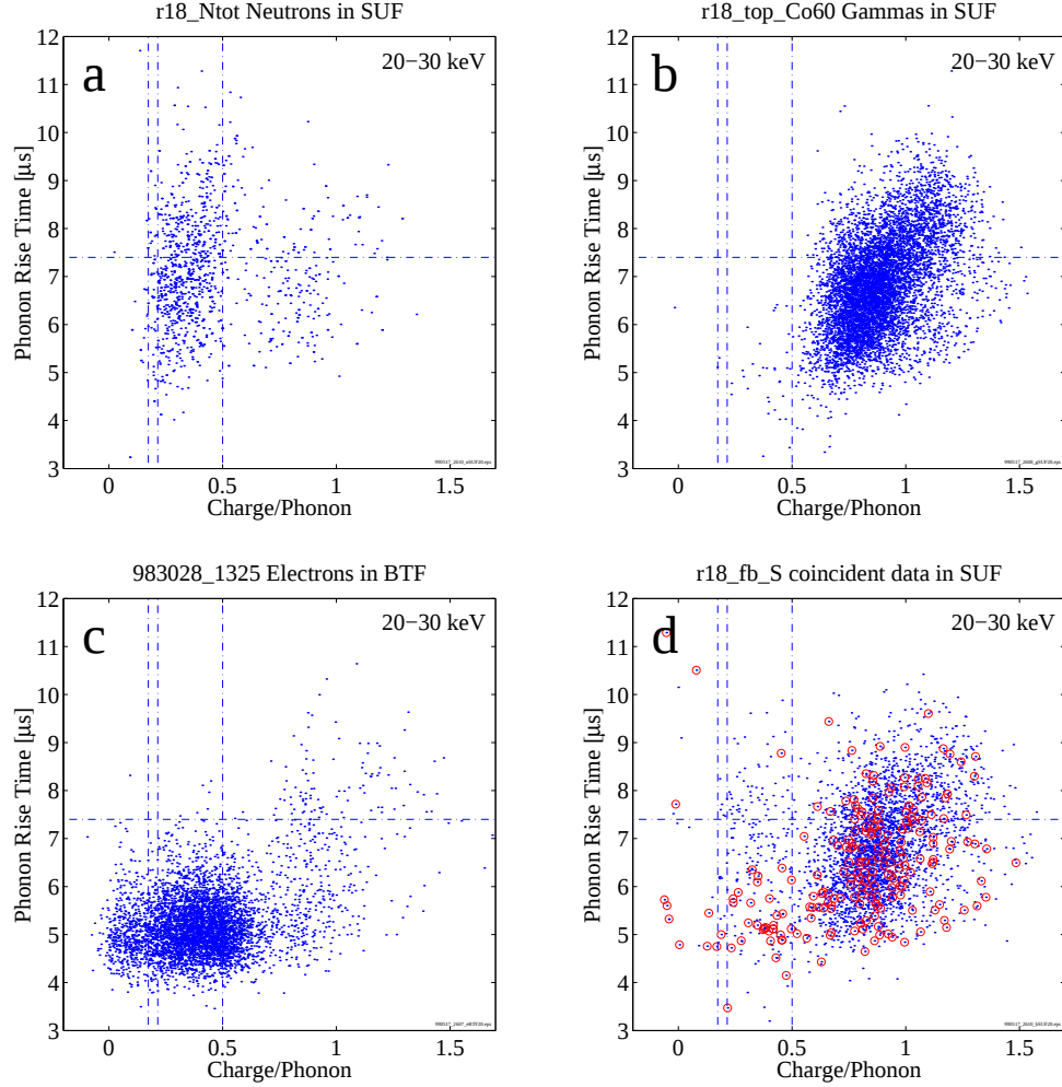
Figure 6.8: 4 sets of phonon rise time vs. Q/P 20-30 keV. The optimal phonon rise time cut is 7.4 \mu\text{s} , the optimal Q/P value is 0.5. \beta_r = 0.01 and \beta_y = 0.001 . The total efficiency for this energy range is 21%. One event survives all cuts as a possible signal candidate in this energy range. Note: a) Neutron calibration run in SUF with a ^{252}\text{Cf} source; b) Photon calibration in SUF with a ^{60}\text{Co} source; c) Electron calibration in BTF with a ^{14}\text{C} and an ^{241}\text{Am} source; d) Low background data with muon anti-coincident events highlighted with small circles.
