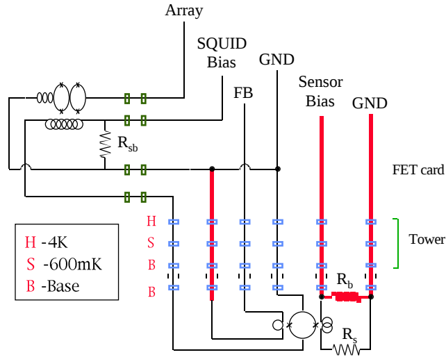
Figure 8.6: A circuit diagram of a two stage SQUID system for the tower geometry. Two feedback lines are now required: one active on the first stage single SQUID, and one passive on the array (to maintain the appropriate position on the V-Phi curve, the array feedback line is not shown). Note: double lines represent wires that are not repeated for each sensor. The total number of wires (from 4K to base) using this system and four phonon sensors would be 15.
