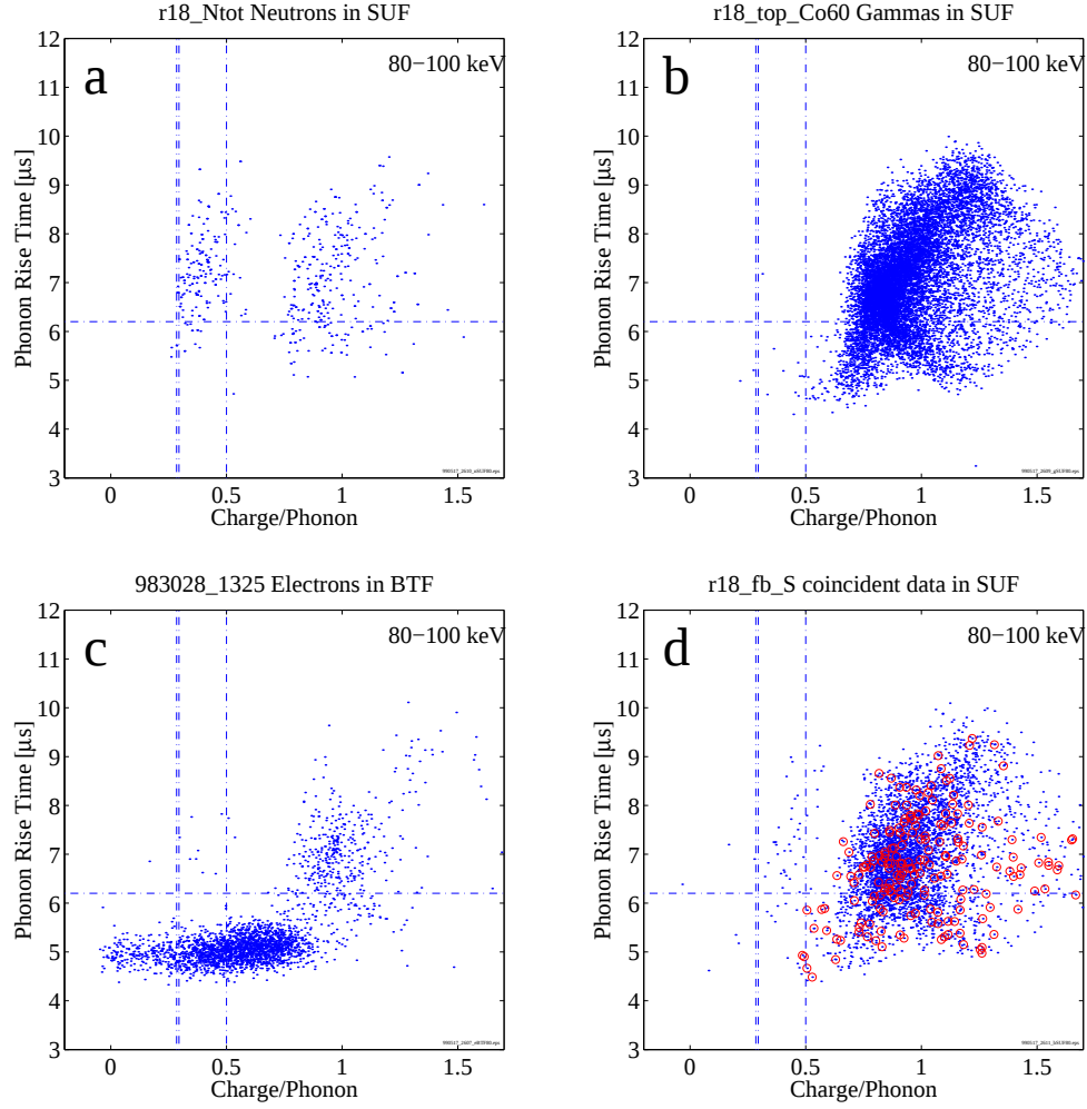
Figure 6.4: 4 sets of phonon rise time vs. Q/P 80-100 keV. The optimal phonon rise time cut is 6.2 \mu\text{s} , the optimal Q/P value is 0.5. \beta_r = 0.0640 and \beta_y = 0.001 . The total efficiency for this energy range is 48%. Note: a) Neutron calibration run in SUF with a ^{252}\text{Cf} source; b) Photon calibration in SUF with a ^{60}\text{Co} source; c) Electron calibration in BTF with a ^{14}\text{C} and an ^{241}\text{Am} source; d) Low background data with muon anti-coincident events highlighted with small circles.
