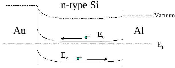
Figure 2.6: A band diagram of the silicon ionization system. The barrier on the aluminum side is significantly smaller than on the gold side.
