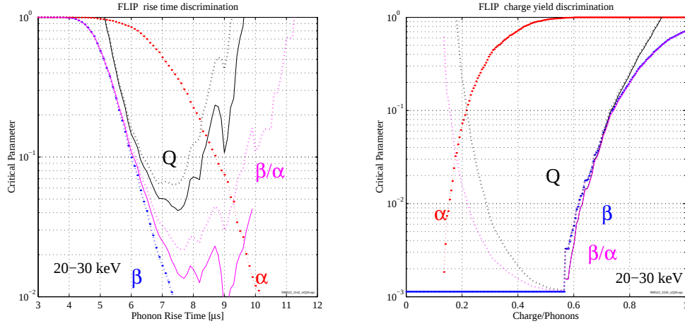
Figure 5.17: a) Phonon discrimination in the 20-30 keV range. b) Charge yield discrimination in the 20-30 keV range. Note that although the charge-based discrimination is an order of magnitude better than that of rise time at the same energy the combination of the two is more beneficial than either alone.
