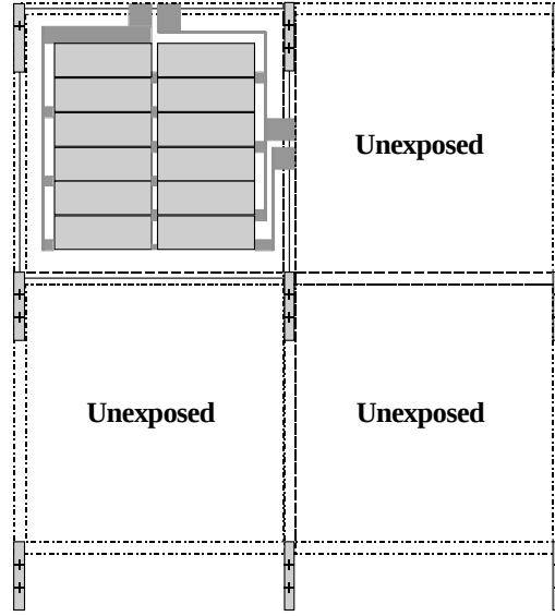
Figure 3.3: A diagram of a single 5 mm die. In order to achieve the 5 X 5 mm geometry we needed to fool the Ultrastep into thinking it was exposing over a 1 cm grid. Note: each alignment mark is simultaneously a left and right mark. The die shown is l_TRPad3. See text for an explanation of the different dies.
