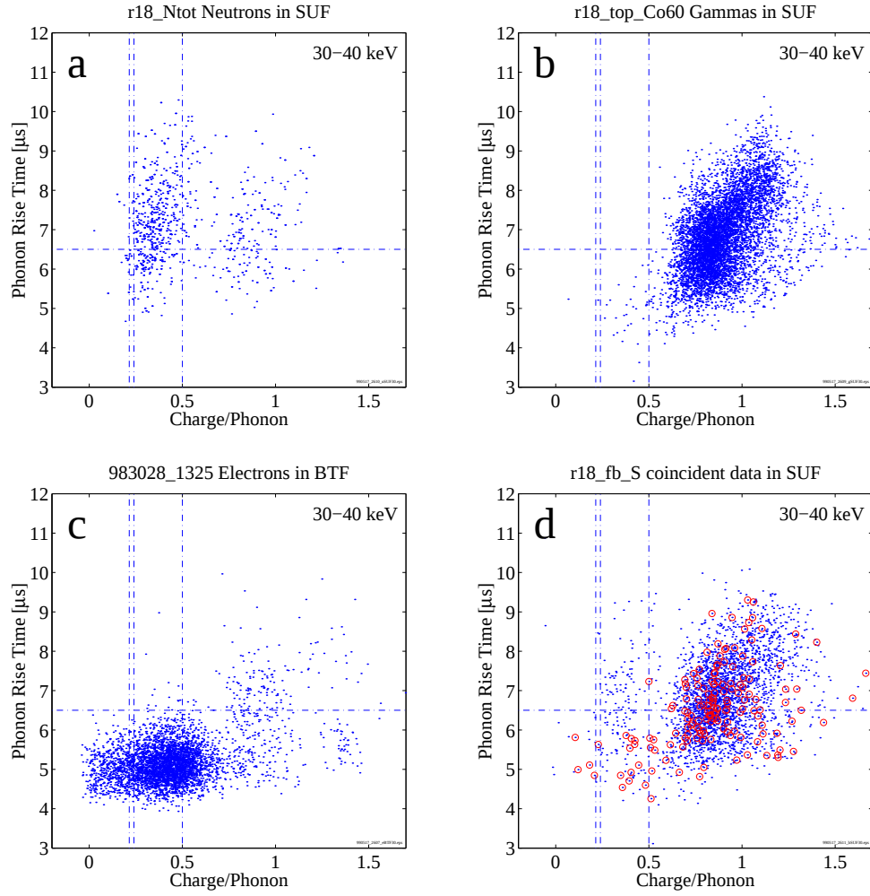
Figure 6.7: 4 sets of phonon rise time vs. Q/P 30-40 keV. The optimal phonon rise time cut is 6.5 \mu\text{s} , the optimal Q/P value is 0.5. \beta_r = 0.02 and \beta_y = 0.001 . The total efficiency for this energy range is 39%. Note: a) Neutron calibration run in SUF with a ^{252}\text{Cf} source; b) Photon calibration in SUF with a ^{60}\text{Co} source; c) Electron calibration in BTF with a ^{14}\text{C} and an ^{241}\text{Am} source; d) Low background data with muon anti-coincident events highlighted with small circles.
