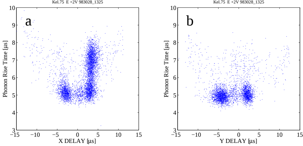
Figure 5.3: Phonon rise time versus delay in X (a) and delay in Y (b). The electrons appear at clearly lower phonon rise times ( \sim 5\mu\text{s} ) than the 60 keV photons.
