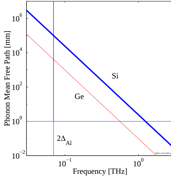
Figure 2.1: A plot of phonon mean free path versus phonon frequency for Silicon and Germanium. Vertical line is the 2\Delta_{Al} energy threshold. Horizontal line is at 1 mm. Taken from Wolfe [72]
