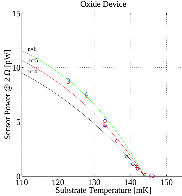
Figure 7.8: Plot of power dissipated vs. substrate temperature for one of the oxide sensors. Curves represent a T^4 , T^5 , and T^6 thermal conductivity dependence. At low powers ( T_s > 130 mK) a T^5 dependence appears to be the best fit.
