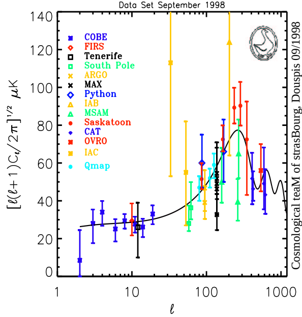
Figure 1.6: A summary of satellite and ground based observations of the power as a function of angular scale in the cosmic microwave background. The curve shown is for a \Omega_M = 0.2 \Omega_\Lambda = 0.8 universe. From astro-ph/9903260
