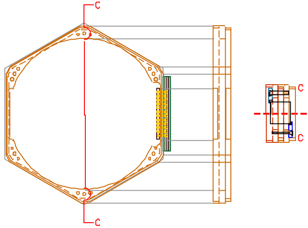
Figure 8.4: A design drawing of the new close-packed detector mount. MillMax sockets now are now in the same plane as the detector to save vertical space. To the right is a view of one face of the hexagon with an outline showing the height of a 1 cm detector.
