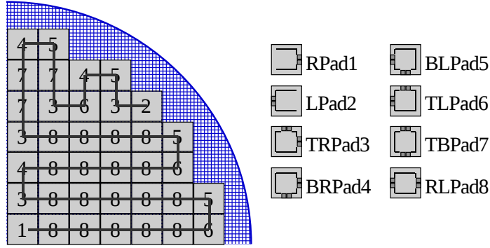
Figure 3.2: One channel of the phonon sensor side with interconnectivity pattern. Eight separate dies (shown on the right) are necessary to complete the snake pattern in each quadrant. The other quadrants are merely mirror images of these quadrants. Because of the limitations of the ultrastep1000 we are forced to double the number of masks to 16 (see Fig. 3.3).
