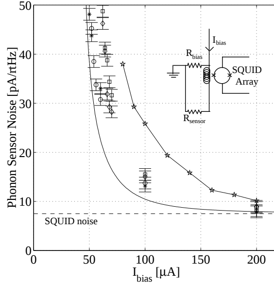
Figure 8.1: A plot of current noise density vs sensor current bias ( I_{bias} ). Data on the left (errorbars) show the measured noise spectral density of each of the 4 phonon sensors as a function of I_{bias} at 50 kHz. Solid curve is a noise prediction including only Johnson noise terms and the SQUID noise (dashed line). Stars show the height of the 60keV peak vs I_{bias} . Inset shows the QET phonon sensor bias circuit.
