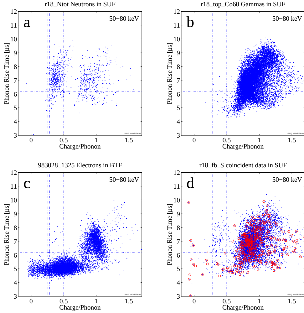
Figure 6.5: 4 sets of phonon rise time vs. Q/P 50-80 keV. The optimal phonon rise time cut is 6.2 \mu\text{s} , the optimal Q/P value is 0.5. \beta_r = 0.03 and \beta_y = 0.001 . The total efficiency for this energy range is 47%. Note: a) Neutron calibration run in SUF with a ^{252}\text{Cf} source; b) Photon calibration in SUF with a ^{60}\text{Co} source; c) Electron calibration in BTF with a ^{14}\text{C} and an ^{241}\text{Am} source; d) Low background data with muon anti-coincident events highlighted with small circles.
