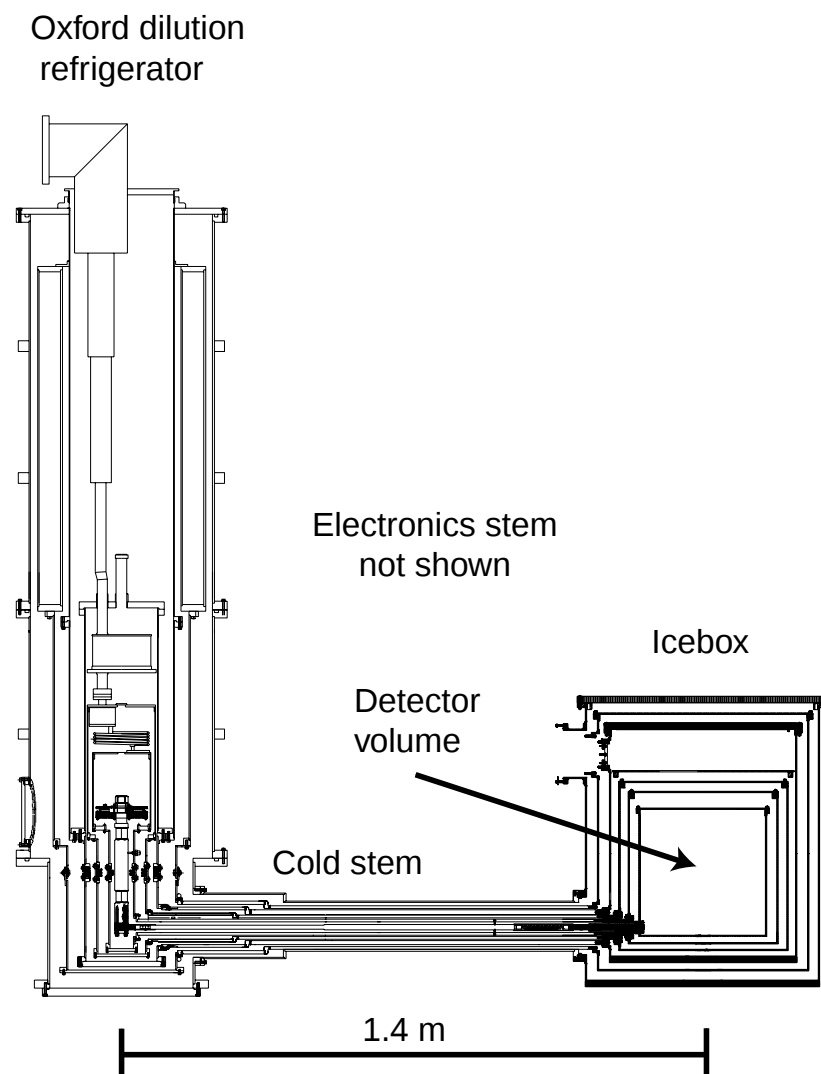
Figure 4.7: A diagram of the Kelvinox 400 dilution refrigerator, and the right-angle icebox assembly. Five concentric copper cylinders carry heat 1.4 m from a 30l cold box (detector volume). No cryogenics pass beyond the right angle joint. Wiring enters along an electronics stem through the top of the icebox. The distances between the temperature stages on the tower match those of the lids of the icebox.
