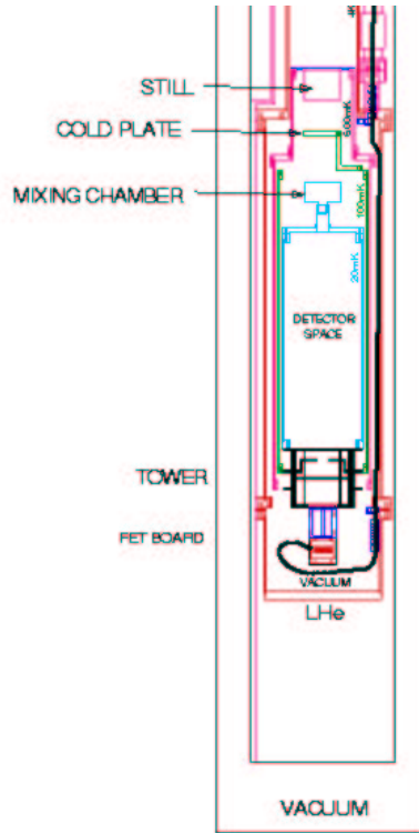
Figure 4.4: A diagram of the Berkeley 75\,\mu\text{W} dilution refrigerator modified to accept an inverted tower assembly. The temperature stages are inverted by a series of concentric copper cans similar to the icebox.
