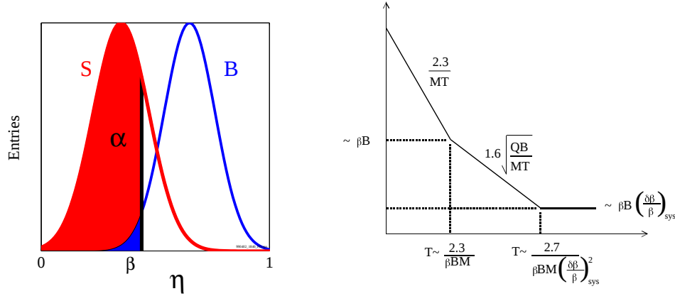
Figure 5.14: A diagram illustrating the background improvements obtained with discrimination. On the left is a cartoon showing the background distribution, B, the signal distribution, S, with \alpha and \beta , the acceptance and rejection factors as a function of an arbitrary cut parameter \eta . On the right is a plot of the upper limit in background rate vs. time. We gain linearly in time until a background is detected, then as the square root through subtraction. Subtraction ultimately fails due to systematic uncertainties.
