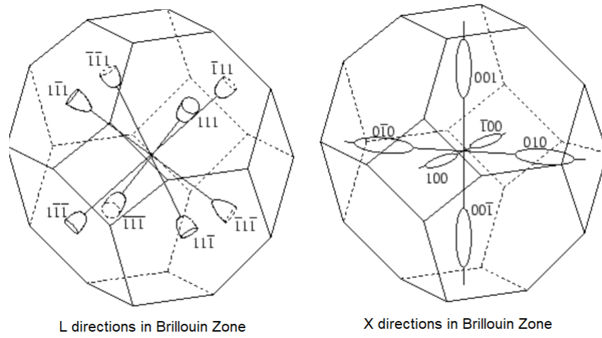
Figure 2.5: This figure shows a three-dimensional version of the same lattice in Figure 2.4, which allows us to see the full set of directional definitions. We show it because the directions defined by the Brillouin zone are useful for describing wave propagation. In the left figure, we show the directions along the edges of the Brillouin zone, which is defined as L = [111] along with its variations. The directions situated along the zone boundaries are known as the X = [001] , and are shown along with its variations in the right figure. The center of the Brillouin zone is known as \Gamma = [000] . Adapted from Ref. [35].
