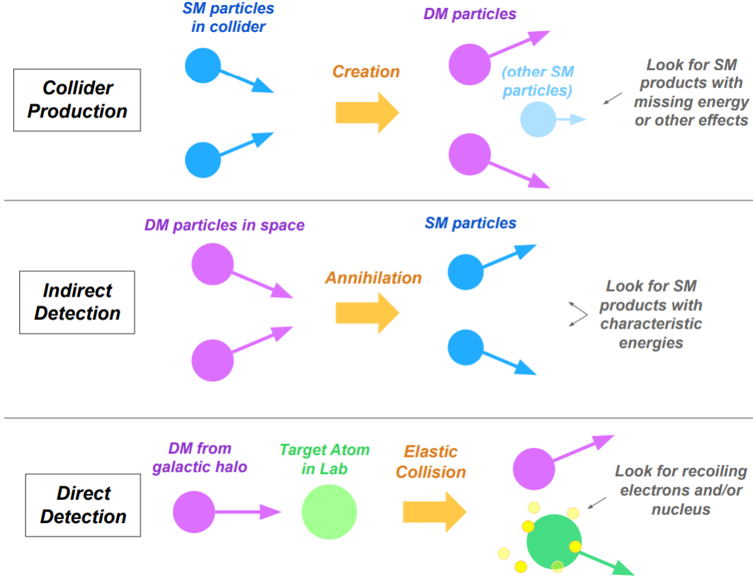
Figure 1.4: This figure shows a cartoon of the three primary experimental approaches to observe an interaction of the hypothesized dark matter (DM) particle. We show it because the work in this dissertation is designed to assist in the understanding of the detectors used in direct detection experiments (bottom row). The top row shows an experiment where two standard model (SM) particles collide with enough energy to produce dark matter particles. Typically, a large detector surrounds the collisions and compares observations to the hypothesis of standard model-only interactions [16]. The middle row shows the indirect detection method in which dark matter particles collide in outer space, annihilate, and produce high-energy final-state particles. Telescopes and other detectors compare observations of particle energies with predictions made only from the standard model [17]. The bottom row shows the direct detection method in which a dark matter particle interacts with standard model particles in a detector. Custom sensors on the detector volume compare observations from the hypotheses both with and without dark matter interactions [15, 18]. Reprinted from Ref. [19].
