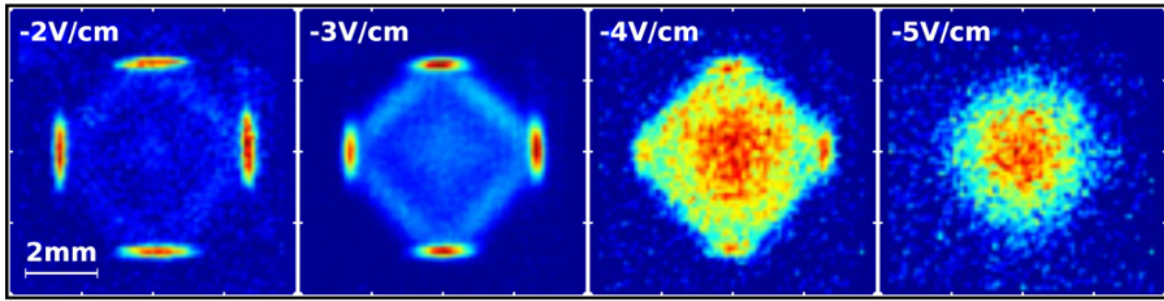
Figure 5.15: This figure shows a set of experimental results for the electrons' arrival positions in a high-purity germanium test device for four different voltages. We show it because the set of results allows for a visual comparison with the case simulated in G4CMP shown in Figure 5.12, as well as provides multiple points so we can extrapolate. We note that there are configuration differences between the experimental results and those shown in Figure 5.12. Specifically, the crystal used here is 3.89 mm thick with 10 mm \times 10 mm top and bottom faces, operating at 1 K with the valleys located at [\pm 1, \pm 1, 0] , [\pm 1, 0, \pm 1] , and [0, \pm 1, \pm 1] . Comparisons can be made by scaling and simple rotations, and we observe that the arrival points, the position of the corners, and the size of the whole shape match qualitatively. On the other hand, again, the density of electrons in between the bands is not the same for the same voltage, and future work, like in Ref. [64], is required to better parameterize the intervalley scattering rates in G4CMP. Reprinted from Ref. [34].
