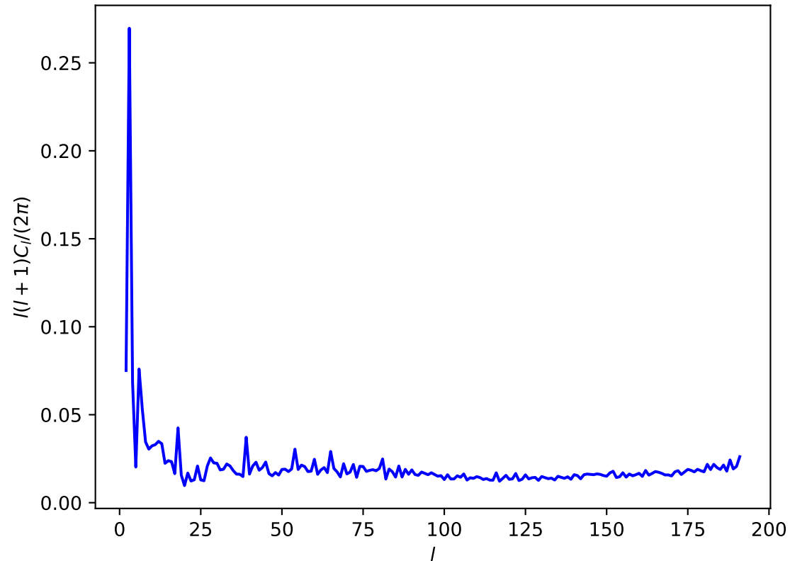
rolling10 z: CoaddM5
