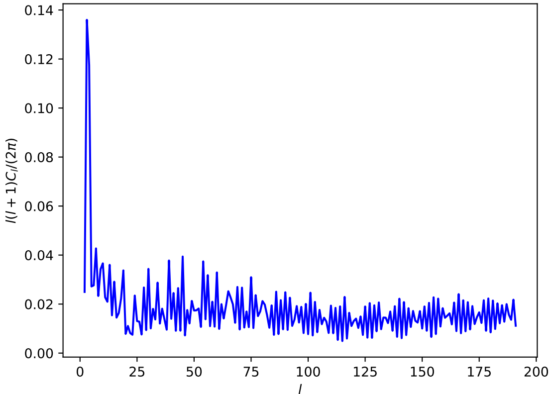
rolling10 y: CoaddM5
