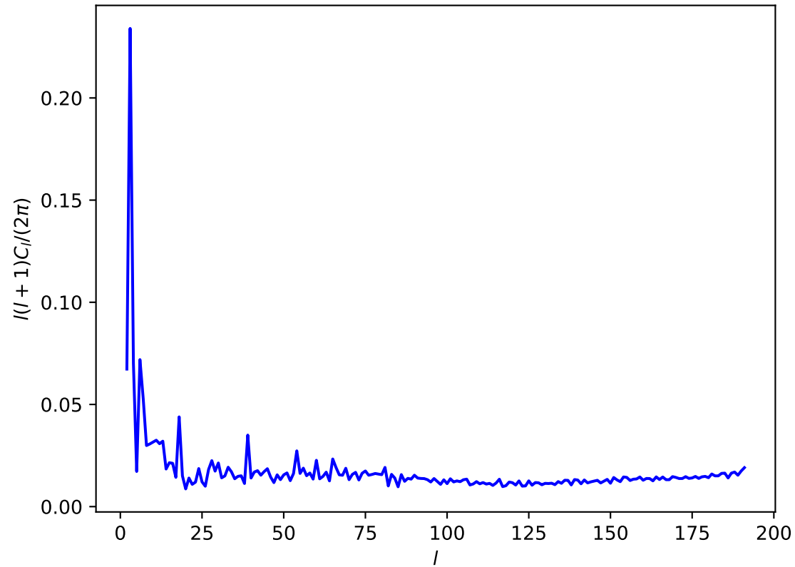
rolling10 r: CoaddM5
