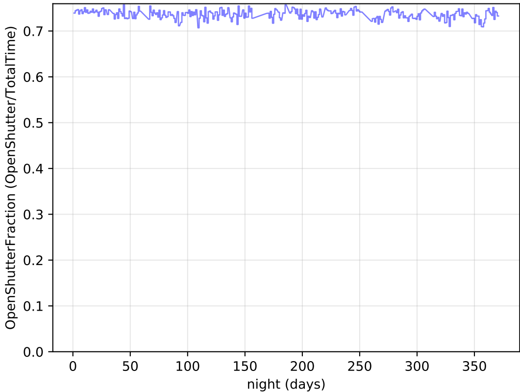
nside64 : OpenShutterFraction
