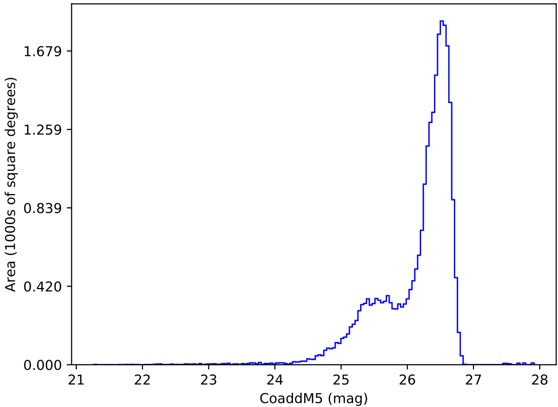
nside64 : CoaddM5
