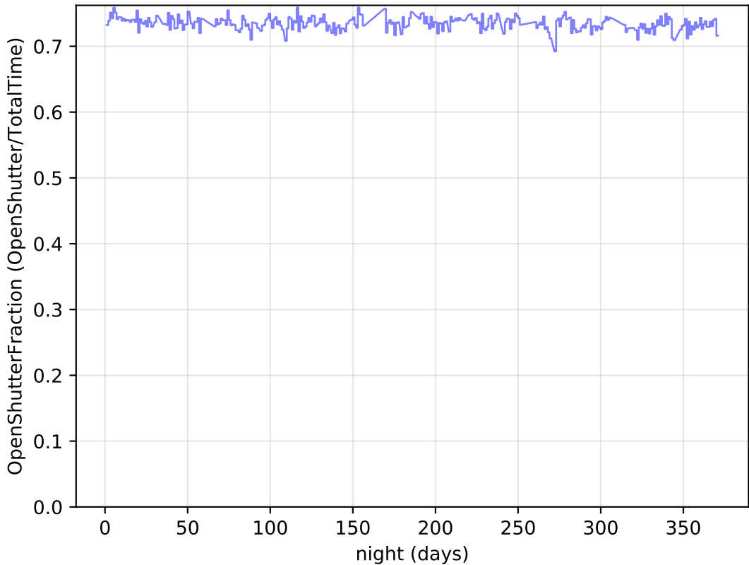
inside32 : OpenShutterFraction
