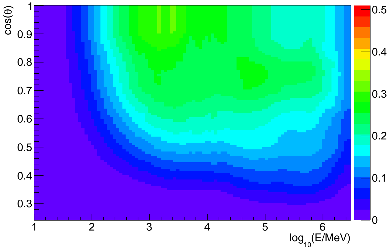
Effective area vs. energy vs. \cos(\theta) comparison for P8R2_SOURCE_V6 PSF3
