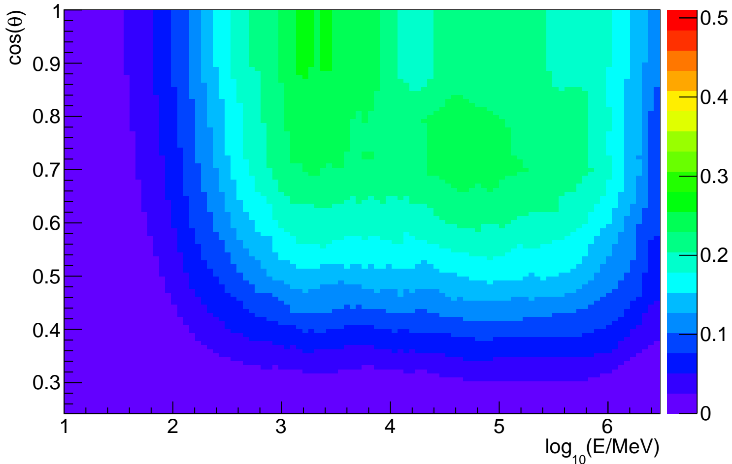
Effective area vs. energy vs. \cos(\theta) comparison for P8R2_SOURCE_V6 PSF2
