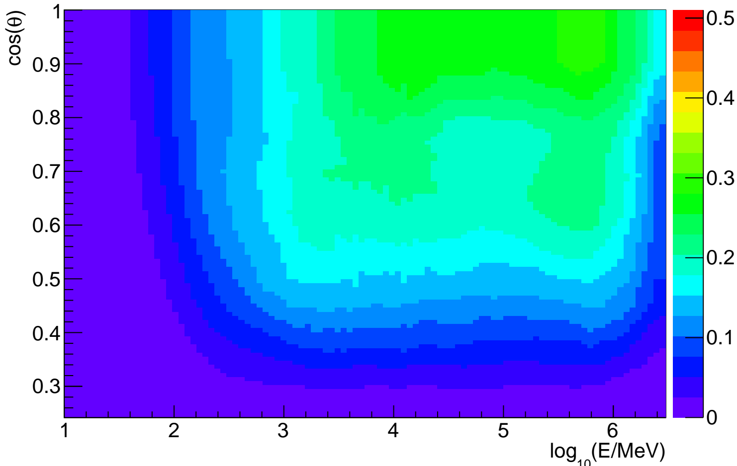
Effective area vs. energy vs. \cos(\theta) comparison for P8R2_SOURCE_V6 PSF1
