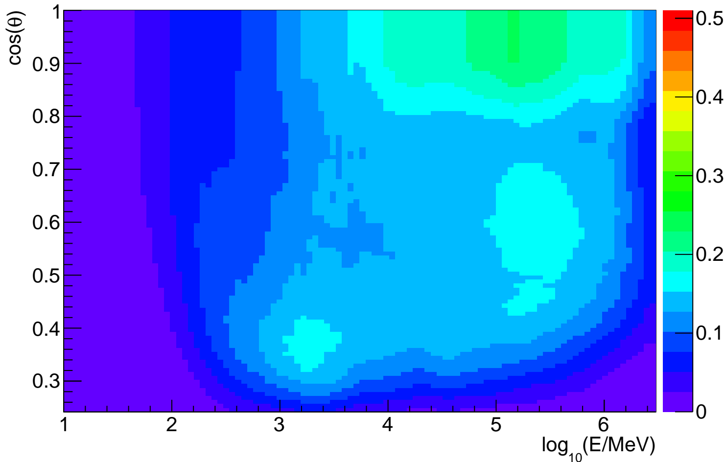
Effective area vs. energy vs. \cos(\theta) comparison for P8R2_SOURCE_V6 PSF0
