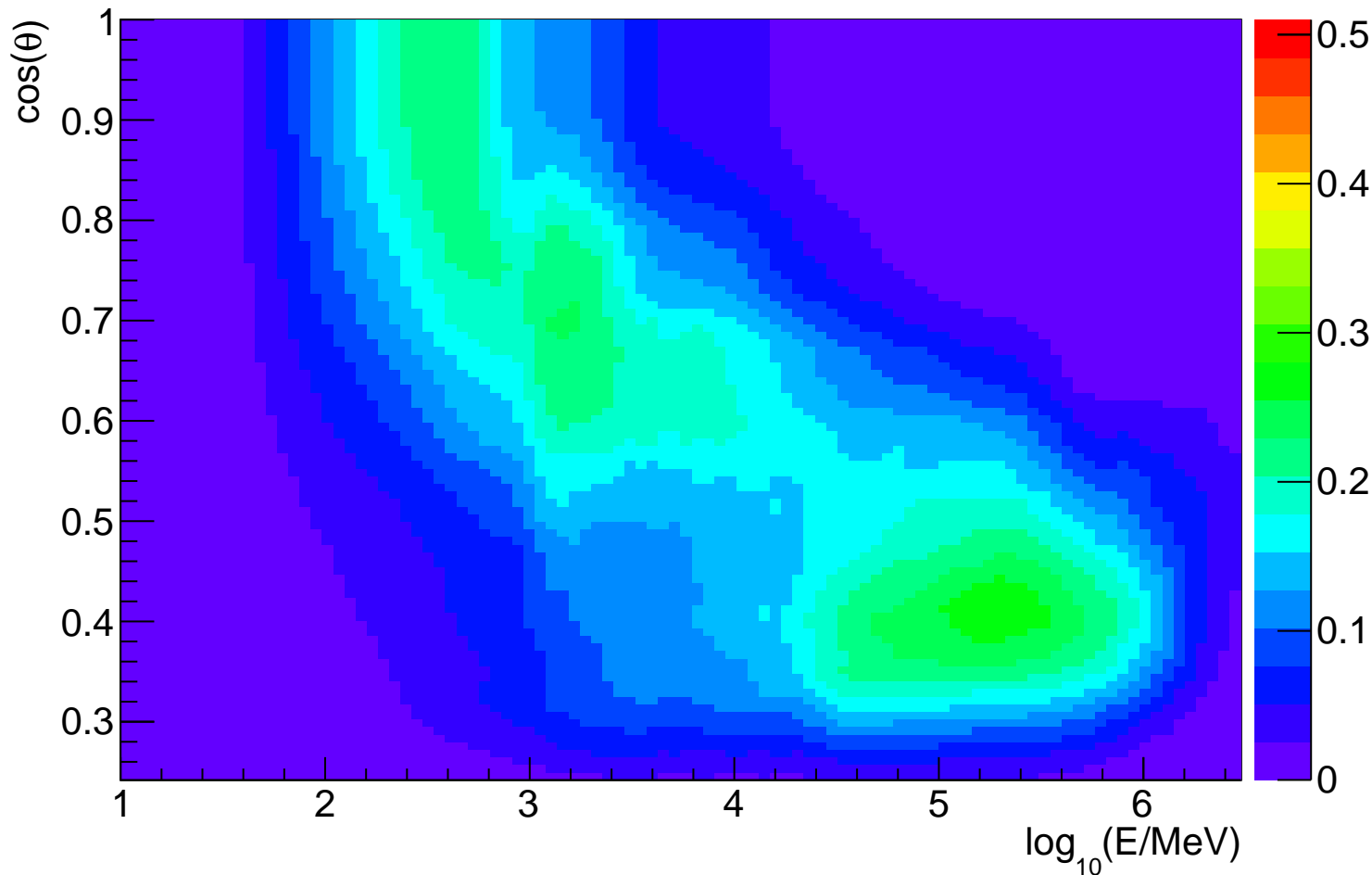
Effective area vs. energy vs. \cos(\theta) comparison for P8R2_SOURCE_V6 EDISP3
