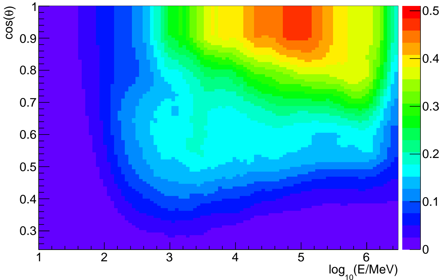
Effective area vs. energy vs. \cos(\theta) comparison for P8R2_SOURCE_V6 EDISP1
