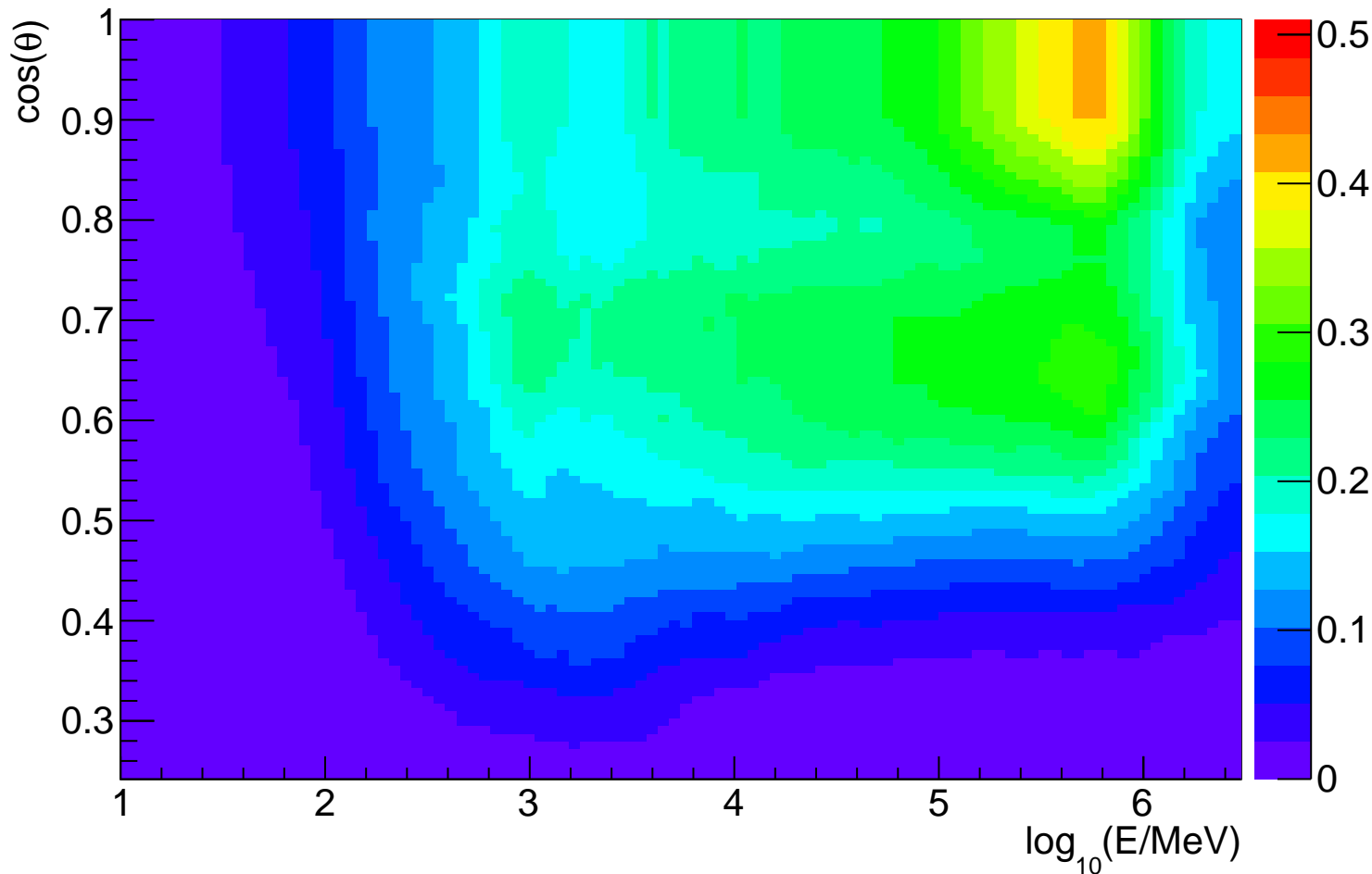
Effective area vs. energy vs. \cos(\theta) comparison for P8R2_SOURCE_V6 EDISP0
