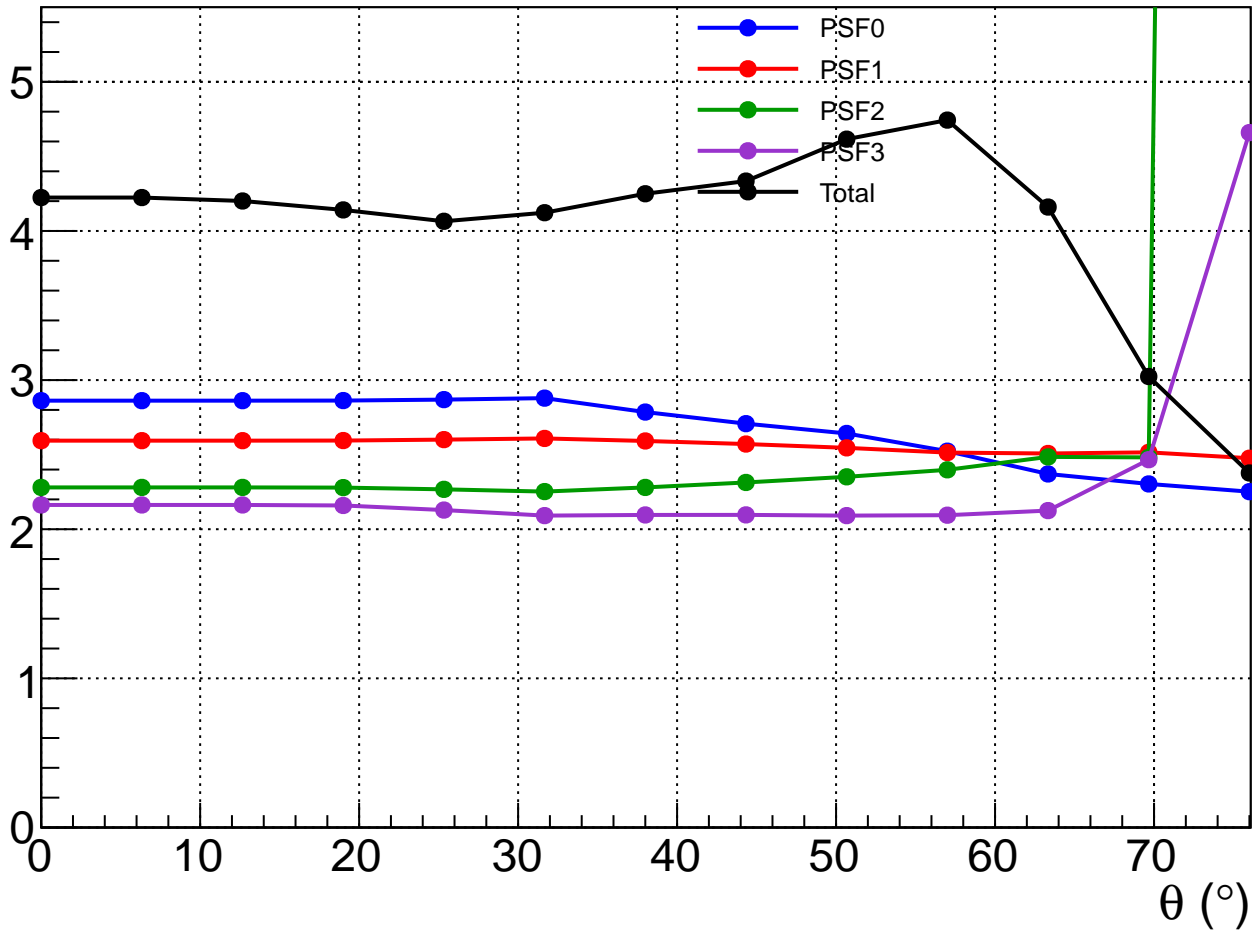
P8R2_SOURCE_V6 PSF containment ratio at 10 GeV
