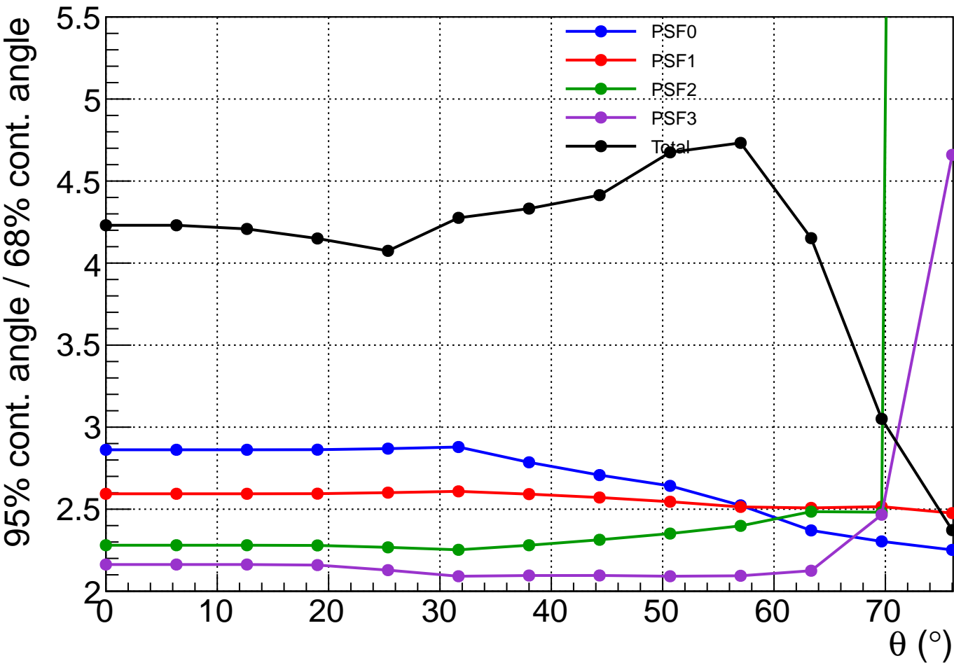
P8R2_SOURCE_V6 PSF containment ratio at 10 GeV, \phi = 0^\circ
