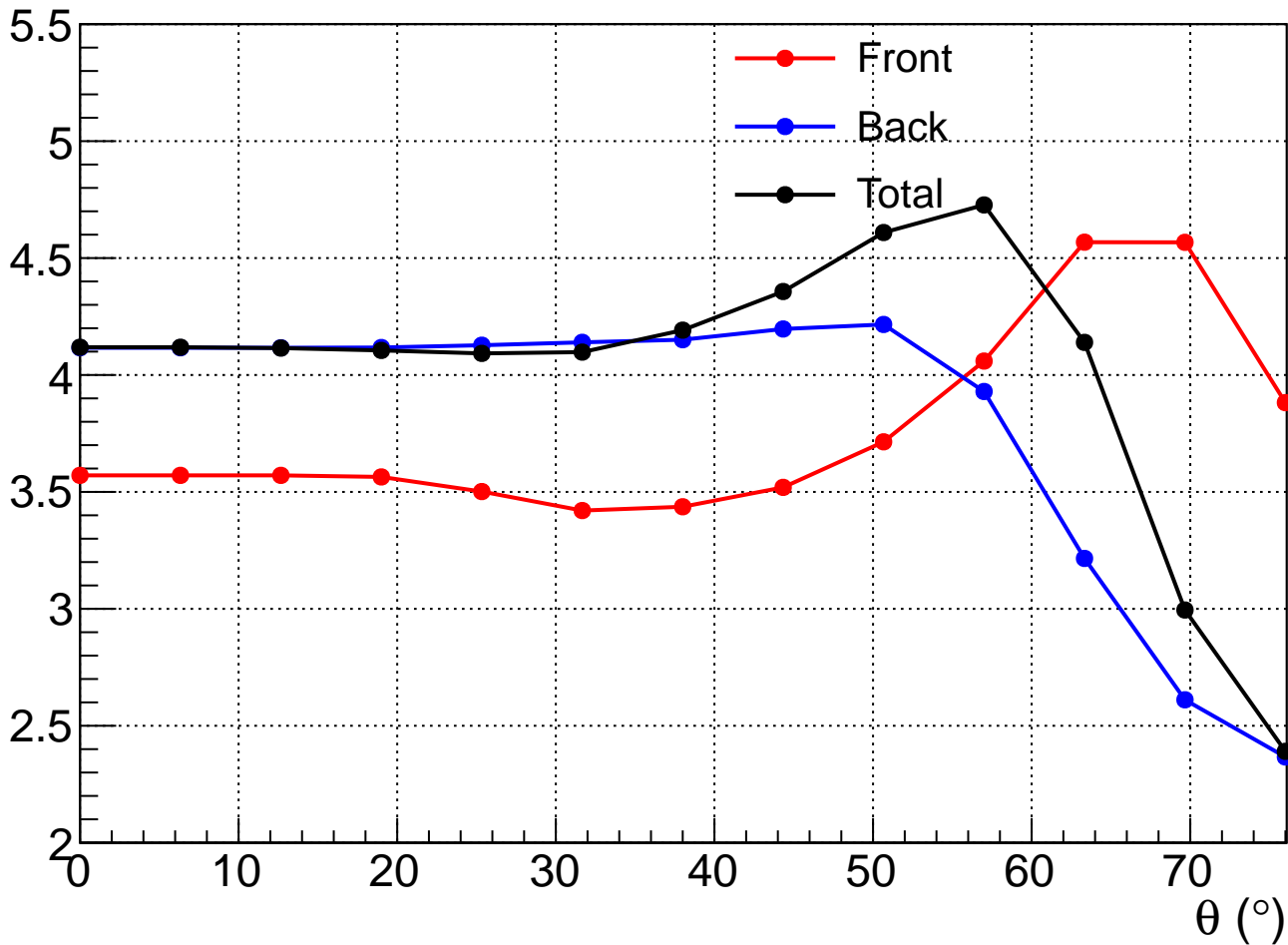
P8R2_SOURCE_V6 PSF containment ratio at 10 GeV, \phi = 0^\circ
