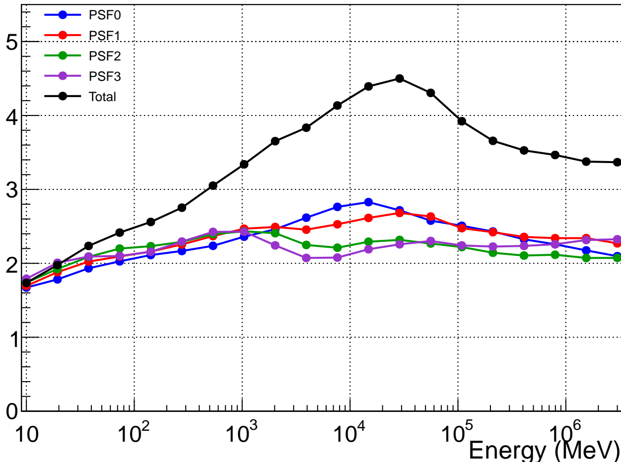
P8R2_SOURCE_V6 PSF containment ratio at normal incidence
