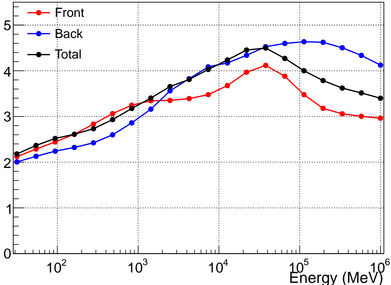
P8R2_SOURCE_V6 PSF containment ratio at normal incidence
