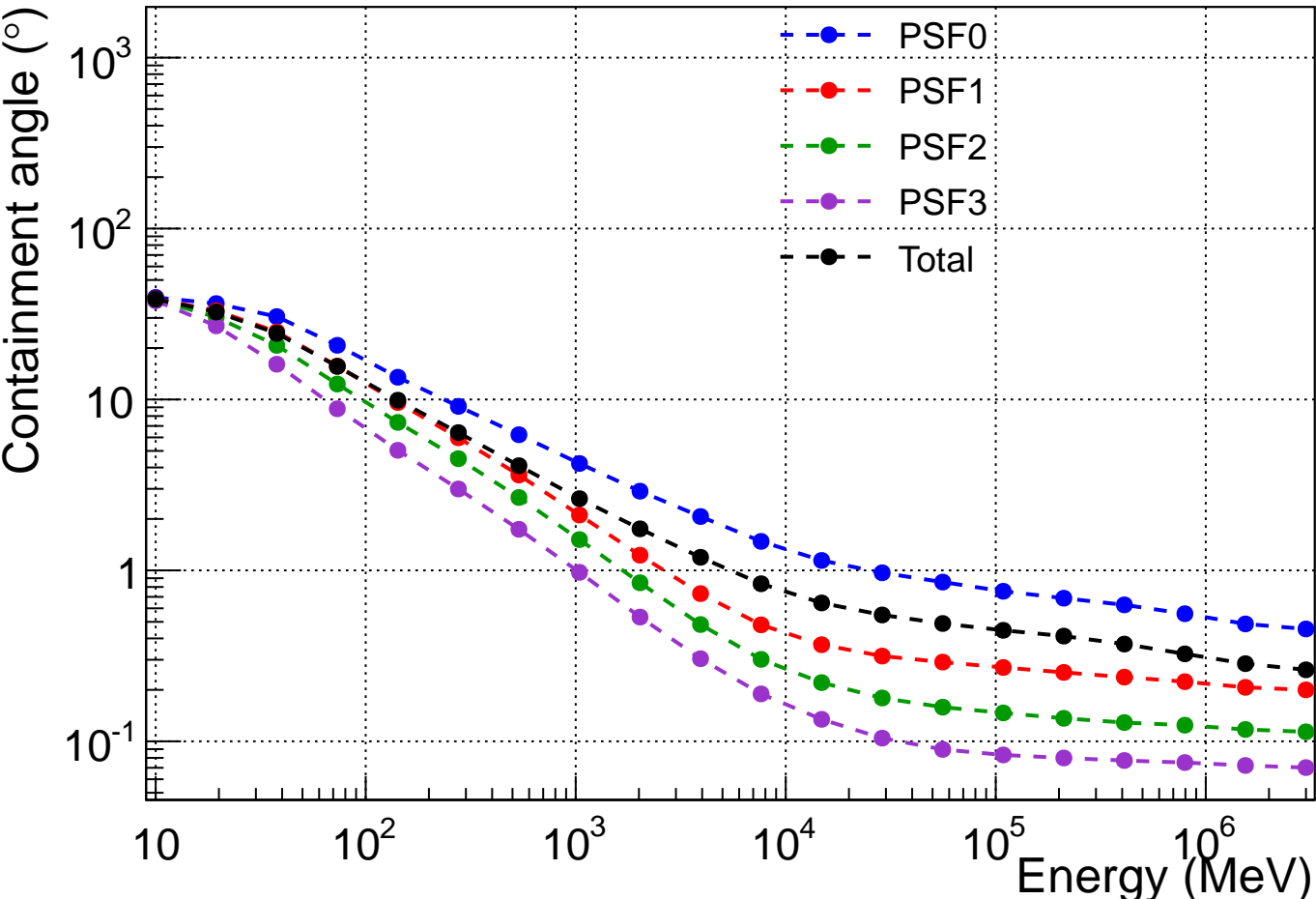
P8R2_SOURCE_V6 theta-average PSF 95% containment
