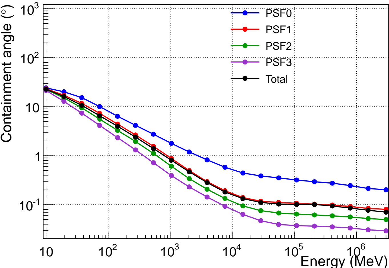
P8R2_SOURCE_V6 theta-average PSF 68% containment
