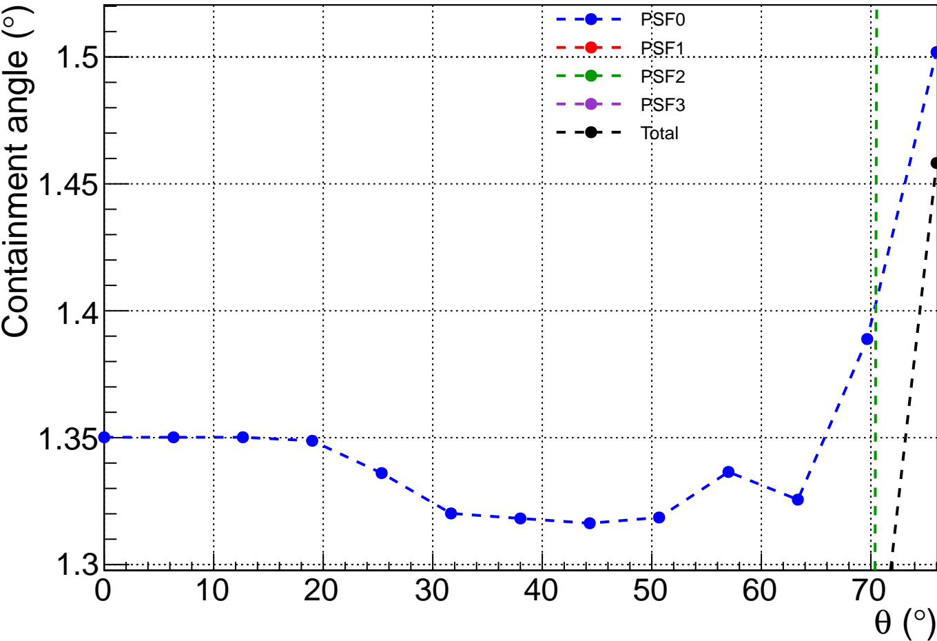
P8R2_SOURCE_V6 PSF at 10 GeV 95% containment
