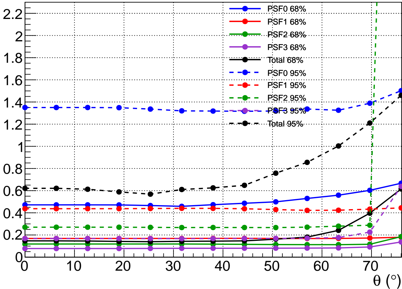
P8R2_SOURCE_V6 PSF at 10 GeV, \phi = 0^\circ
