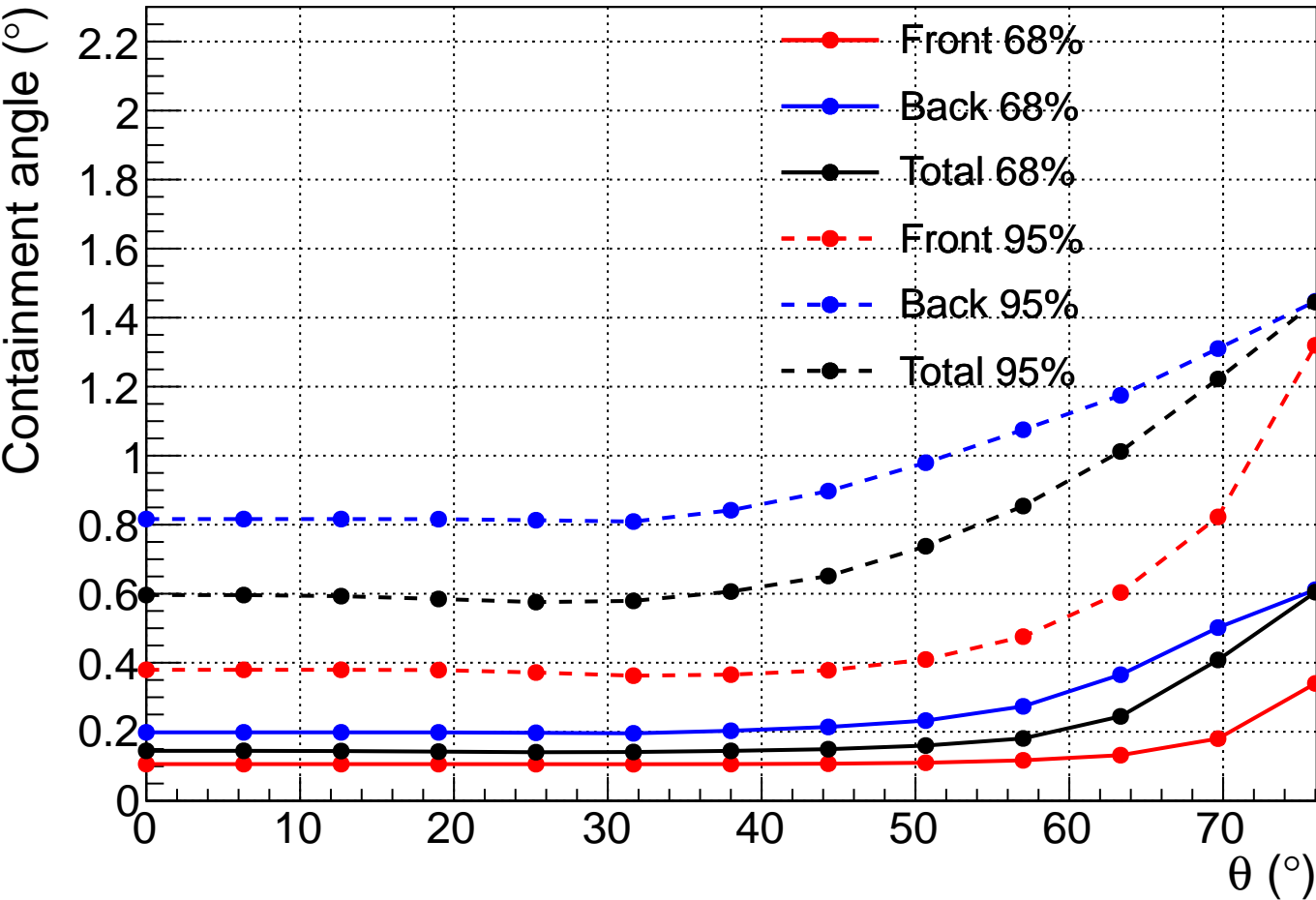
P8R2_SOURCE_V6 PSF at 10 GeV, \phi = 0^\circ
